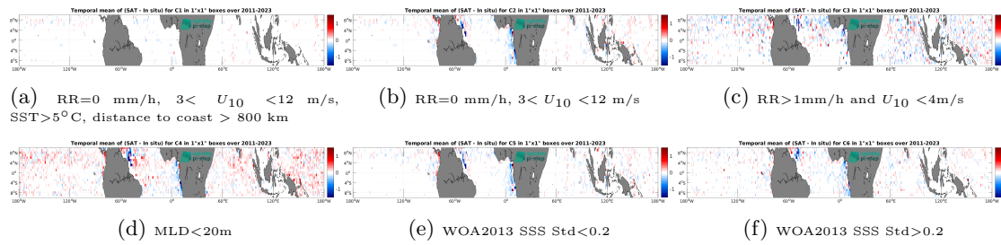
Figure 12: Temporal mean gridded over spatial boxes of size 1^\circ \times 1^\circ of \Delta SSS (SMAP SSS L4 OI v2 - 7 Days (ESR) - Argo) for 6 different subdatasets corresponding to:RR=0 mm/h, 3 < U_{10} < 12 m/s, SST >5^\circ C, distance to coast > 800 km (a), RR=0 mm/h, 3 < U_{10} < 12 m/s (b), RR >1 mm/h and U_{10} < 4 m/s (c),MLD <20 m (d),WOA2013 SSS Std <0.2 (e),WOA2013 SSS Std >0.2 (f).
