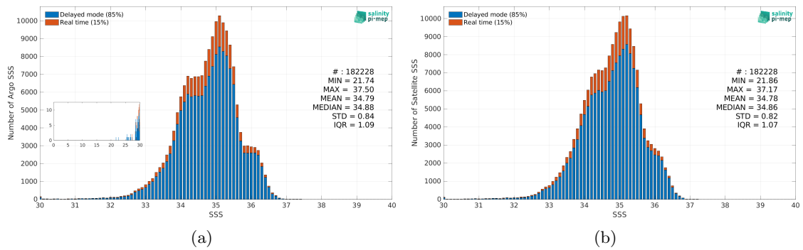
Figure 2: Histograms of SSS from Argo (a) and SMAP SSS L4 OI v2 - 7 Days (ESR) (b) considering all match-up pairs per bins of 0.1 over the Equatorial Ocean 10N-10S Pi-MEP region and for the full satellite product period.
