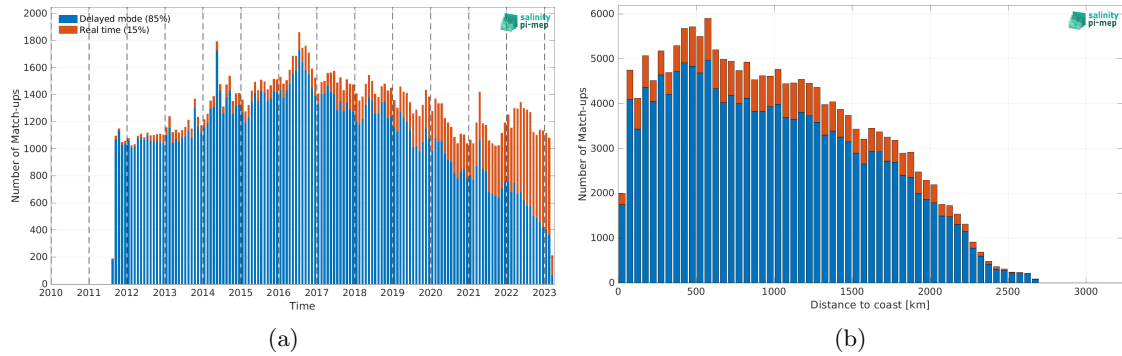
Figure 1: Number of match-ups between Argo and SMAP SSS L4 OI v2 - 7 Days (ESR) SSS as a function of time (a) and as function of the distance to coast (b) over the Equatorial Ocean 10N-10S Pi-MEP region and for the full satellite product period.
