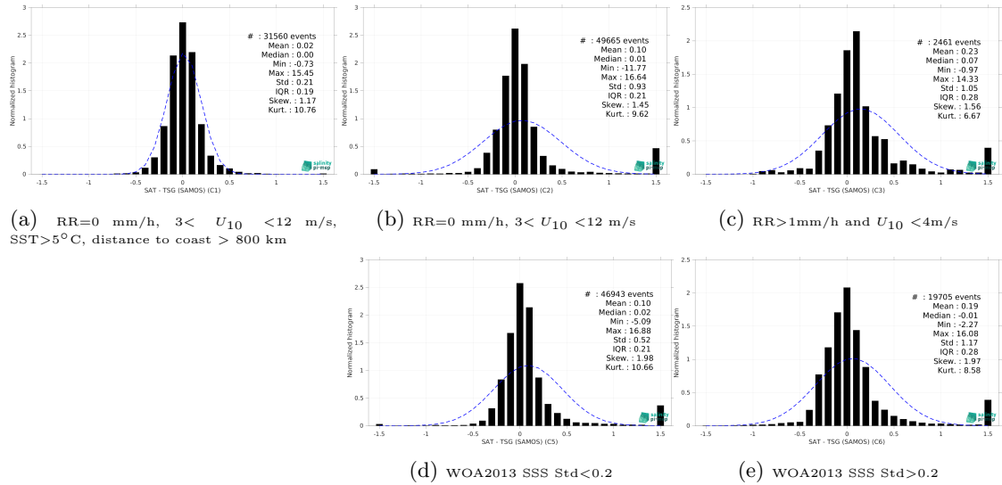
Figure 13: Normalized histogram of \Delta SSS (SMAP SSS L4 OI v2 - Monthly (IPRC) - TSG (SAMOS)) for 5 different subdatasets corresponding to: RR=0 mm/h, 3 < U_{10} < 12 m/s, SST >5^\circ C, distance to coast > 800 km (a), RR=0 mm/h, 3 < U_{10} < 12 m/s (b), RR >1 mm/h and U_{10} < 4 m/s (c), WOA2013 SSS Std <0.2 (d), WOA2013 SSS Std >0.2 (e).
