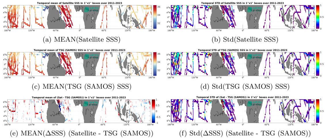
Figure 6: Temporal mean (left) and Std (right) of SSS from SMAP SSS L4 OI v2 - Monthly (IPRC) (top), TSG (SAMOS) (middle), and of \Delta SSS (Satellite - TSG (SAMOS)). Only match-up pairs are used to generate these maps.
