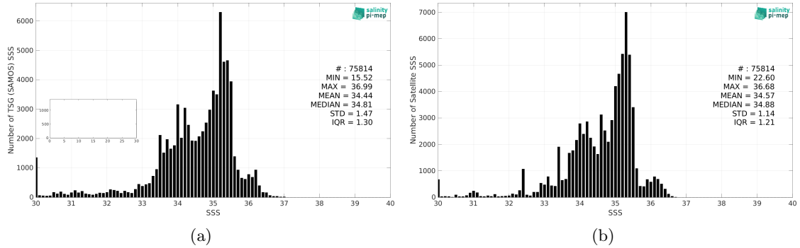
Figure 2: Histograms of SSS from TSG (SAMOS) (a) and SMAP SSS L4 OI v2 - Monthly (IPRC) (b) considering all match-up pairs per bins of 0.1 over the Equatorial Ocean 10N-10S Pi-MEP region and for the full satellite product period.
