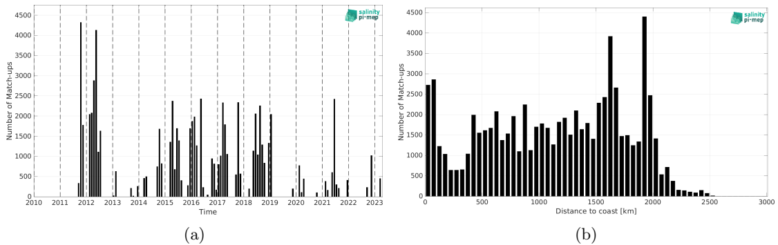
Figure 1: Number of match-ups between TSG (SAMOS) and SMAP SSS L4 OI v2 - Monthly (IPRC) SSS as a function of time (a) and as function of the distance to coast (b) over the Equatorial Ocean 10N-10S Pi-MEP region and for the full satellite product period.
