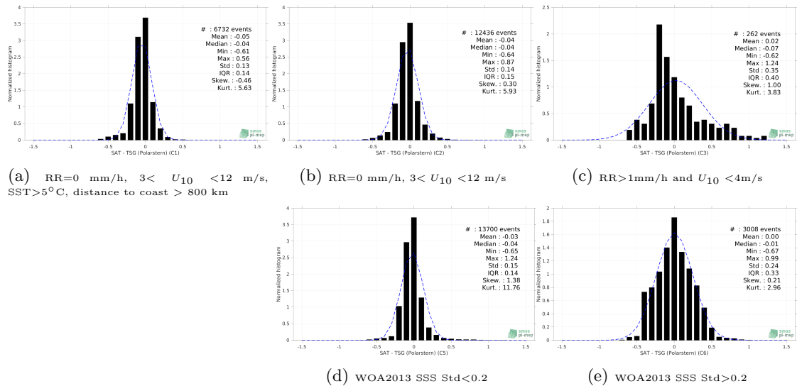
Figure 13: Normalized histogram of \Delta SSS (SMAP SSS L4 OI v2 - Monthly (IPRC) - TSG (Polarstern)) for 5 different subdatasets corresponding to: RR=0 mm/h, 3 < U_{10} < 12 m/s, SST >5^\circ\text{C} , distance to coast > 800 km (a), RR=0 mm/h, 3 < U_{10} < 12 m/s (b), RR >1 mm/h and U_{10} < 4 m/s (c), WOA2013 SSS Std <0.2 (d), WOA2013 SSS Std >0.2 (e).
