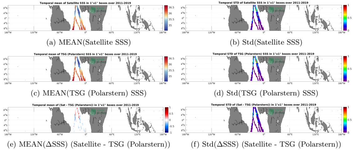
Figure 6: Temporal mean (left) and Std (right) of SSS from SMAP SSS L4 OI v2 - Monthly (IPRC) (top), TSG (Polarstern) (middle), and of \Delta SSS (Satellite - TSG (Polarstern)). Only match-up pairs are used to generate these maps.
