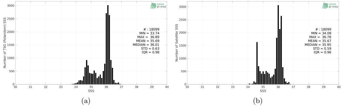
Figure 2: Histograms of SSS from TSG (Polarstern) (a) and SMAP SSS L4 OI v2 - Monthly (IPRC) (b) considering all match-up pairs per bins of 0.1 over the Equatorial Ocean 10N-10S Pi-MEP region and for the full satellite product period.
