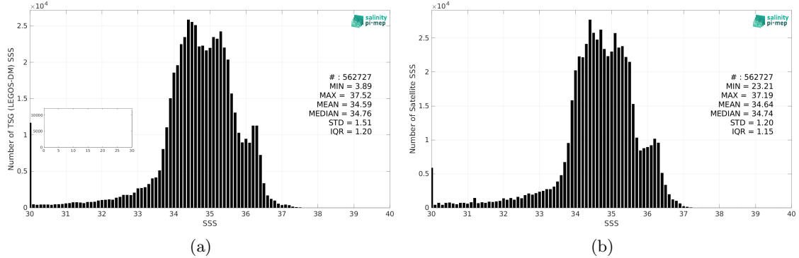
Figure 2: Histograms of SSS from TSG (LEGOS-DM) (a) and SMAP SSS L4 OI v2 - Monthly (IPRC) (b) considering all match-up pairs per bins of 0.1 over the Equatorial Ocean 10N-10S Pi-MEP region and for the full satellite product period.
