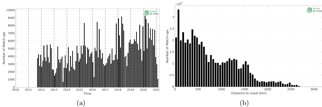
Figure 1: Number of match-ups between TSG (LEGOS-DM) and SMAP SSS L4 OI v2 - Monthly (IPRC) SSS as a function of time (a) and as function of the distance to coast (b) over the Equatorial Ocean 10N-10S Pi-MEP region and for the full satellite product period.
