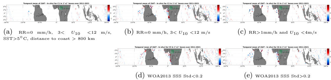
Figure 12: Temporal mean gridded over spatial boxes of size 1^\circ \times 1^\circ of \Delta SSS (SMAP SSS L4 OI v2 - Monthly (IPRC) - TSG (LEGOS-DM)) for 5 different subdatasets corresponding to: RR=0 mm/h, 3 < U_{10} < 12 m/s, SST >5^\circ\text{C} , distance to coast > 800 km (a), RR=0 mm/h, 3 < U_{10} < 12 m/s (b), RR >1 mm/h and U_{10} < 4 m/s (c), WOA2013 SSS Std <0.2 (d), WOA2013 SSS Std >0.2 (e).
