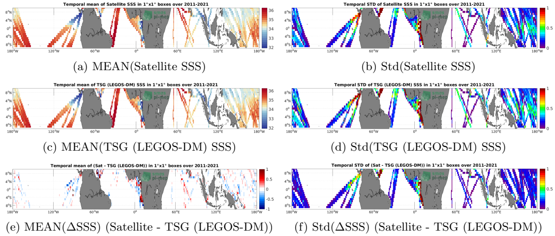
Figure 6: Temporal mean (left) and Std (right) of SSS from SMAP SSS L4 OI v2 - Monthly (IPRC) (top), TSG (LEGOS-DM) (middle), and of \Delta SSS (Satellite - TSG (LEGOS-DM)). Only match-up pairs are used to generate these maps.
