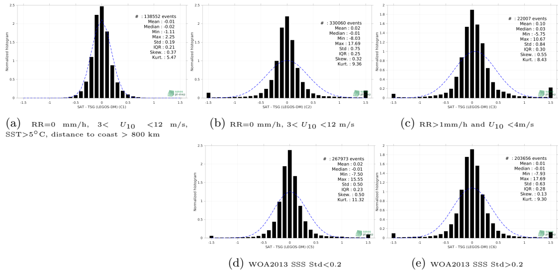
Figure 13: Normalized histogram of \Delta SSS (SMAP SSS L4 OI v2 - Monthly (IPRC) - TSG (LEGOS-DM)) for 5 different subdatasets corresponding to: RR=0 mm/h, 3 < U_{10} < 12 m/s, SST >5^\circ\text{C} , distance to coast > 800 km (a), RR=0 mm/h, 3 < U_{10} < 12 m/s (b), RR >1 mm/h and U_{10} < 4 m/s (c), WOA2013 SSS Std <0.2 (d), WOA2013 SSS Std >0.2 (e).
