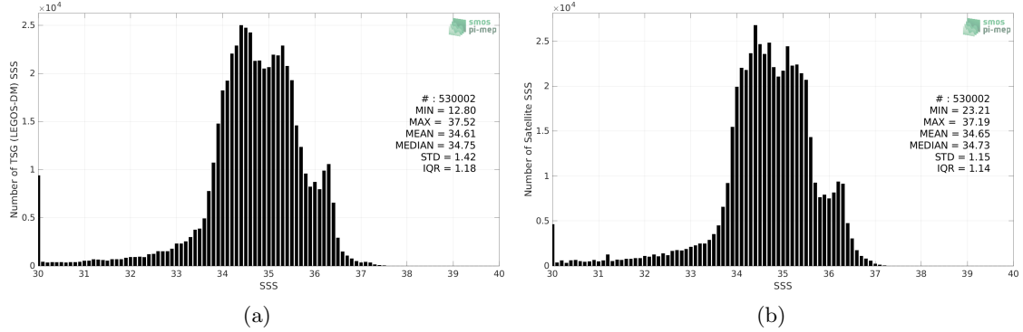
Figure 2: Histograms of SSS from TSG (LEGOS-DM) (a) and SMAP SSS L4 OI v2 - Monthly (IPRC) (b) considering all match-up pairs per bins of 0.1 over the Equatorial Ocean 10N-10S Pi-MEP region and for the full satellite product period.
