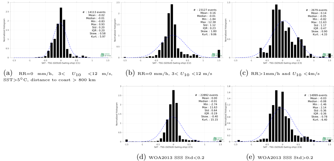
Figure 13: Normalized histogram of \Delta SSS (SMAP SSS L4 OI v2 - Monthly (IPRC) - TSG (GOSUD-Sailing-ship)) for 5 different subdatasets corresponding to: RR=0 mm/h, 3 < U_{10} < 12 m/s, SST >5^\circ C, distance to coast > 800 km (a), RR=0 mm/h, 3 < U_{10} < 12 m/s (b), RR >1 mm/h and U_{10} < 4 m/s (c), WOA2013 SSS Std <0.2 (d), WOA2013 SSS Std >0.2 (e).
