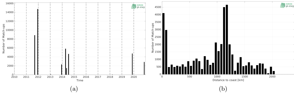
Figure 1: Number of match-ups between TSG (GOSUD-Sailing-ship) and SMAP SSS L4 OI v2 - Monthly (IPRC) SSS as a function of time (a) and as function of the distance to coast (b) over the Equatorial Ocean 10N-10S Pi-MEP region and for the full satellite product period.
