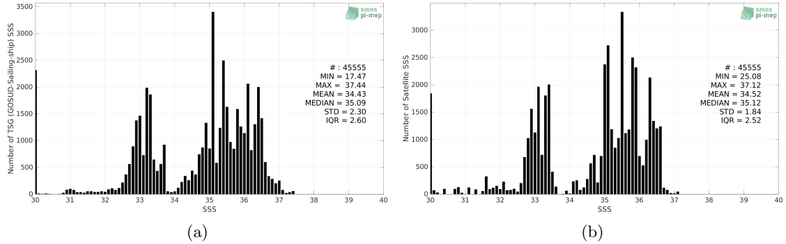
Figure 2: Histograms of SSS from TSG (GOSUD-Sailing-ship) (a) and SMAP SSS L4 OI v2 - Monthly (IPRC) (b) considering all match-up pairs per bins of 0.1 over the Equatorial Ocean 10N-10S Pi-MEP region and for the full satellite product period.
