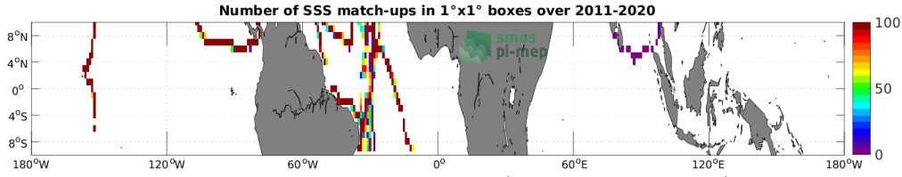
Figure 4: Number of SSS match-ups between TSG (GOSUD-Sailing-ship) SSS and the SMAP SSS L4 OI v2 - Monthly (IPRC) SSS product for the Equatorial Ocean 10N-10S Pi-MEP region over 1^\circ \times 1^\circ boxes and for the full satellite product period.
