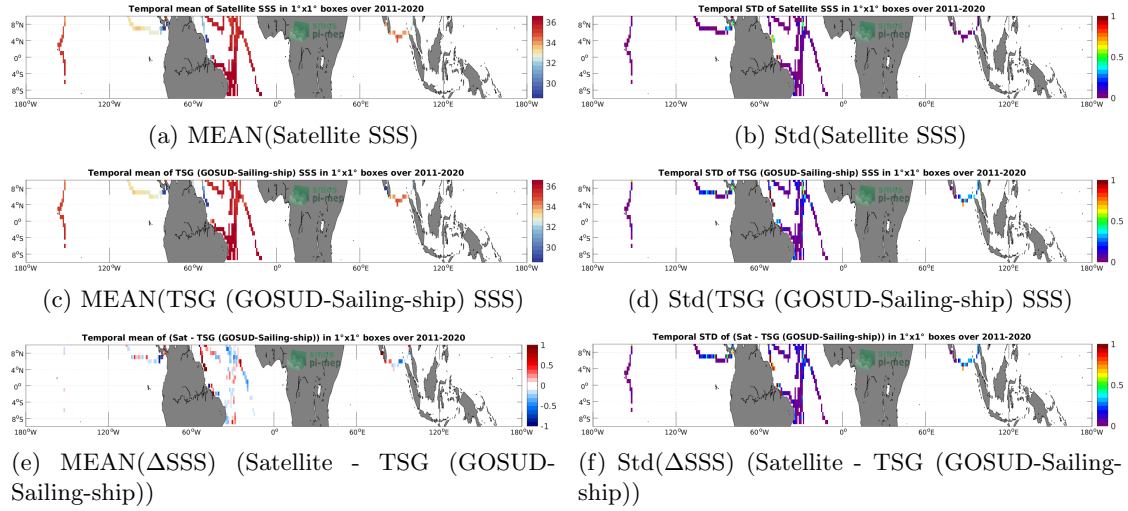
Figure 6: Temporal mean (left) and Std (right) of SSS from SMAP SSS L4 OI v2 - Monthly (IPRC) (top), TSG (GOSUD-Sailing-ship) (middle), and of \Delta SSS (Satellite - TSG (GOSUD-Sailing-ship)). Only match-up pairs are used to generate these maps.
