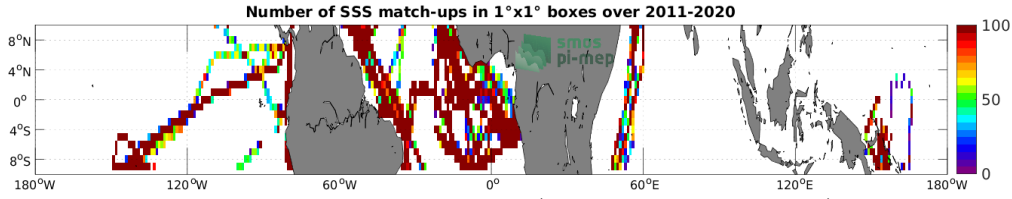
Figure 4: Number of SSS match-ups between TSG (GOSUD-Research-vessel) SSS and the SMAP SSS L4 OI v2 - Monthly (IPRC) SSS product for the Equatorial Ocean 10N-10S Pi-MEP region over 1^\circ \times 1^\circ boxes and for the full satellite product period.
