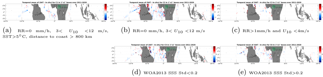
Figure 12: Temporal mean gridded over spatial boxes of size 1^\circ \times 1^\circ of \Delta SSS (SMAP SSS L4 OI v2 - Monthly (IPRC) - TSG (GOSUD-Research-vessel)) for 5 different subdatasets corresponding to: RR=0 mm/h, 3 < U_{10} < 12 m/s, SST>5°C, distance to coast > 800 km (a), RR=0 mm/h, 3 < U_{10} < 12 m/s (b), RR>1mm/h and U_{10} < 4 m/s (c), WOA2013 SSS Std<0.2 (d), WOA2013 SSS Std>0.2 (e).
