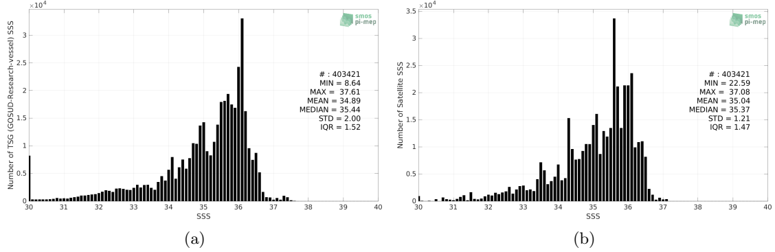
Figure 2: Histograms of SSS from TSG (GOSUD-Research-vessel) (a) and SMAP SSS L4 OI v2 - Monthly (IPRC) (b) considering all match-up pairs per bins of 0.1 over the Equatorial Ocean 10N-10S Pi-MEP region and for the full satellite product period.
