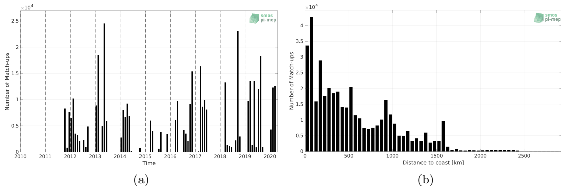
Figure 1: Number of match-ups between TSG (GOSUD-Research-vessel) and SMAP SSS L4 OI v2 - Monthly (IPRC) SSS as a function of time (a) and as function of the distance to coast (b) over the Equatorial Ocean 10N-10S Pi-MEP region and for the full satellite product period.
