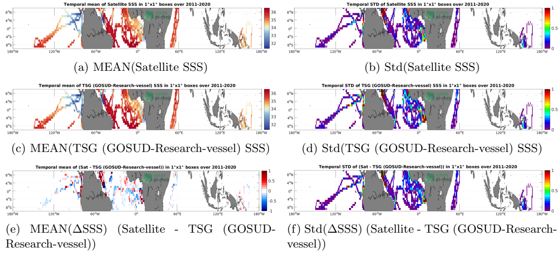
Figure 6: Temporal mean (left) and Std (right) of SSS from SMAP SSS L4 OI v2 - Monthly (IPRC) (top), TSG (GOSUD-Research-vessel) (middle), and of \Delta SSS (Satellite - TSG (GOSUD-Research-vessel)). Only match-up pairs are used to generate these maps.
