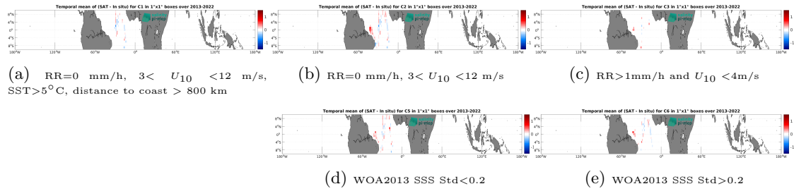
Figure 12: Temporal mean gridded over spatial boxes of size 1^\circ \times 1^\circ of \Delta SSS (SMAP SSS L4 OI v2 - Monthly (IPRC) - TSG (CSIC-UTM)) for 5 different subdatasets corresponding to:RR=0 mm/h, 3 < U_{10} < 12 m/s, SST >5^\circ C, distance to coast > 800 km (a), RR=0 mm/h, 3 < U_{10} < 12 m/s (b), RR >1 mm/h and U_{10} < 4 m/s (c), WOA2013 SSS Std <0.2 (d), WOA2013 SSS Std >0.2 (e).
