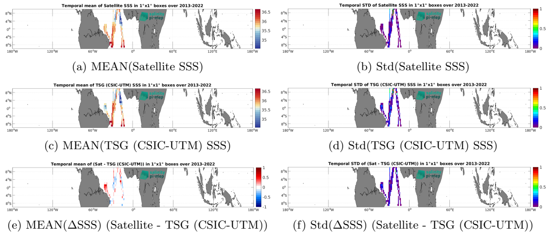
Figure 6: Temporal mean (left) and Std (right) of SSS from SMAP SSS L4 OI v2 - Monthly (IPRC) (top), TSG (CSIC-UTM) (middle), and of \Delta SSS (Satellite - TSG (CSIC-UTM)). Only match-up pairs are used to generate these maps.
