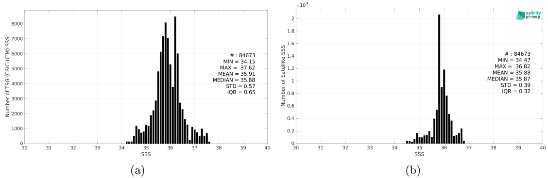
Figure 2: Histograms of SSS from TSG (CSIC-UTM) (a) and SMAP SSS L4 OI v2 - Monthly (IPRC) (b) considering all match-up pairs per bins of 0.1 over the Equatorial Ocean 10N-10S Pi-MEP region and for the full satellite product period.
