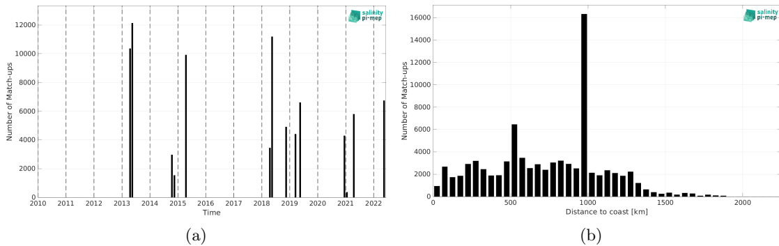
Figure 1: Number of match-ups between TSG (CSIC-UTM) and SMAP SSS L4 OI v2 - Monthly (IPRC) SSS as a function of time (a) and as function of the distance to coast (b) over the Equatorial Ocean 10N-10S Pi-MEP region and for the full satellite product period.
