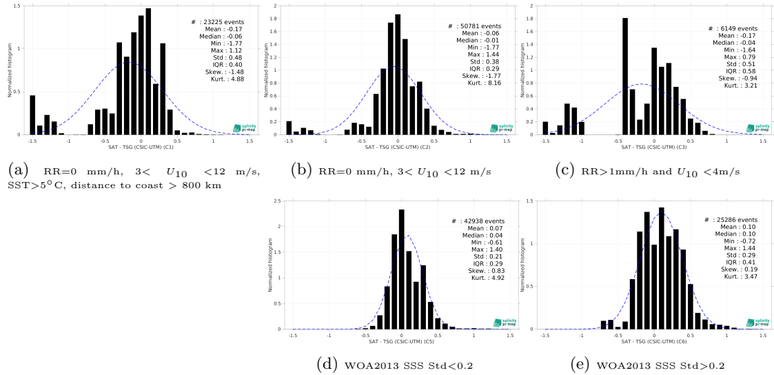
Figure 13: Normalized histogram of \Delta SSS (SMAP SSS L4 OI v2 - Monthly (IPRC) - TSG (CSIC-UTM)) for 5 different subdatasets corresponding to: RR=0 mm/h, 3 < U_{10} < 12 m/s, SST >5^\circ C, distance to coast > 800 km (a), RR=0 mm/h, 3 < U_{10} < 12 m/s (b), RR >1 mm/h and U_{10} < 4 m/s (c), WOA2013 SSS Std <0.2 (d), WOA2013 SSS Std >0.2 (e).
