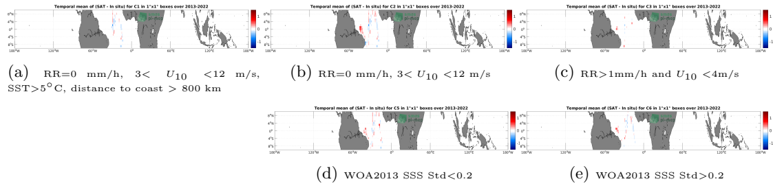
Figure 12: Temporal mean gridded over spatial boxes of size 1^\circ \times 1^\circ of \Delta SSS (SMAP SSS L4 OI v2 - Monthly (IPRC) - TSG (CSIC-UTM)) for 5 different subdatasets corresponding to: RR=0 mm/h, 3 < U_{10} < 12 m/s, SST>5°C, distance to coast > 800 km (a), RR=0 mm/h, 3 < U_{10} < 12 m/s (b), RR>1mm/h and U_{10} < 4 m/s (c), WOA2013 SSS Std<0.2 (d), WOA2013 SSS Std>0.2 (e).
