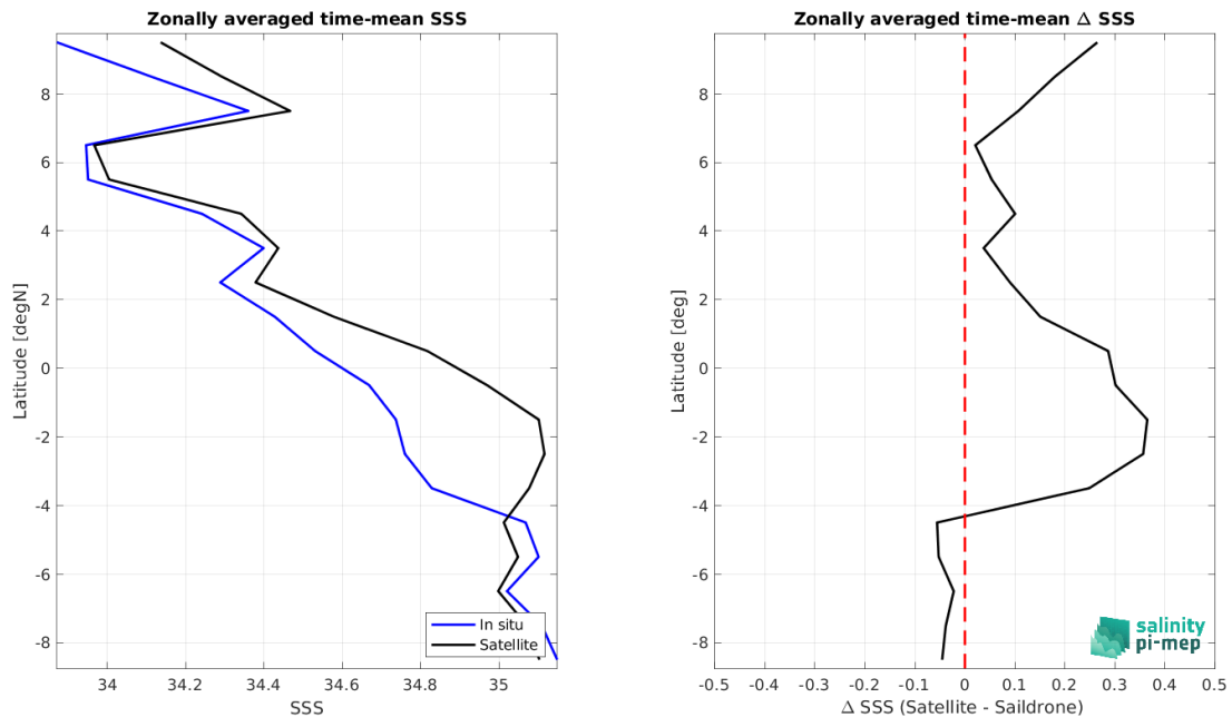
Figure 8: Left panel: Zonal mean SSS from SMAP SSS L4 OI v2 - Monthly (IPRC) satellite product (black) and from Sairdrone (blue). Right panel: Zonal mean of \Delta SSS (Satellite - Sairdrone) for all the collected Pi-MEP match-up pairs estimated over the full satellite product period.
