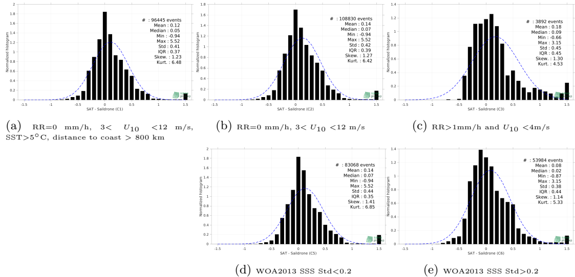
Figure 13: Normalized histogram of \Delta SSS (SMAP SSS L4 OI v2 - Monthly (IPRC) - Sailldrone) for 5 different subdatasets corresponding to: RR=0 mm/h, 3 < U_{10} < 12 m/s, SST>5°C, distance to coast > 800 km (a), RR=0 mm/h, 3 < U_{10} < 12 m/s (b), RR>1mm/h and U_{10} < 4 m/s (c), WOA2013 SSS Std<0.2 (d), WOA2013 SSS Std>0.2 (e).
