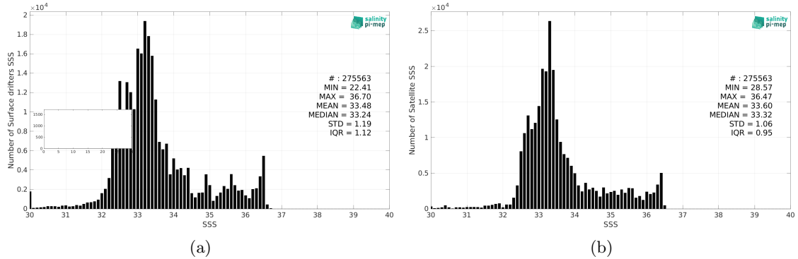
Figure 2: Histograms of SSS from Surface drifters (a) and SMAP SSS L4 OI v2 - Monthly (IPRC) (b) considering all match-up pairs per bins of 0.1 over the Equatorial Ocean 10N-10S Pi-MEP region and for the full satellite product period.
