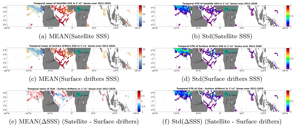
Figure 5: Temporal mean (left) and Std (right) of SSS from SMAP SSS L4 OI v2 - Monthly (IPRC) (top), Surface drifters (middle), and of \Delta SSS (Satellite - Surface drifters). Only match-up pairs are used to generate these maps.
