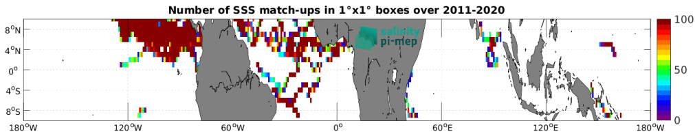
Figure 3: Number of SSS match-ups between Surface drifters SSS and the SMAP SSS L4 OI v2 - Monthly (IPRC) SSS product for the Equatorial Ocean 10N-10S Pi-MEP region over 1^\circ \times 1^\circ boxes and for the full satellite product period.
