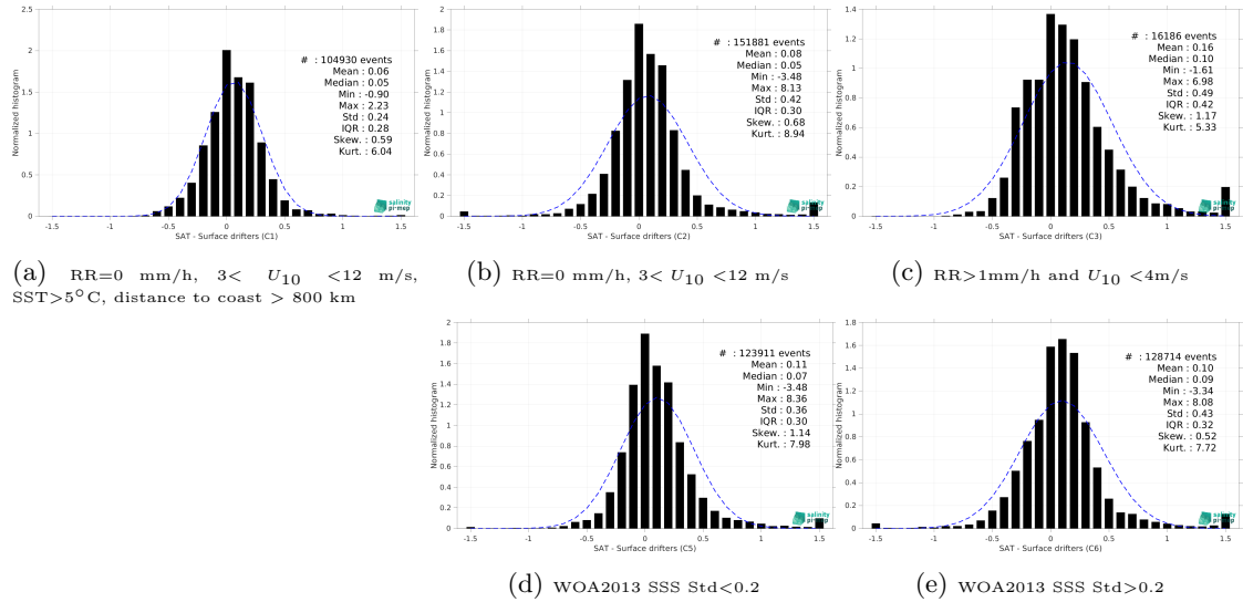
Figure 12: Normalized histogram of \Delta SSS (SMAP SSS L4 OI v2 - Monthly (IPRC) - Surface drifters) for 5 different subdatasets corresponding to: RR=0 mm/h, 3 < U_{10} < 12 m/s, SST >5^\circ C, distance to coast > 800 km (a), RR=0 mm/h, 3 < U_{10} < 12 m/s (b), RR >1 mm/h and U_{10} < 4 m/s (c), WOA2013 SSS Std <0.2 (d), WOA2013 SSS Std >0.2 (e).
