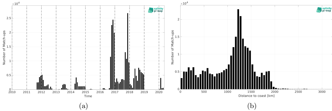
Figure 1: Number of match-ups between Surface drifters and SMAP SSS L4 OI v2 - Monthly (IPRC) SSS as a function of time (a) and as function of the distance to coast (b) over the Equatorial Ocean 10N-10S Pi-MEP region and for the full satellite product period.
