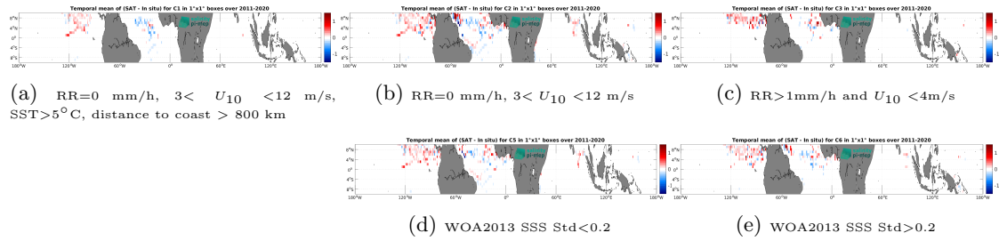
Figure 11: Temporal mean gridded over spatial boxes of size 1^\circ \times 1^\circ of \Delta SSS (SMAP SSS L4 OI v2 - Monthly (IPRC) - Surface drifters) for 5 different subdatasets corresponding to: RR=0 mm/h, 3 < U_{10} < 12 m/s, SST >5^\circ C, distance to coast > 800 km (a), RR=0 mm/h, 3 < U_{10} < 12 m/s (b), RR >1 mm/h and U_{10} < 4 m/s (c), WOA2013 SSS Std <0.2 (d), WOA2013 SSS Std >0.2 (e).
