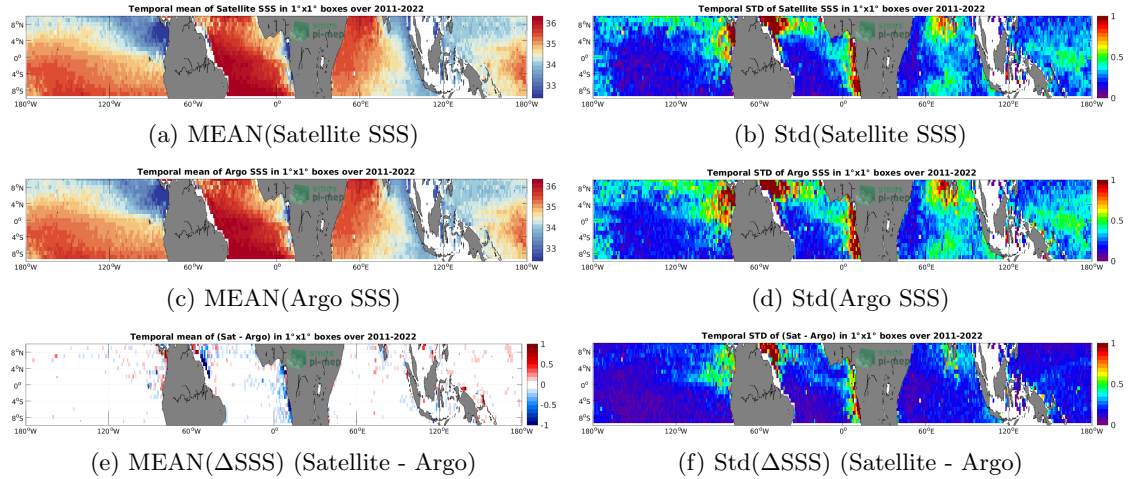
Figure 6: Temporal mean (left) and Std (right) of SSS from SMAP SSS L4 OI v2 - Monthly (IPRC) (top), Argo (middle), and of \Delta SSS (Satellite - Argo). Only match-up pairs are used to generate these maps.
