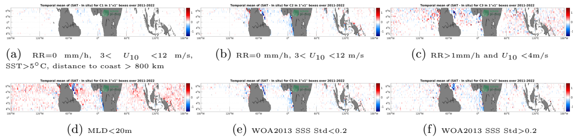
Figure 12: Temporal mean gridded over spatial boxes of size 1^\circ \times 1^\circ of \Delta SSS (SMAP SSS L4 OI v2 - Monthly (IPRC) - Argo) for 6 different subdatasets corresponding to:RR=0 mm/h, 3 < U_{10} < 12 m/s, SST >5^\circ C, distance to coast > 800 km (a), RR=0 mm/h, 3 < U_{10} < 12 m/s (b), RR >1 mm/h and U_{10} < 4 m/s (c),MLD <20 m (d),WOA2013 SSS Std <0.2 (e),WOA2013 SSS Std >0.2 (f).
