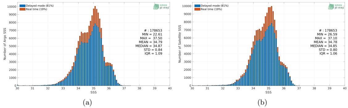
Figure 2: Histograms of SSS from Argo (a) and SMAP SSS L4 OI v2 - Monthly (IPRC) (b) considering all match-up pairs per bins of 0.1 over the Equatorial Ocean 10N-10S Pi-MEP region and for the full satellite product period.
