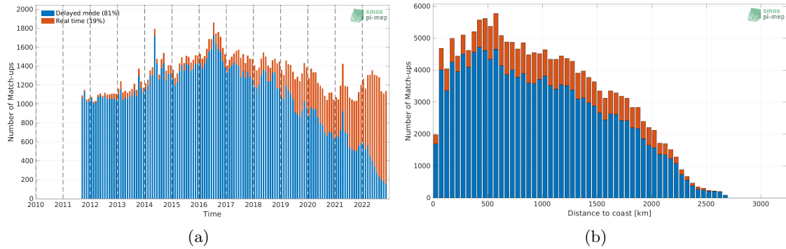
Figure 1: Number of match-ups between Argo and SMAP SSS L4 OI v2 - Monthly (IPRC) SSS as a function of time (a) and as function of the distance to coast (b) over the Equatorial Ocean 10N-10S Pi-MEP region and for the full satellite product period.
