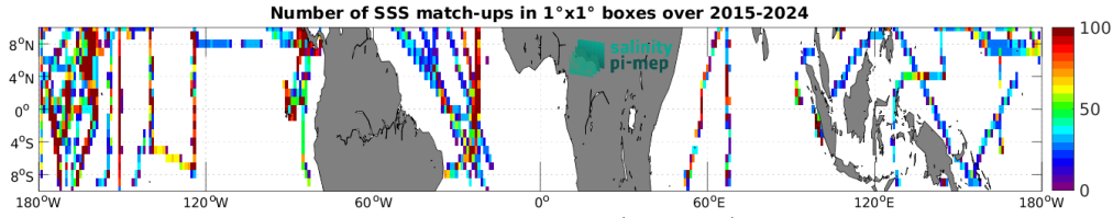
Figure 5: Number of SSS match-ups between TSG (SAMOS) SSS and the SMAP SSS L3 v6 - 8-Day running (RSS) SSS product for the Equatorial Ocean 10N-10S Pi-MEP region over 1^\circ \times 1^\circ boxes and for the full satellite product period.
