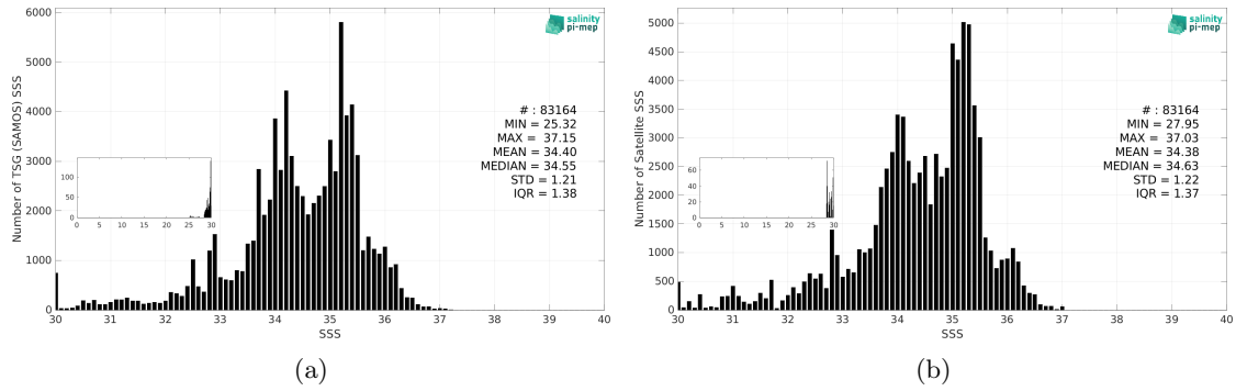
Figure 3: Histograms of SSS from TSG (SAMOS) (a) and SMAP SSS L3 v6 - 8-Day running (RSS) (b) considering all match-up pairs per bins of 0.1 over the Equatorial Ocean 10N-10S Pi-MEP region and for the full satellite product period.
