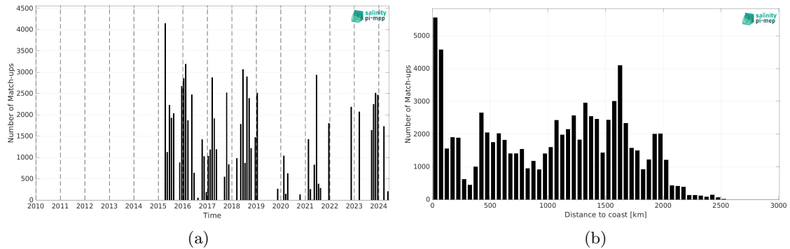
Figure 2: Number of match-ups between TSG (SAMOS) and SMAP SSS L3 v6 - 8-Day running (RSS) SSS as a function of time (a) and as function of the distance to coast (b) over the Equatorial Ocean 10N-10S Pi-MEP region and for the full satellite product period.
