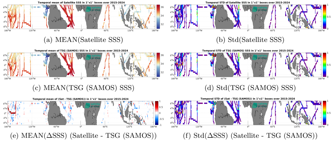
Figure 7: Temporal mean (left) and Std (right) of SSS from SMAP SSS L3 v6 - 8-Day running (RSS) (top), TSG (SAMOS) (middle), and of \Delta SSS (Satellite - TSG (SAMOS)). Only match-up pairs are used to generate these maps.
