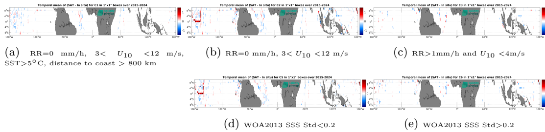
Figure 14: Temporal mean gridded over spatial boxes of size 1^\circ \times 1^\circ of \Delta SSS (SMAP SSS L3 v6 - 8-Day running (RSS) - TSG (SAMOS)) for 5 different subdatasets corresponding to:RR=0 mm/h, 3 < U_{10} < 12 m/s, SST>5°C, distance to coast > 800 km (a), RR=0 mm/h, 3 < U_{10} < 12 m/s (b), RR>1mm/h and U_{10} < 4 m/s (c), WOA2013 SSS Std<0.2 (d), WOA2013 SSS Std>0.2 (e).
