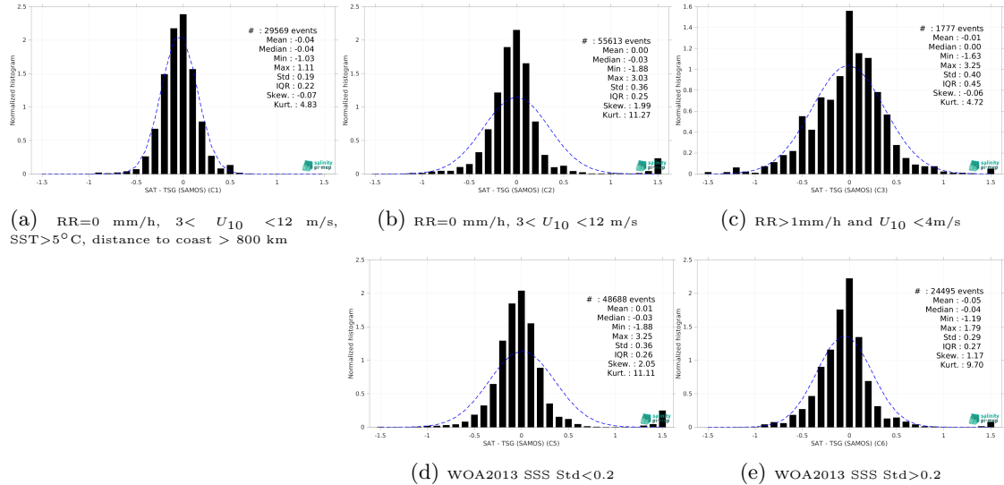
Figure 15: Normalized histogram of \Delta SSS (SMAP SSS L3 v6 - 8-Day running (RSS) - TSG (SAMOS)) for 5 different subdatasets corresponding to: RR=0 mm/h, 3 < U_{10} < 12 m/s, SST>5°C, distance to coast > 800 km (a), RR=0 mm/h, 3 < U_{10} < 12 m/s (b), RR>1mm/h and U_{10} < 4 m/s (c), WOA2013 SSS Std<0.2 (d), WOA2013 SSS Std>0.2 (e).
