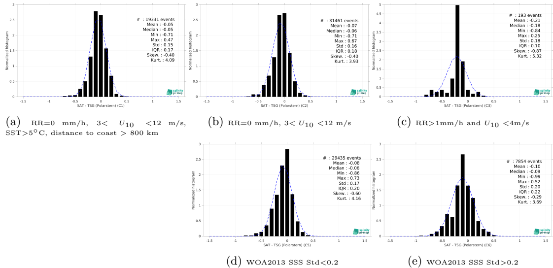
Figure 15: Normalized histogram of \Delta SSS (SMAP SSS L3 v6 - 8-Day running (RSS) - TSG (Polarstern)) for 5 different subdatasets corresponding to: RR=0 mm/h, 3 < U_{10} < 12 m/s, SST >5^\circ C, distance to coast > 800 km (a), RR=0 mm/h, 3 < U_{10} < 12 m/s (b), RR >1 mm/h and U_{10} < 4 m/s (c), WOA2013 SSS Std <0.2 (d), WOA2013 SSS Std >0.2 (e).
