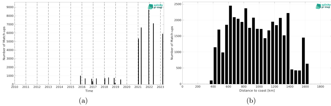
Figure 2: Number of match-ups between TSG (Polarstern) and SMAP SSS L3 v6 - 8-Day running (RSS) SSS as a function of time (a) and as function of the distance to coast (b) over the Equatorial Ocean 10N-10S Pi-MEP region and for the full satellite product period.
