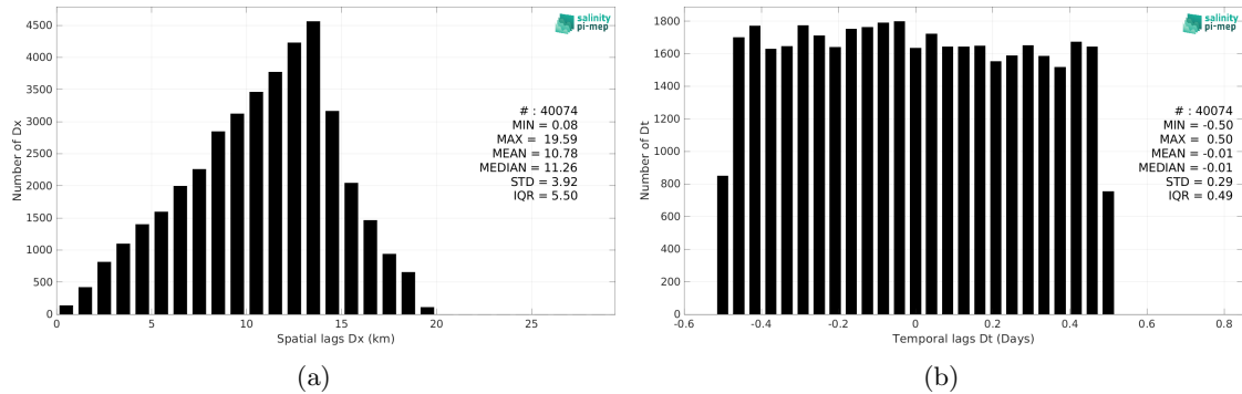
Figure 6: Histograms of the spatial (a) and temporal (b) lags between the location/time of the TSG (Polarstern) measurement and the date of the corresponding SMAP SSS L3 v6 - 8-Day running (RSS) SSS pixel.
