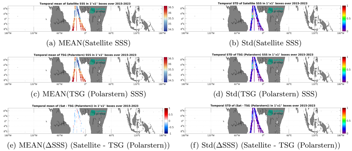
Figure 7: Temporal mean (left) and Std (right) of SSS from SMAP SSS L3 v6 - 8-Day running (RSS) (top), TSG (Polarstern) (middle), and of \Delta SSS (Satellite - TSG (Polarstern)). Only match-up pairs are used to generate these maps.
