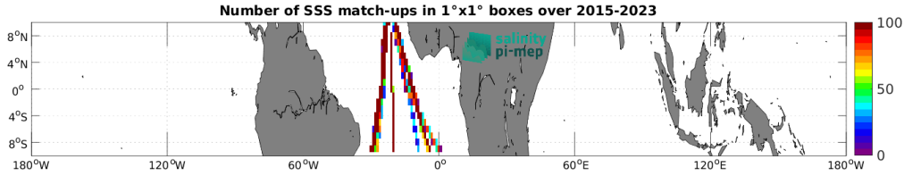
Figure 5: Number of SSS match-ups between TSG (Polarstern) SSS and the SMAP SSS L3 v6 - 8-Day running (RSS) SSS product for the Equatorial Ocean 10N-10S Pi-MEP region over 1^\circ \times 1^\circ boxes and for the full satellite product period.
