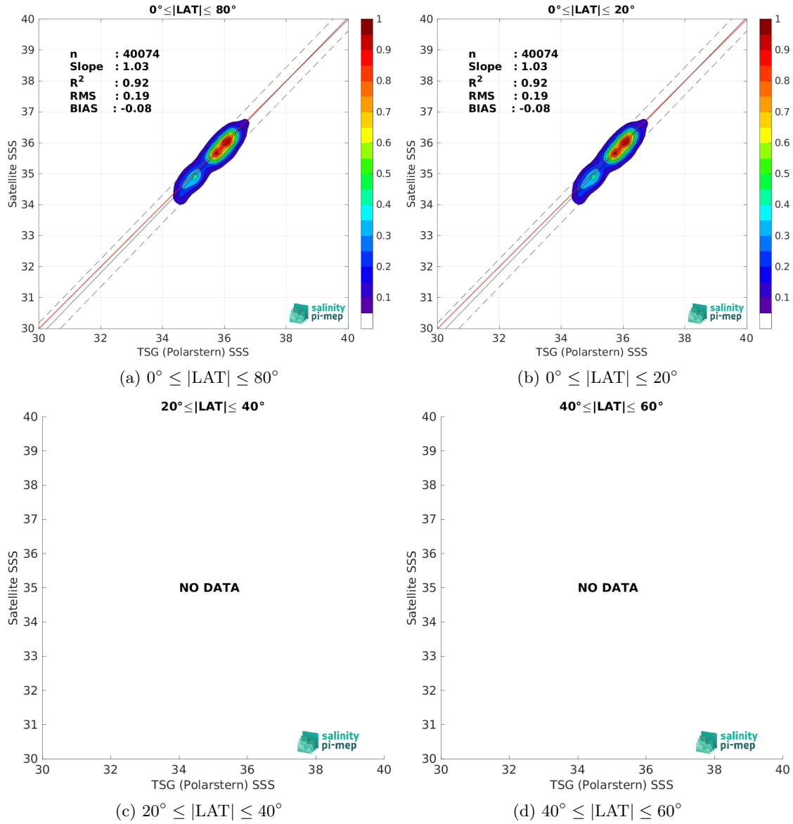
Figure 10: Contour maps of the concentration of SMAP SSS L3 v6 - 8-Day running (RSS) SSS (y-axis) versus TSG (Polarstern) SSS (x-axis) at match-up pairs for different latitude bands. For each plot, the red line shows x=y . The black thin and dashed lines indicate a linear fit through the data cloud and the \pm 95\% confidence levels, respectively. The number match-up pairs n , the slope and R^2 coefficient of the linear fit, the root mean square (RMS) and the mean bias between satellite and in situ data are indicated for each latitude band in each plots.
