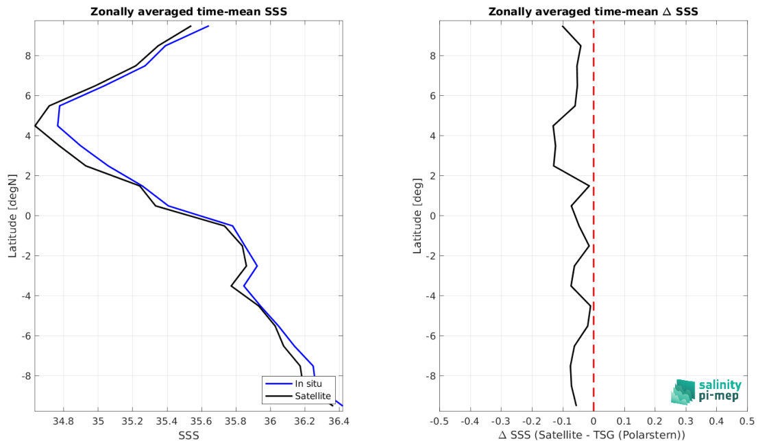
Figure 9: Left panel: Zonal mean SSS from SMAP SSS L3 v6 - 8-Day running (RSS) satellite product (black) and from TSG (Polarstern) (blue). Right panel: Zonal mean of \Delta SSS (Satellite - TSG (Polarstern)) for all the collected Pi-MEP match-up pairs estimated over the full satellite product period.
