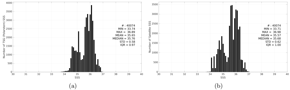
Figure 3: Histograms of SSS from TSG (Polarstern) (a) and SMAP SSS L3 v6 - 8-Day running (RSS) (b) considering all match-up pairs per bins of 0.1 over the Equatorial Ocean 10N-10S Pi-MEP region and for the full satellite product period.
