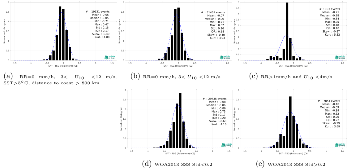
Figure 15: Normalized histogram of \Delta SSS (SMAP SSS L3 v6 - 8-Day running (RSS) - TSG (Polarstern)) for 5 different subdatasets corresponding to: RR=0 mm/h, 3 < U_{10} < 12 m/s, SST >5^\circ C, distance to coast > 800 km (a), RR=0 mm/h, 3 < U_{10} < 12 m/s (b), RR >1 mm/h and U_{10} < 4 m/s (c), WOA2013 SSS Std <0.2 (d), WOA2013 SSS Std >0.2 (e).
