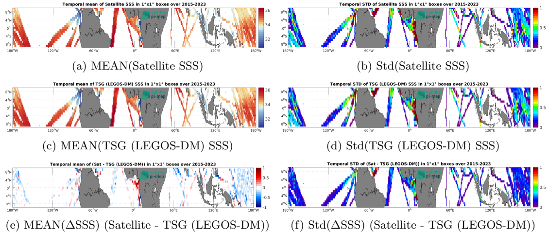
Figure 7: Temporal mean (left) and Std (right) of SSS from SMAP SSS L3 v6 - 8-Day running (RSS) (top), TSG (LEGOS-DM) (middle), and of \Delta SSS (Satellite - TSG (LEGOS-DM)). Only match-up pairs are used to generate these maps.
