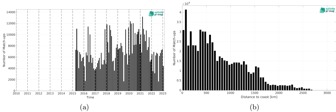
Figure 2: Number of match-ups between TSG (LEGOS-DM) and SMAP SSS L3 v6 - 8-Day running (RSS) SSS as a function of time (a) and as function of the distance to coast (b) over the Equatorial Ocean 10N-10S Pi-MEP region and for the full satellite product period.
