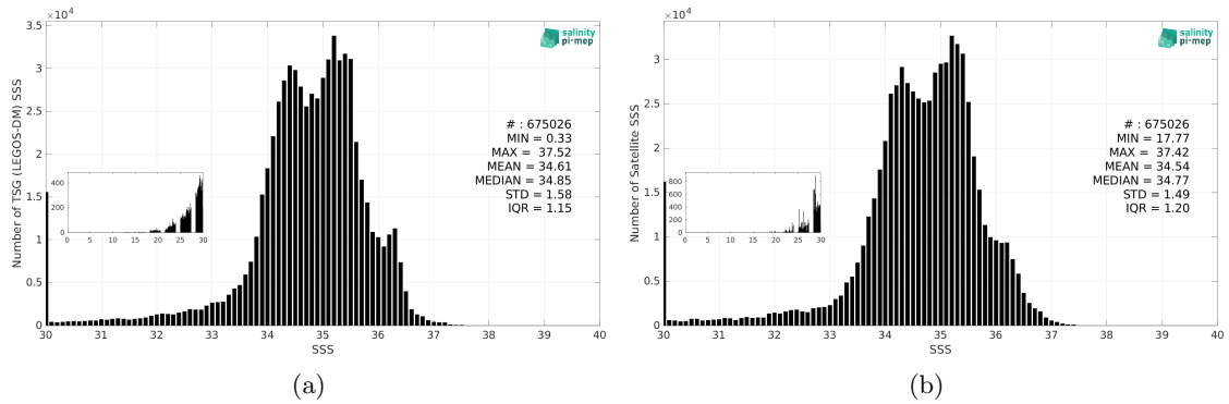
Figure 3: Histograms of SSS from TSG (LEGOS-DM) (a) and SMAP SSS L3 v6 - 8-Day running (RSS) (b) considering all match-up pairs per bins of 0.1 over the Equatorial Ocean 10N-10S Pi-MEP region and for the full satellite product period.
