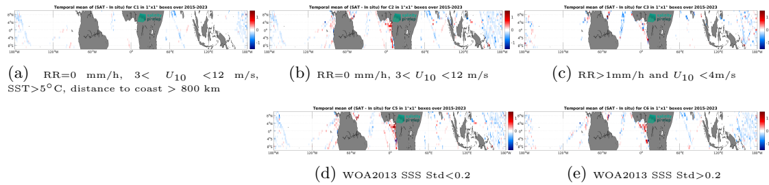
Figure 14: Temporal mean gridded over spatial boxes of size 1^\circ \times 1^\circ of \Delta SSS (SMAP SSS L3 v6 - 8-Day running (RSS) - TSG (LEGOS-DM)) for 5 different subdatasets corresponding to:RR=0 mm/h, 3 < U_{10} < 12 m/s, SST>5°C, distance to coast > 800 km (a), RR=0 mm/h, 3 < U_{10} < 12 m/s (b), RR>1mm/h and U_{10} < 4 m/s (c), WOA2013 SSS Std<0.2 (d), WOA2013 SSS Std>0.2 (e).
