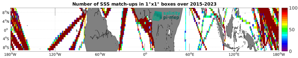
Figure 5: Number of SSS match-ups between TSG (LEGOS-DM) SSS and the SMAP SSS L3 v6 - 8-Day running (RSS) SSS product for the Equatorial Ocean 10N-10S Pi-MEP region over 1^\circ \times 1^\circ boxes and for the full satellite product period.
