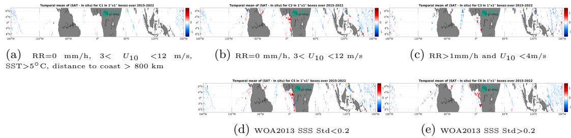
Figure 14: Temporal mean gridded over spatial boxes of size 1^\circ \times 1^\circ of \Delta\text{SSS} (SMAP SSS L3 v6 - 8-Day running (RSS) - TSG (LEGOS-DM)) for 5 different subdatasets corresponding to: RR=0 mm/h, 3 < U_{10} < 12 m/s, SST>5°C, distance to coast > 800 km (a), RR=0 mm/h, 3 < U_{10} < 12 m/s (b), RR>1mm/h and U_{10} < 4 m/s (c), WOA2013 SSS Std<0.2 (d), WOA2013 SSS Std>0.2 (e).
