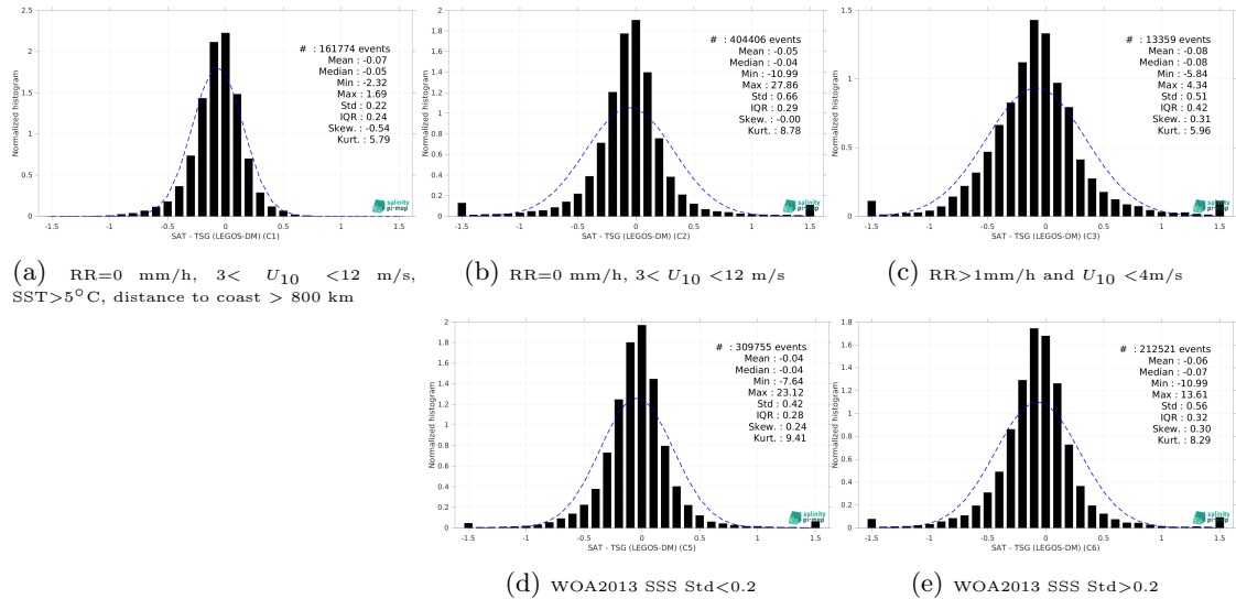
Figure 15: Normalized histogram of \Delta\text{SSS} (SMAP SSS L3 v6 - 8-Day running (RSS) - TSG (LEGOS-DM)) for 5 different subdatasets corresponding to: RR=0 mm/h, 3 < U_{10} < 12 m/s, SST>5°C, distance to coast > 800 km (a), RR=0 mm/h, 3 < U_{10} < 12 m/s (b), RR>1mm/h and U_{10} < 4 m/s (c), WOA2013 SSS Std<0.2 (d), WOA2013 SSS Std>0.2 (e).
