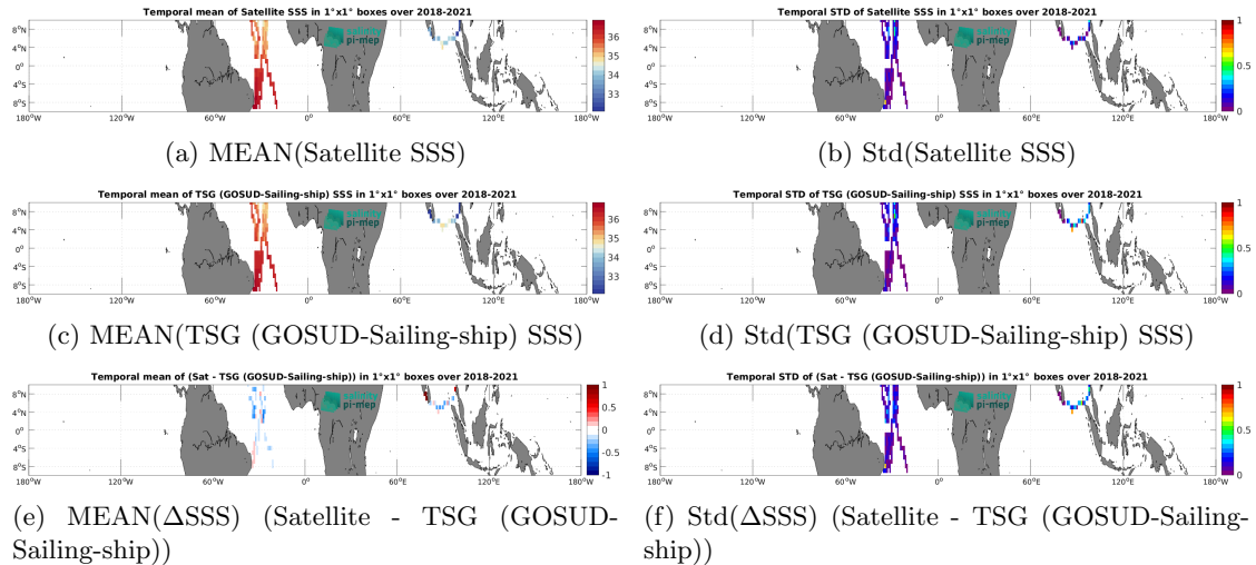
Figure 7: Temporal mean (left) and Std (right) of SSS from SMAP SSS L3 v6 - 8-Day running (RSS) (top), TSG (GOSUD-Sailing-ship) (middle), and of \Delta SSS (Satellite - TSG (GOSUD-Sailing-ship)). Only match-up pairs are used to generate these maps.
