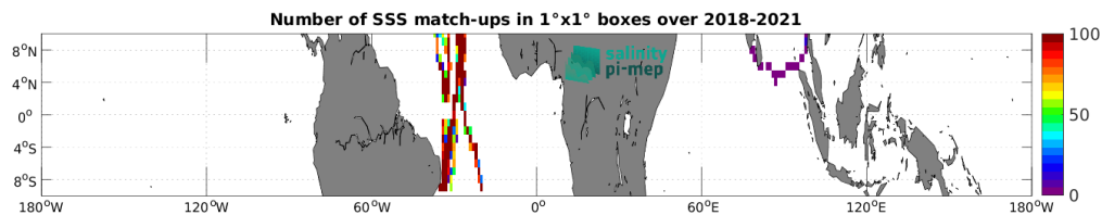
Figure 5: Number of SSS match-ups between TSG (GOSUD-Sailing-ship) SSS and the SMAP SSS L3 v6 - 8-Day running (RSS) SSS product for the Equatorial Ocean 10N-10S Pi-MEP region over 1^\circ \times 1^\circ boxes and for the full satellite product period.
