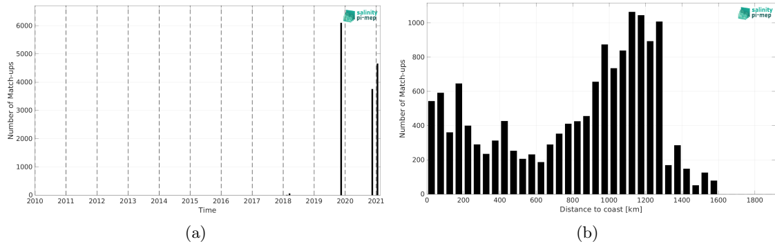
Figure 2: Number of match-ups between TSG (GOSUD-Sailing-ship) and SMAP SSS L3 v6 - 8-Day running (RSS) SSS as a function of time (a) and as function of the distance to coast (b) over the Equatorial Ocean 10N-10S Pi-MEP region and for the full satellite product period.
