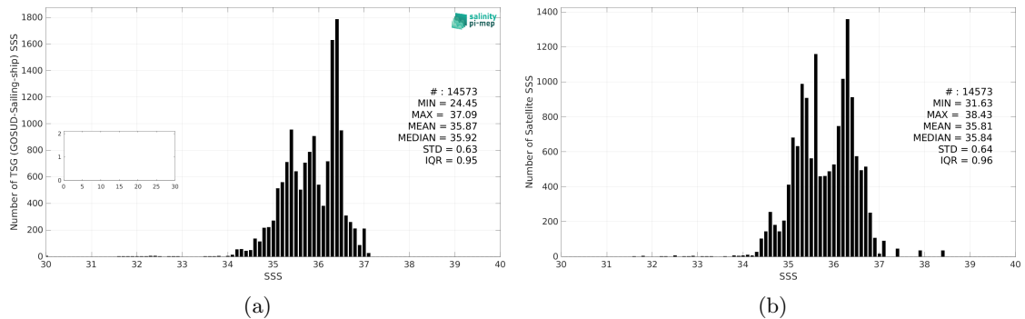
Figure 3: Histograms of SSS from TSG (GOSUD-Sailing-ship) (a) and SMAP SSS L3 v6 - 8-Day running (RSS) (b) considering all match-up pairs per bins of 0.1 over the Equatorial Ocean 10N-10S Pi-MEP region and for the full satellite product period.
