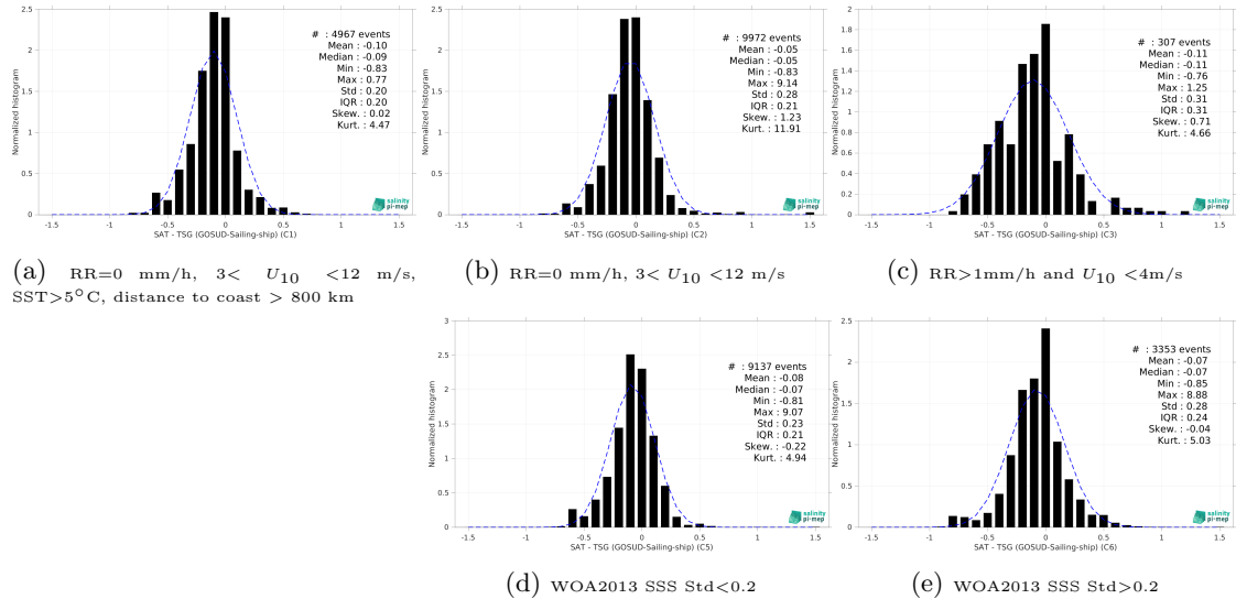
Figure 15: Normalized histogram of \Delta SSS (SMAP SSS L3 v6 - 8-Day running (RSS) - TSG (GOSUD-Sailing-ship)) for 5 different subdatasets corresponding to: RR=0 mm/h, 3 < U_{10} < 12 m/s, SST>5°C, distance to coast > 800 km (a), RR=0 mm/h, 3 < U_{10} < 12 m/s (b), RR>1mm/h and U_{10} < 4 m/s (c), WOA2013 SSS Std<0.2 (d), WOA2013 SSS Std>0.2 (e).
