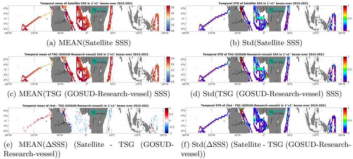
Figure 7: Temporal mean (left) and Std (right) of SSS from SMAP SSS L3 v6 - 8-Day running (RSS) (top), TSG (GOSUD-Research-vessel) (middle), and of \Delta SSS (Satellite - TSG (GOSUD-Research-vessel)). Only match-up pairs are used to generate these maps.
