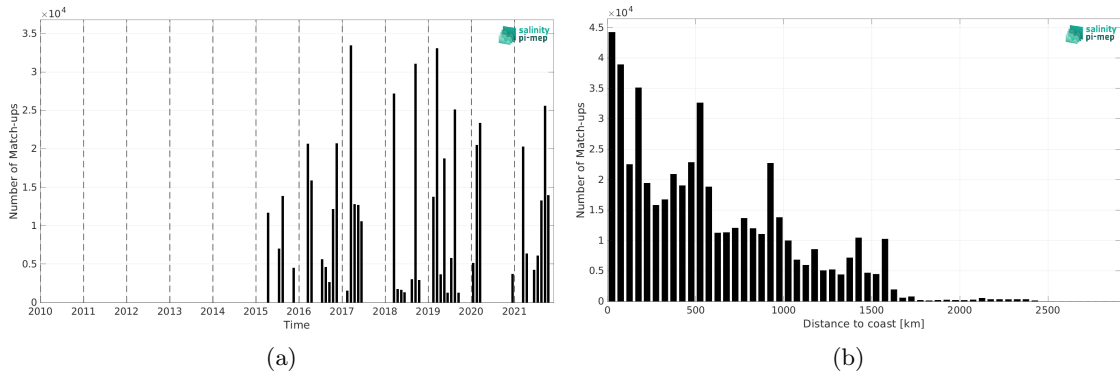
Figure 2: Number of match-ups between TSG (GOSUD-Research-vessel) and SMAP SSS L3 v6 - 8-Day running (RSS) SSS as a function of time (a) and as function of the distance to coast (b) over the Equatorial Ocean 10N-10S Pi-MEP region and for the full satellite product period.
