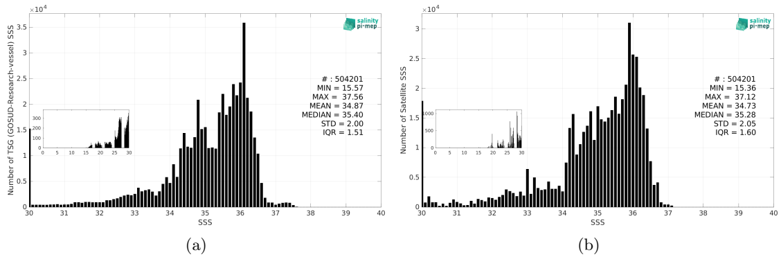
Figure 3: Histograms of SSS from TSG (GOSUD-Research-vessel) (a) and SMAP SSS L3 v6 - 8-Day running (RSS) (b) considering all match-up pairs per bins of 0.1 over the Equatorial Ocean 10N-10S Pi-MEP region and for the full satellite product period.
