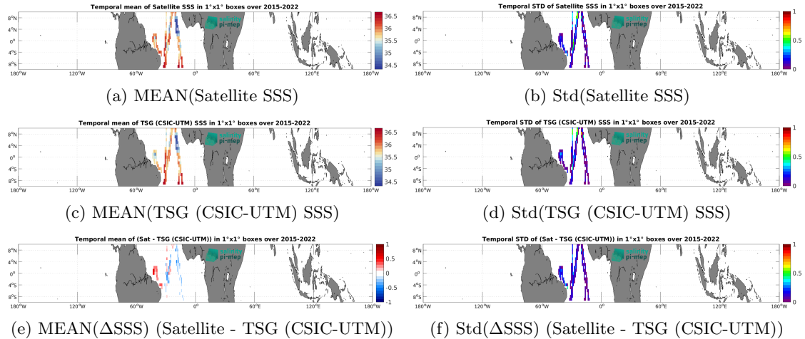
Figure 7: Temporal mean (left) and Std (right) of SSS from SMAP SSS L3 v6 - 8-Day running (RSS) (top), TSG (CSIC-UTM) (middle), and of \Delta SSS (Satellite - TSG (CSIC-UTM)). Only match-up pairs are used to generate these maps.
