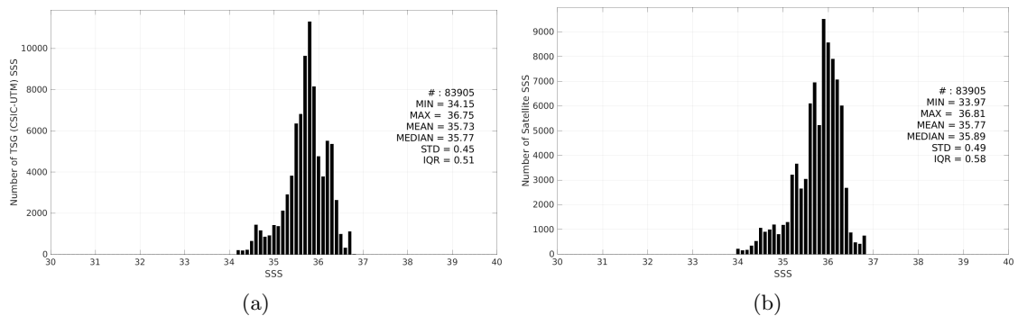
Figure 3: Histograms of SSS from TSG (CSIC-UTM) (a) and SMAP SSS L3 v6 - 8-Day running (RSS) (b) considering all match-up pairs per bins of 0.1 over the Equatorial Ocean 10N-10S Pi-MEP region and for the full satellite product period.
