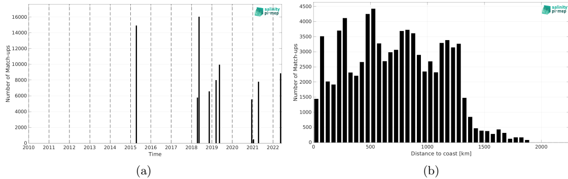
Figure 2: Number of match-ups between TSG (CSIC-UTM) and SMAP SSS L3 v6 - 8-Day running (RSS) SSS as a function of time (a) and as function of the distance to coast (b) over the Equatorial Ocean 10N-10S Pi-MEP region and for the full satellite product period.
