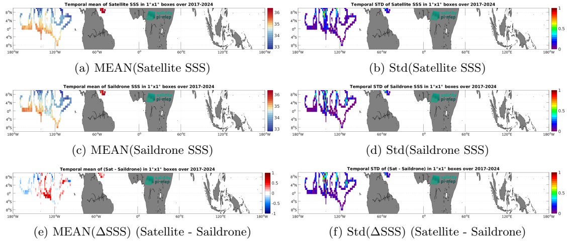
Figure 7: Temporal mean (left) and Std (right) of SSS from SMAP SSS L3 v6 - 8-Day running (RSS) (top), Saildrone (middle), and of \Delta SSS (Satellite - Saildrone). Only match-up pairs are used to generate these maps.
