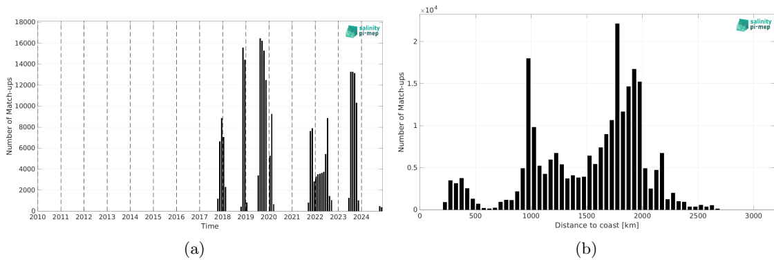
Figure 2: Number of match-ups between Saildrone and SMAP SSS L3 v6 - 8-Day running (RSS) SSS as a function of time (a) and as function of the distance to coast (b) over the Equatorial Ocean 10N-10S Pi-MEP region and for the full satellite product period.
