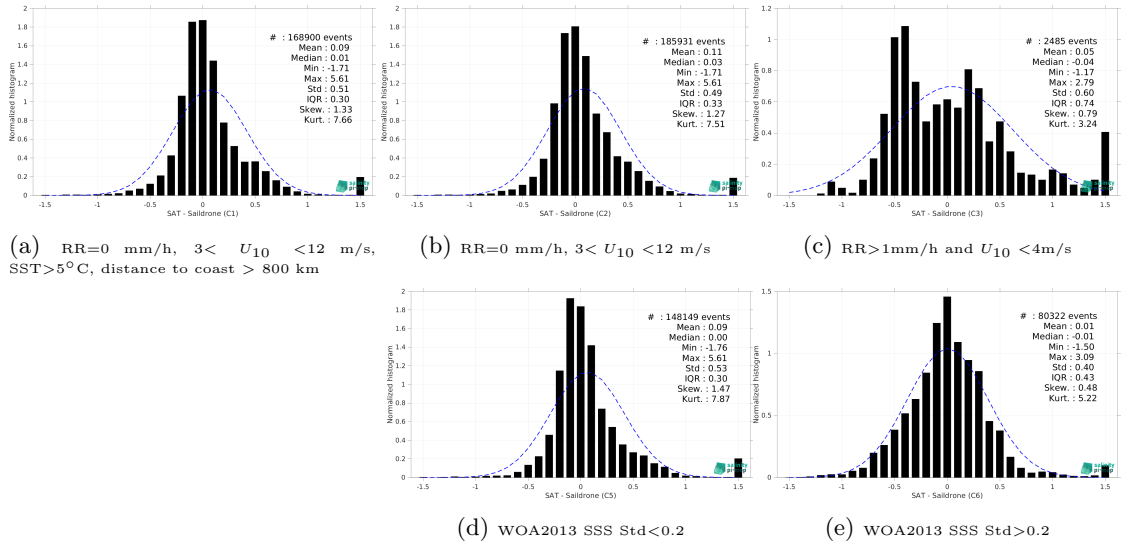
Figure 15: Normalized histogram of \Delta\text{SSS} (SMAP SSS L3 v6 - 8-Day running (RSS) - Saildrone) for 5 different subdatasets corresponding to: RR=0 mm/h, 3 < U_{10} < 12 m/s, SST>5°C, distance to coast > 800 km (a), RR=0 mm/h, 3 < U_{10} < 12 m/s (b), RR>1mm/h and U_{10} < 4 m/s (c), WOA2013 SSS Std<0.2 (d), WOA2013 SSS Std>0.2 (e).
