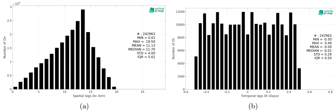
Figure 6: Histograms of the spatial (a) and temporal (b) lags between the location/time of the Saildrone measurement and the date of the corresponding SMAP SSS L3 v6 - 8-Day running (RSS) SSS pixel.
