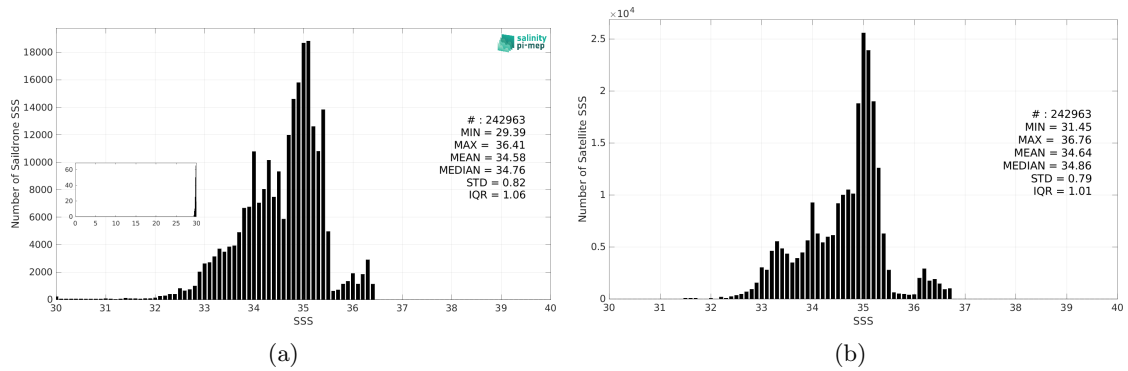
Figure 3: Histograms of SSS from Saildrone (a) and SMAP SSS L3 v6 - 8-Day running (RSS) (b) considering all match-up pairs per bins of 0.1 over the Equatorial Ocean 10N-10S Pi-MEP region and for the full satellite product period.
