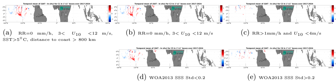
Figure 14: Temporal mean gridded over spatial boxes of size 1^\circ \times 1^\circ of \Delta\text{SSS} (SMAP SSS L3 v6 - 8-Day running (RSS) - Saildrone) for 5 different subdatasets corresponding to:RR=0 mm/h, 3 < U_{10} < 12 m/s, SST>5°C, distance to coast > 800 km (a), RR=0 mm/h, 3 < U_{10} < 12 m/s (b), RR>1mm/h and U_{10} < 4 m/s (c), WOA2013 SSS Std<0.2 (d), WOA2013 SSS Std>0.2 (e).
