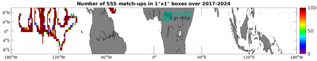
Figure 5: Number of SSS match-ups between Saildrone SSS and the SMAP SSS L3 v6 - 8-Day running (RSS) SSS product for the Equatorial Ocean 10N-10S Pi-MEP region over 1^\circ \times 1^\circ boxes and for the full satellite product period.
