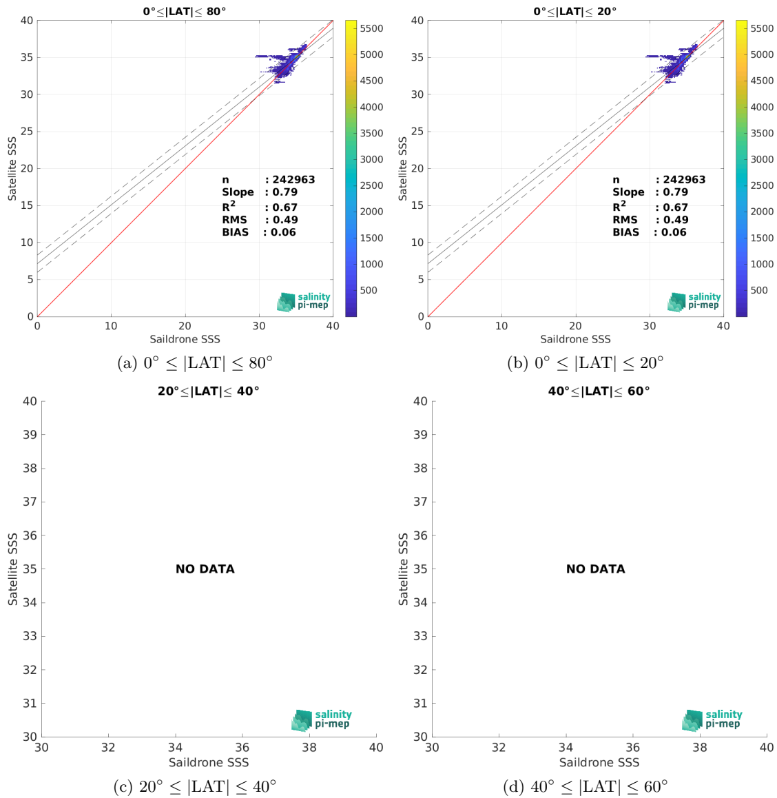
Figure 10: Contour maps of the concentration of SMAP SSS L3 v6 - 8-Day running (RSS) SSS (y-axis) versus Sairdrone SSS (x-axis) at match-up pairs for different latitude bands. For each plot, the red line shows x=y . The black thin and dashed lines indicate a linear fit through the data cloud and the \pm 95\% confidence levels, respectively. The number match-up pairs n , the slope and R^2 coefficient of the linear fit, the root mean square (RMS) and the mean bias between satellite and in situ data are indicated for each latitude band in each plots.
