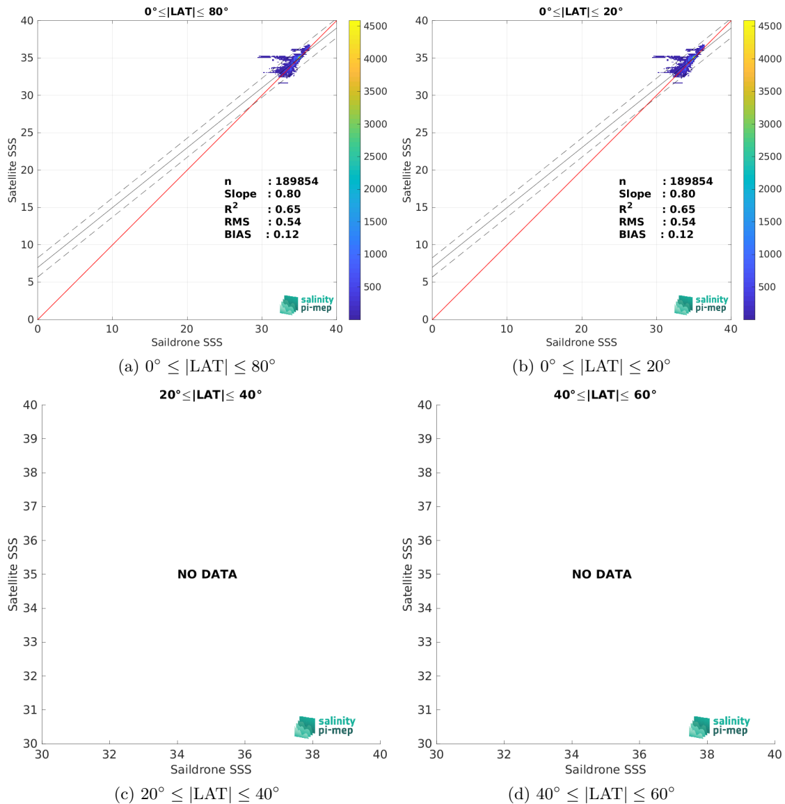
Figure 10: Contour maps of the concentration of SMAP SSS L3 v6 - 8-Day running (RSS) SSS (y-axis) versus Sairdron SSS (x-axis) at match-up pairs for different latitude bands. For each plot, the red line shows x=y . The black thin and dashed lines indicate a linear fit through the data cloud and the \pm 95\% confidence levels, respectively. The number match-up pairs n , the slope and R^2 coefficient of the linear fit, the root mean square (RMS) and the mean bias between satellite and in situ data are indicated for each latitude band in each plots.
