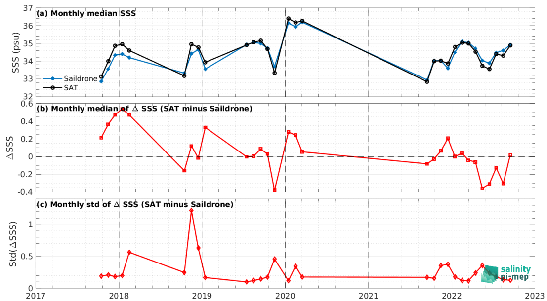
Figure 8: Time series of the monthly median SSS (top), median of \Delta SSS (Satellite - Sairdrone) and Std of \Delta SSS (Satellite - Sairdrone) over the Equatorial Ocean 10N-10S Pi-MEP region considering all match-ups collected by the Pi-MEP.
