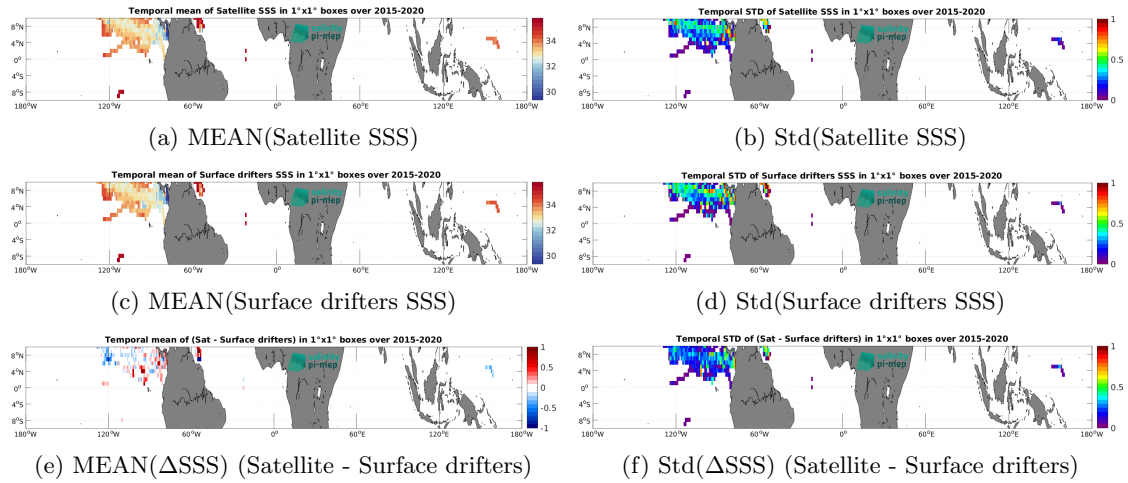
Figure 6: Temporal mean (left) and Std (right) of SSS from SMAP SSS L3 v6 - 8-Day running (RSS) (top), Surface drifters (middle), and of \Delta SSS (Satellite - Surface drifters). Only match-up pairs are used to generate these maps.
