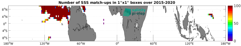
Figure 4: Number of SSS match-ups between Surface drifters SSS and the SMAP SSS L3 v6 - 8-Day running (RSS) SSS product for the Equatorial Ocean 10N-10S Pi-MEP region over 1^\circ \times 1^\circ boxes and for the full satellite product period.
