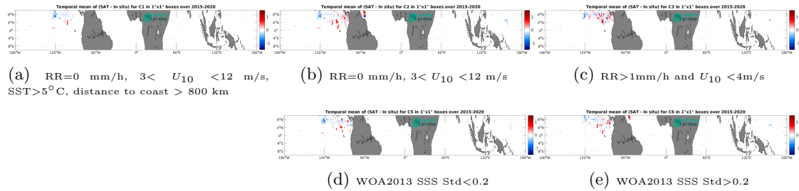
Figure 13: Temporal mean gridded over spatial boxes of size 1^\circ \times 1^\circ of \Delta SSS (SMAP SSS L3 v6 - 8-Day running (RSS) - Surface drifters) for 5 different subdatasets corresponding to: RR=0 mm/h, 3 < U_{10} < 12 m/s, SST >5^\circ C, distance to coast > 800 km (a), RR=0 mm/h, 3 < U_{10} < 12 m/s (b), RR >1 mm/h and U_{10} < 4 m/s (c), WOA2013 SSS Std <0.2 (d), WOA2013 SSS Std >0.2 (e).
