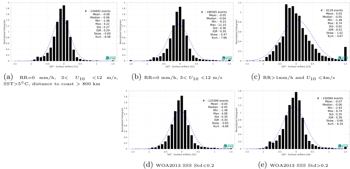
Figure 14: Normalized histogram of \Delta SSS (SMAP SSS L3 v6 - 8-Day running (RSS) - Surface drifters) for 5 different subdatasets corresponding to: RR=0 mm/h, 3 < U_{10} < 12 m/s, SST >5^\circ C, distance to coast > 800 km (a), RR=0 mm/h, 3 < U_{10} < 12 m/s (b), RR >1 mm/h and U_{10} < 4 m/s (c), WOA2013 SSS Std <0.2 (d), WOA2013 SSS Std >0.2 (e).
