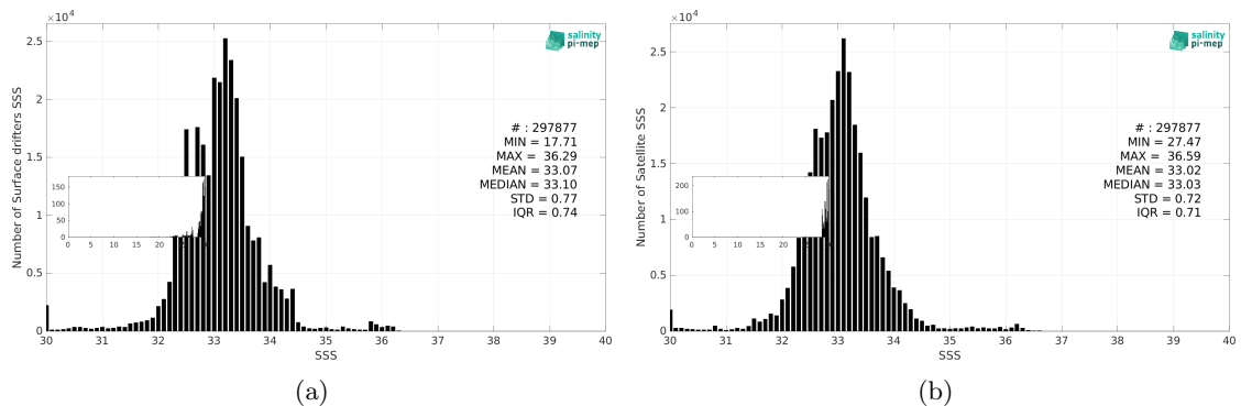
Figure 3: Histograms of SSS from Surface drifters (a) and SMAP SSS L3 v6 - 8-Day running (RSS) (b) considering all match-up pairs per bins of 0.1 over the Equatorial Ocean 10N-10S Pi-MEP region and for the full satellite product period.
