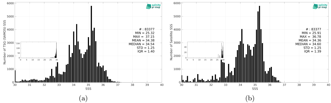
Figure 3: Histograms of SSS from TSG (SAMOS) (a) and SMAP SSS L3 v6 - Monthly (RSS) (b) considering all match-up pairs per bins of 0.1 over the Equatorial Ocean 10N-10S Pi-MEP region and for the full satellite product period.
