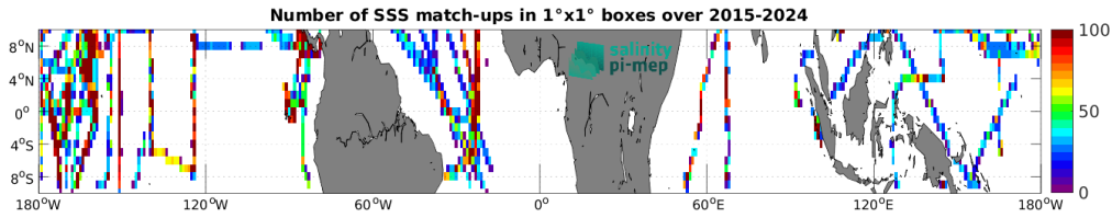
Figure 5: Number of SSS match-ups between TSG (SAMOS) SSS and the SMAP SSS L3 v6 - Monthly (RSS) SSS product for the Equatorial Ocean 10N-10S Pi-MEP region over 1^\circ \times 1^\circ boxes and for the full satellite product period.
