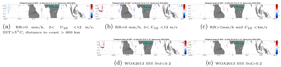
Figure 14: Temporal mean gridded over spatial boxes of size 1^\circ \times 1^\circ of \Delta SSS (SMAP SSS L3 v6 - Monthly (RSS) - TSG (SAMOS)) for 5 different subdatasets corresponding to:RR=0 mm/h, 3 < U_{10} < 12 m/s, SST > 5^\circ C , distance to coast > 800 km (a), RR=0 mm/h, 3 < U_{10} < 12 m/s (b), RR>1mm/h and U_{10} < 4 m/s (c), WOA2013 SSS Std<0.2 (d), WOA2013 SSS Std>0.2 (e).
