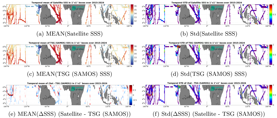
Figure 7: Temporal mean (left) and Std (right) of SSS from SMAP SSS L3 v6 - Monthly (RSS) (top), TSG (SAMOS) (middle), and of \Delta SSS (Satellite - TSG (SAMOS)). Only match-up pairs are used to generate these maps.
