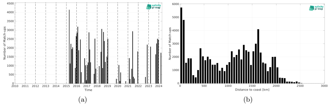
Figure 2: Number of match-ups between TSG (SAMOS) and SMAP SSS L3 v6 - Monthly (RSS) SSS as a function of time (a) and as function of the distance to coast (b) over the Equatorial Ocean 10N-10S Pi-MEP region and for the full satellite product period.
