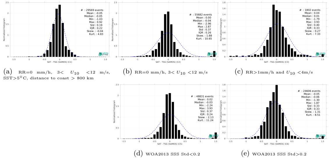
Figure 15: Normalized histogram of \Delta SSS (SMAP SSS L3 v6 - Monthly (RSS) - TSG (SAMOS)) for 5 different subdatasets corresponding to: RR=0 mm/h, 3 < U_{10} < 12 m/s, SST > 5^\circ C , distance to coast > 800 km (a), RR=0 mm/h, 3 < U_{10} < 12 m/s (b), RR>1mm/h and U_{10} < 4 m/s (c), WOA2013 SSS Std<0.2 (d), WOA2013 SSS Std>0.2 (e).
