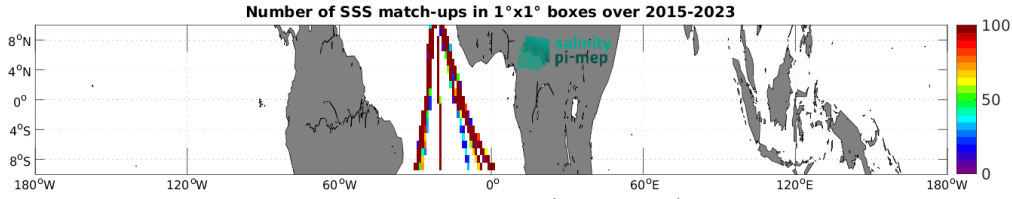
Figure 5: Number of SSS match-ups between TSG (Polarstern) SSS and the SMAP SSS L3 v6 - Monthly (RSS) SSS product for the Equatorial Ocean 10N-10S Pi-MEP region over 1^\circ \times 1^\circ boxes and for the full satellite product period.
