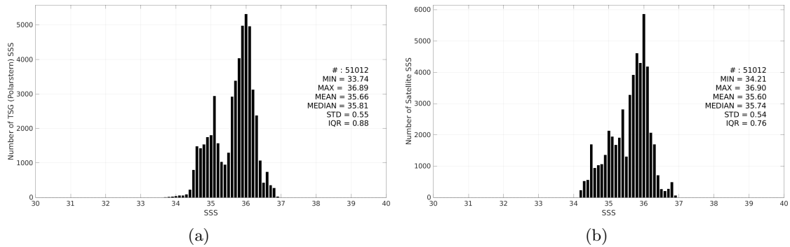
Figure 3: Histograms of SSS from TSG (Polarstern) (a) and SMAP SSS L3 v6 - Monthly (RSS) (b) considering all match-up pairs per bins of 0.1 over the Equatorial Ocean 10N-10S Pi-MEP region and for the full satellite product period.
