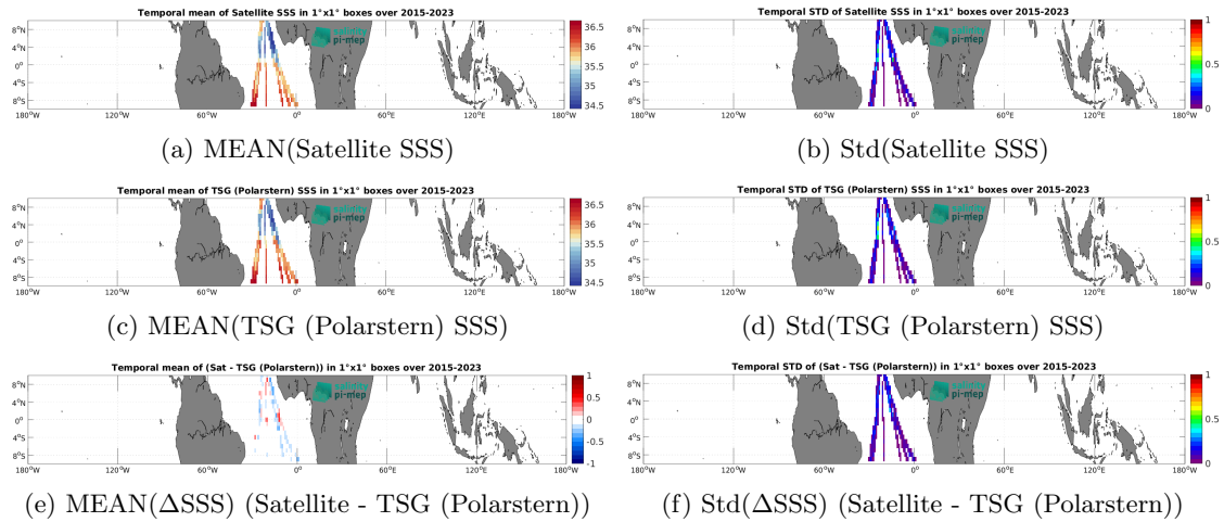
Figure 7: Temporal mean (left) and Std (right) of SSS from SMAP SSS L3 v6 - Monthly (RSS) (top), TSG (Polarstern) (middle), and of \Delta SSS (Satellite - TSG (Polarstern)). Only match-up pairs are used to generate these maps.
