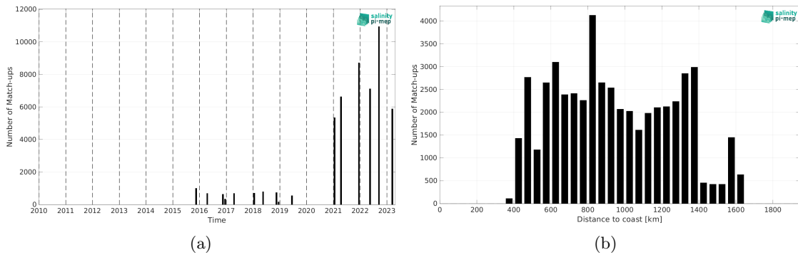
Figure 2: Number of match-ups between TSG (Polarstern) and SMAP SSS L3 v6 - Monthly (RSS) SSS as a function of time (a) and as function of the distance to coast (b) over the Equatorial Ocean 10N-10S Pi-MEP region and for the full satellite product period.
