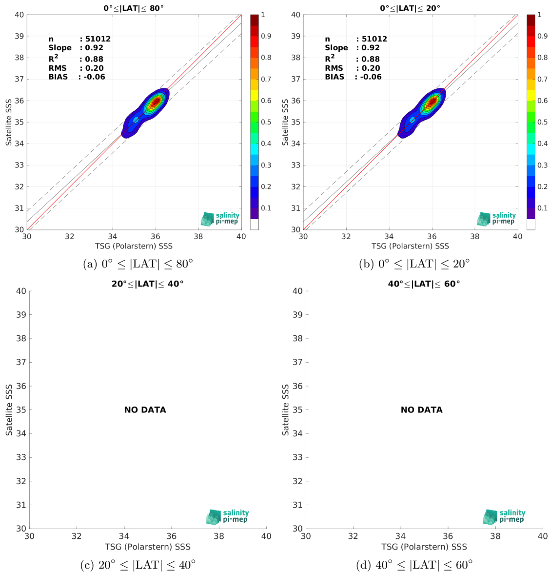
Figure 10: Contour maps of the concentration of SMAP SSS L3 v6 - Monthly (RSS) SSS (y-axis) versus TSG (Polarstern) SSS (x-axis) at match-up pairs for different latitude bands. For each plot, the red line shows x=y . The black thin and dashed lines indicate a linear fit through the data cloud and the \pm 95\% confidence levels, respectively. The number match-up pairs n , the slope and R^2 coefficient of the linear fit, the root mean square (RMS) and the mean bias between satellite and in situ data are indicated for each latitude band in each plots.
