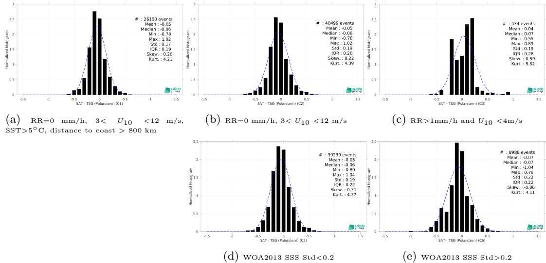
Figure 15: Normalized histogram of \Delta SSS (SMAP SSS L3 v6 - Monthly (RSS) - TSG (Polarstern)) for 5 different subdatasets corresponding to: RR=0 mm/h, 3 < U_{10} < 12 m/s, SST>5°C, distance to coast > 800 km (a), RR=0 mm/h, 3 < U_{10} < 12 m/s (b), RR>1mm/h and U_{10} < 4 m/s (c), WOA2013 SSS Std<0.2 (d), WOA2013 SSS Std>0.2 (e).
