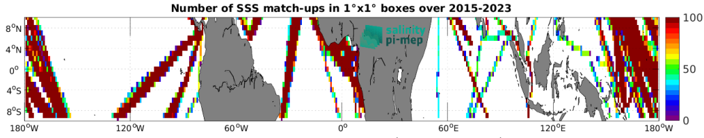
Figure 5: Number of SSS match-ups between TSG (LEGOS-DM) SSS and the SMAP SSS L3 v6 - Monthly (RSS) SSS product for the Equatorial Ocean 10N-10S Pi-MEP region over 1^\circ \times 1^\circ boxes and for the full satellite product period.
