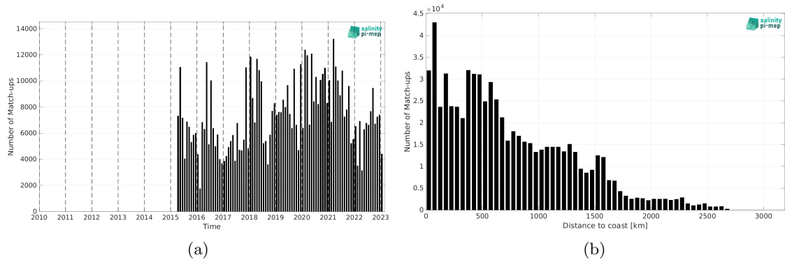
Figure 2: Number of match-ups between TSG (LEGOS-DM) and SMAP SSS L3 v6 - Monthly (RSS) SSS as a function of time (a) and as function of the distance to coast (b) over the Equatorial Ocean 10N-10S Pi-MEP region and for the full satellite product period.
