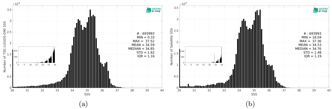
Figure 3: Histograms of SSS from TSG (LEGOS-DM) (a) and SMAP SSS L3 v6 - Monthly (RSS) (b) considering all match-up pairs per bins of 0.1 over the Equatorial Ocean 10N-10S Pi-MEP region and for the full satellite product period.
