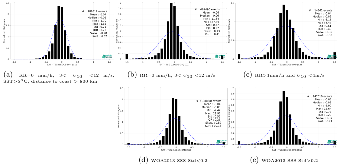
Figure 15: Normalized histogram of \Delta\text{SSS} (SMAP SSS L3 v6 - Monthly (RSS) - TSG (LEGOS-DM)) for 5 different subdatasets corresponding to: RR=0 mm/h, 3 < U_{10} < 12 m/s, SST>5°C, distance to coast > 800 km (a), RR=0 mm/h, 3 < U_{10} < 12 m/s (b), RR>1mm/h and U_{10} < 4 m/s (c), WOA2013 SSS Std<0.2 (d), WOA2013 SSS Std>0.2 (e).
