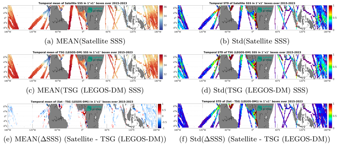
Figure 7: Temporal mean (left) and Std (right) of SSS from SMAP SSS L3 v6 - Monthly (RSS) (top), TSG (LEGOS-DM) (middle), and of \Delta SSS (Satellite - TSG (LEGOS-DM)). Only match-up pairs are used to generate these maps.
