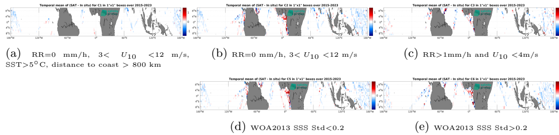
Figure 14: Temporal mean gridded over spatial boxes of size 1^\circ \times 1^\circ of \Delta\text{SSS} (SMAP SSS L3 v6 - Monthly (RSS) - TSG (LEGOS-DM)) for 5 different subdatasets corresponding to: RR=0 mm/h, 3 < U_{10} < 12 m/s, SST>5°C, distance to coast > 800 km (a), RR=0 mm/h, 3 < U_{10} < 12 m/s (b), RR>1mm/h and U_{10} < 4 m/s (c), WOA2013 SSS Std<0.2 (d), WOA2013 SSS Std>0.2 (e).
