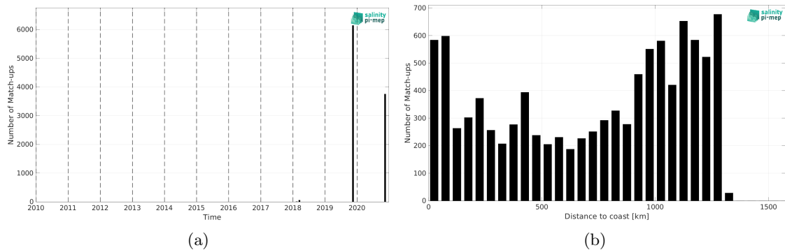
Figure 2: Number of match-ups between TSG (GOSUD-Sailing-ship) and SMAP SSS L3 v6 - Monthly (RSS) SSS as a function of time (a) and as function of the distance to coast (b) over the Equatorial Ocean 10N-10S Pi-MEP region and for the full satellite product period.
