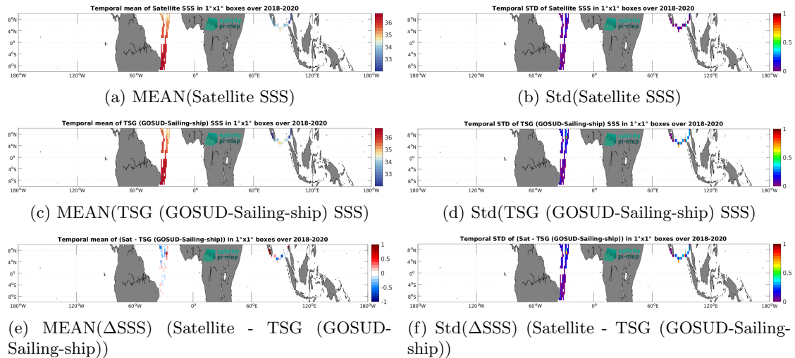
Figure 7: Temporal mean (left) and Std (right) of SSS from SMAP SSS L3 v6 - Monthly (RSS) (top), TSG (GOSUD-Sailing-ship) (middle), and of \Delta SSS (Satellite - TSG (GOSUD-Sailing-ship)). Only match-up pairs are used to generate these maps.
