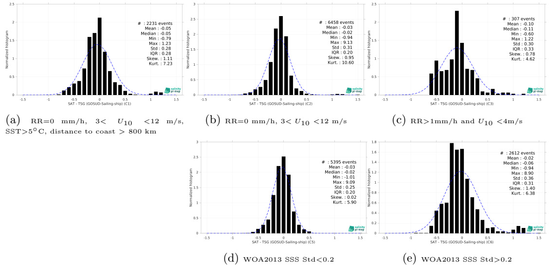
Figure 15: Normalized histogram of \Delta SSS (SMAP SSS L3 v6 - Monthly (RSS) - TSG (GOSUD-Sailing-ship)) for 5 different subdatasets corresponding to: RR=0 mm/h, 3 < U_{10} < 12 m/s, SST>5°C, distance to coast > 800 km (a), RR=0 mm/h, 3 < U_{10} < 12 m/s (b), RR>1mm/h and U_{10} < 4 m/s (c), WOA2013 SSS Std<0.2 (d), WOA2013 SSS Std>0.2 (e).
