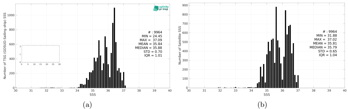
Figure 3: Histograms of SSS from TSG (GOSUD-Sailing-ship) (a) and SMAP SSS L3 v6 - Monthly (RSS) (b) considering all match-up pairs per bins of 0.1 over the Equatorial Ocean 10N-10S Pi-MEP region and for the full satellite product period.
