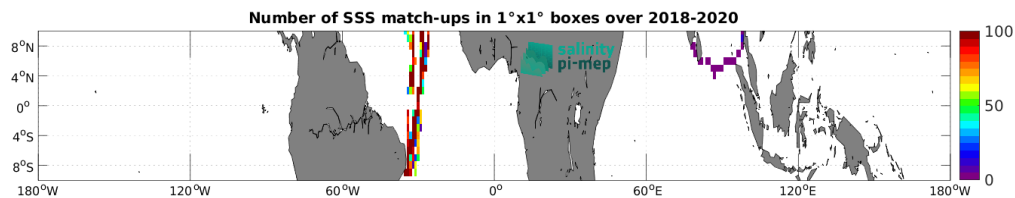
Figure 5: Number of SSS match-ups between TSG (GOSUD-Sailing-ship) SSS and the SMAP SSS L3 v6 - Monthly (RSS) SSS product for the Equatorial Ocean 10N-10S Pi-MEP region over 1^\circ \times 1^\circ boxes and for the full satellite product period.
