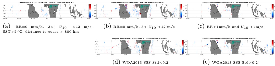
Figure 14: Temporal mean gridded over spatial boxes of size 1^\circ \times 1^\circ of \Delta SSS (SMAP SSS L3 v6 - Monthly (RSS) - TSG (GOSUD-Research-vessel)) for 5 different subdatasets corresponding to: RR=0 mm/h, 3 < U_{10} < 12 m/s, SST >5^\circ C, distance to coast > 800 km (a), RR=0 mm/h, 3 < U_{10} < 12 m/s (b), RR >1 mm/h and U_{10} < 4 m/s (c), WOA2013 SSS Std <0.2 (d), WOA2013 SSS Std >0.2 (e).
