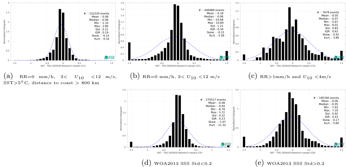
Figure 15: Normalized histogram of \Delta SSS (SMAP SSS L3 v6 - Monthly (RSS) - TSG (GOSUD-Research-vessel)) for 5 different subdatasets corresponding to: RR=0 mm/h, 3 < U_{10} < 12 m/s, SST >5^\circ C, distance to coast > 800 km (a), RR=0 mm/h, 3 < U_{10} < 12 m/s (b), RR >1 mm/h and U_{10} < 4 m/s (c), WOA2013 SSS Std <0.2 (d), WOA2013 SSS Std >0.2 (e).
