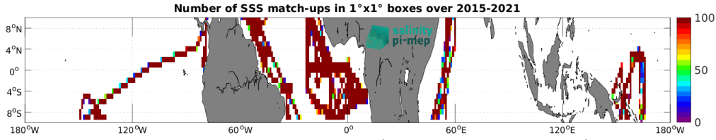
Figure 5: Number of SSS match-ups between TSG (GOSUD-Research-vessel) SSS and the SMAP SSS L3 v6 - Monthly (RSS) SSS product for the Equatorial Ocean 10N-10S Pi-MEP region over 1^\circ \times 1^\circ boxes and for the full satellite product period.
