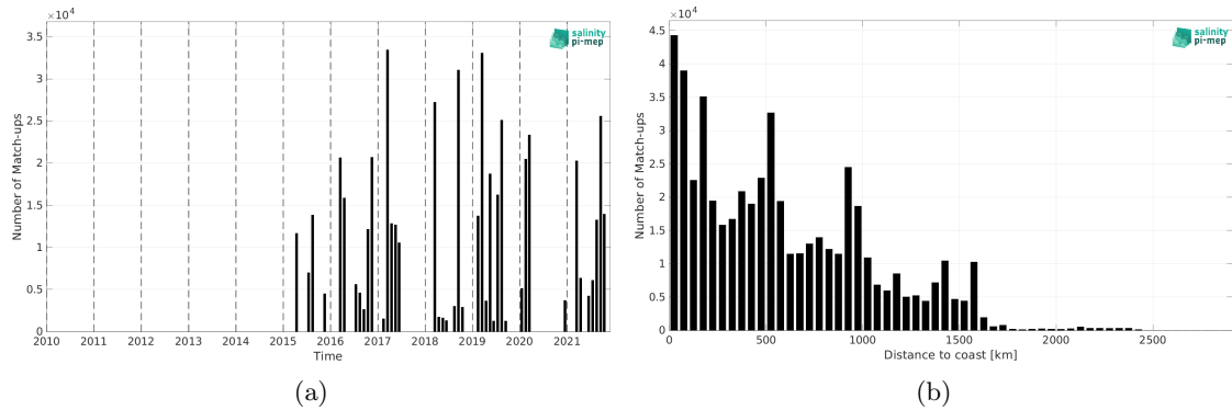
Figure 2: Number of match-ups between TSG (GOSUD-Research-vessel) and SMAP SSS L3 v6 - Monthly (RSS) SSS as a function of time (a) and as function of the distance to coast (b) over the Equatorial Ocean 10N-10S Pi-MEP region and for the full satellite product period.
