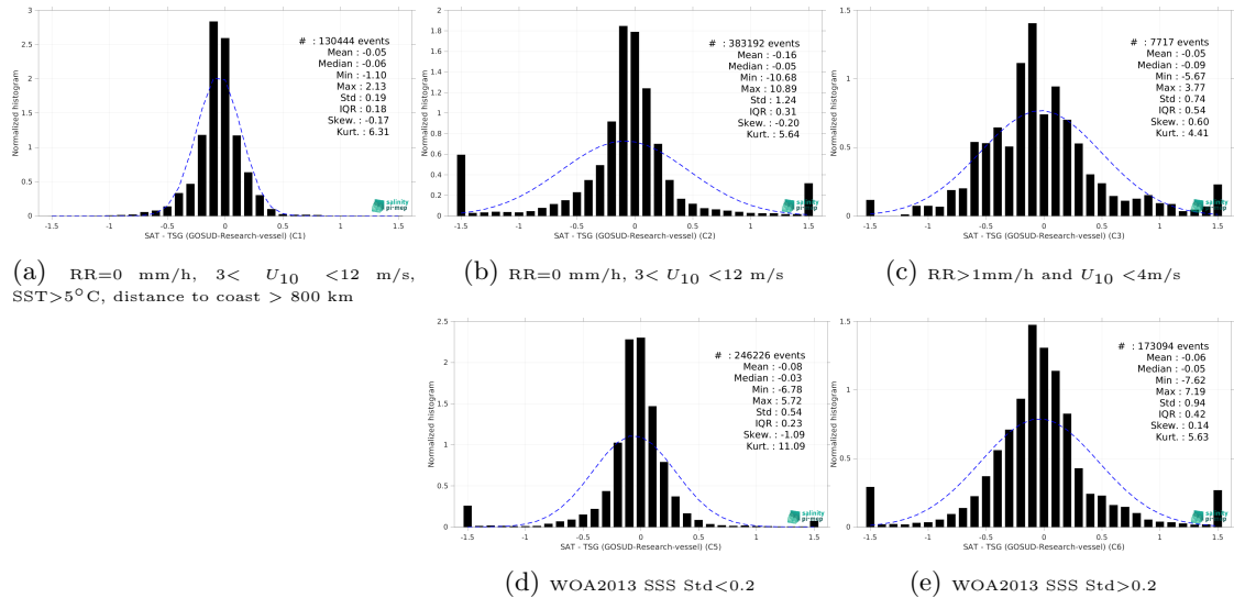
Figure 15: Normalized histogram of \Delta\text{SSS} (SMAP SSS L3 v6 - Monthly (RSS) - TSG (GOSUD-Research-vessel)) for 5 different subdatasets corresponding to: RR=0 mm/h, 3 < U_{10} < 12 m/s, SST>5°C, distance to coast > 800 km (a), RR=0 mm/h, 3 < U_{10} < 12 m/s (b), RR>1mm/h and U_{10} < 4 m/s (c), WOA2013 SSS Std<0.2 (d), WOA2013 SSS Std>0.2 (e).
