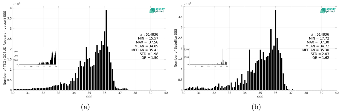
Figure 3: Histograms of SSS from TSG (GOSUD-Research-vessel) (a) and SMAP SSS L3 v6 - Monthly (RSS) (b) considering all match-up pairs per bins of 0.1 over the Equatorial Ocean 10N-10S Pi-MEP region and for the full satellite product period.
