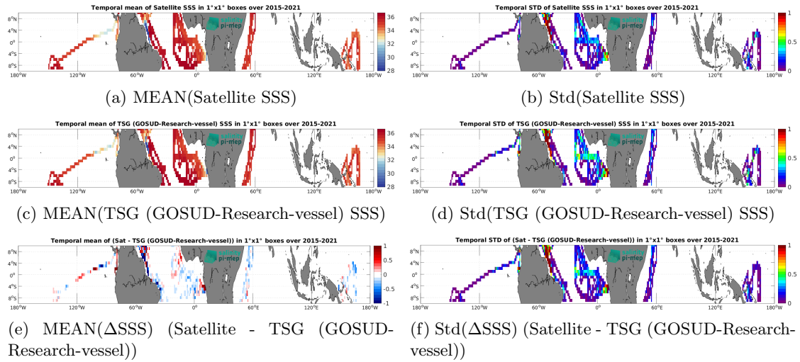
Figure 7: Temporal mean (left) and Std (right) of SSS from SMAP SSS L3 v6 - Monthly (RSS) (top), TSG (GOSUD-Research-vessel) (middle), and of \Delta SSS (Satellite - TSG (GOSUD-Research-vessel)). Only match-up pairs are used to generate these maps.
