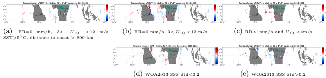
Figure 14: Temporal mean gridded over spatial boxes of size 1^\circ \times 1^\circ of \Delta\text{SSS} (SMAP SSS L3 v6 - Monthly (RSS) - TSG (GOSUD-Research-vessel)) for 5 different subdatasets corresponding to: RR=0 mm/h, 3 < U_{10} < 12 m/s, SST>5°C, distance to coast > 800 km (a), RR=0 mm/h, 3 < U_{10} < 12 m/s (b), RR>1mm/h and U_{10} < 4 m/s (c), WOA2013 SSS Std<0.2 (d), WOA2013 SSS Std>0.2 (e).
