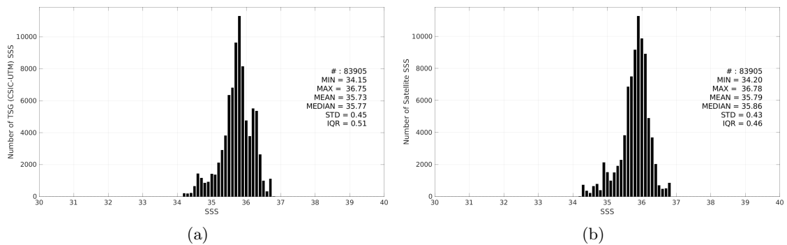
Figure 3: Histograms of SSS from TSG (CSIC-UTM) (a) and SMAP SSS L3 v6 - Monthly (RSS) (b) considering all match-up pairs per bins of 0.1 over the Equatorial Ocean 10N-10S Pi-MEP region and for the full satellite product period.
