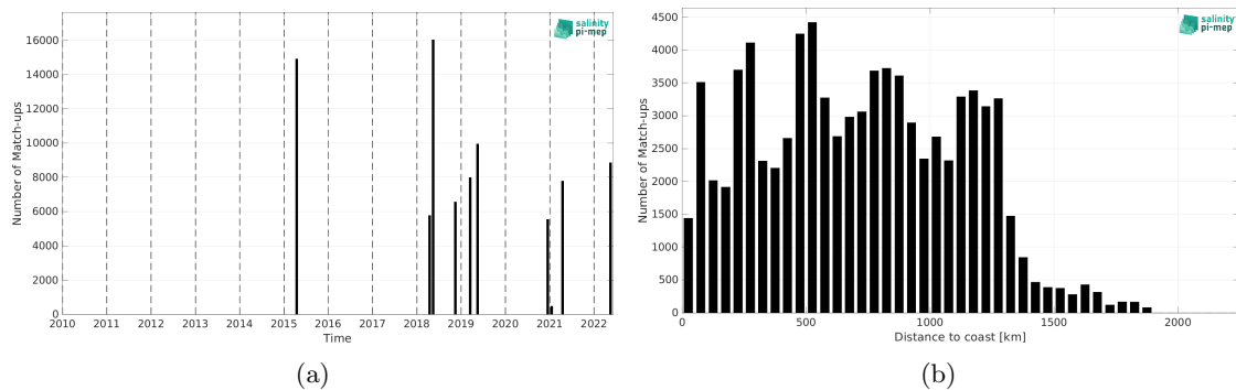
Figure 2: Number of match-ups between TSG (CSIC-UTM) and SMAP SSS L3 v6 - Monthly (RSS) SSS as a function of time (a) and as function of the distance to coast (b) over the Equatorial Ocean 10N-10S Pi-MEP region and for the full satellite product period.
