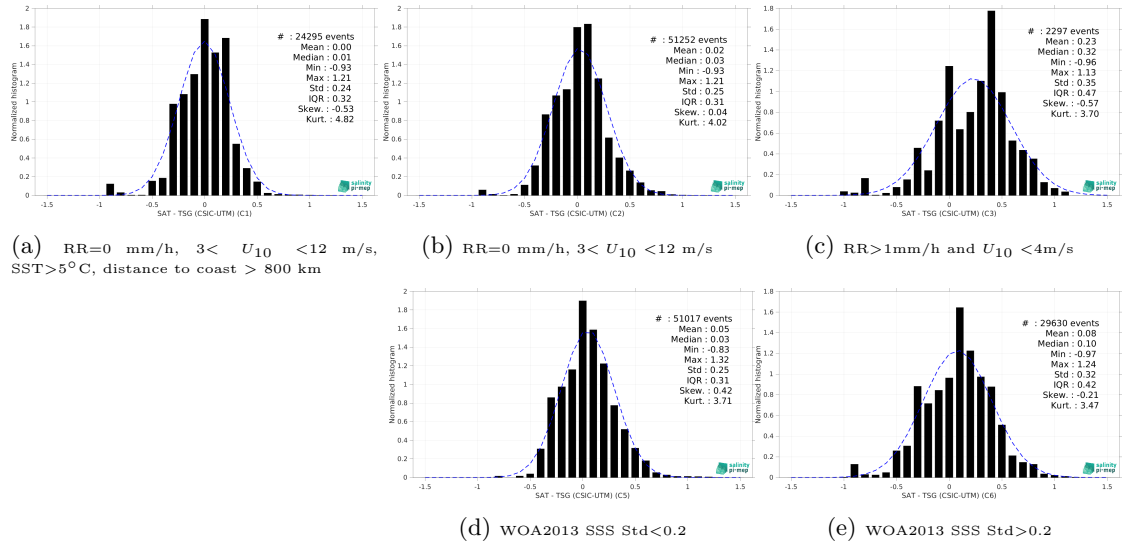
Figure 15: Normalized histogram of \Delta\text{SSS} (SMAP SSS L3 v6 - Monthly (RSS) - TSG (CSIC-UTM)) for 5 different subdatasets corresponding to: RR=0 mm/h, 3 < U_{10} < 12 m/s, SST>5°C, distance to coast > 800 km (a), RR=0 mm/h, 3 < U_{10} < 12 m/s (b), RR>1mm/h and U_{10} < 4 m/s (c), WOA2013 SSS Std<0.2 (d), WOA2013 SSS Std>0.2 (e).
