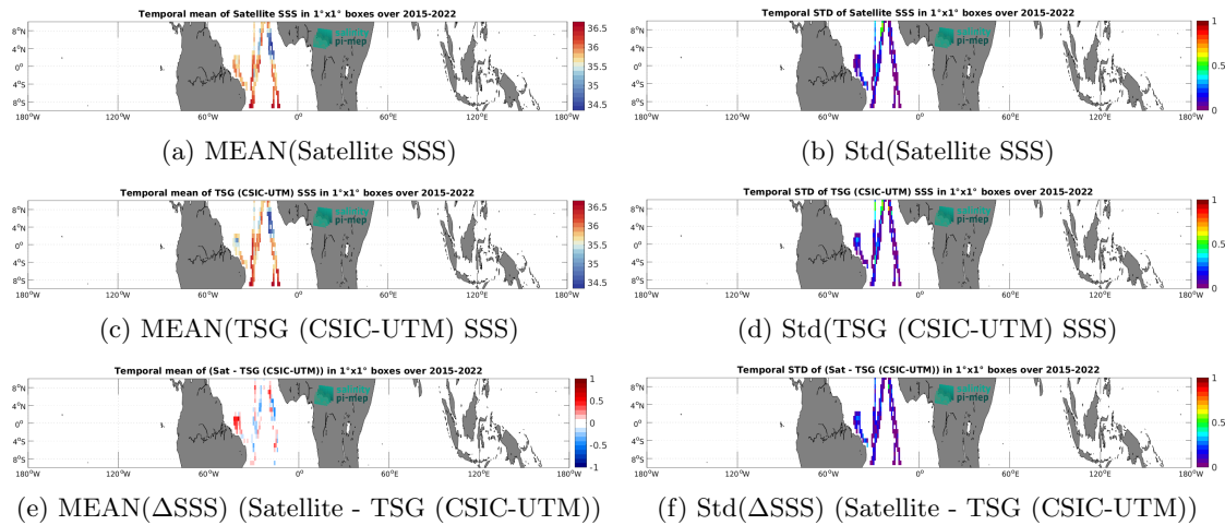
Figure 7: Temporal mean (left) and Std (right) of SSS from SMAP SSS L3 v6 - Monthly (RSS) (top), TSG (CSIC-UTM) (middle), and of \Delta SSS (Satellite - TSG (CSIC-UTM)). Only match-up pairs are used to generate these maps.
