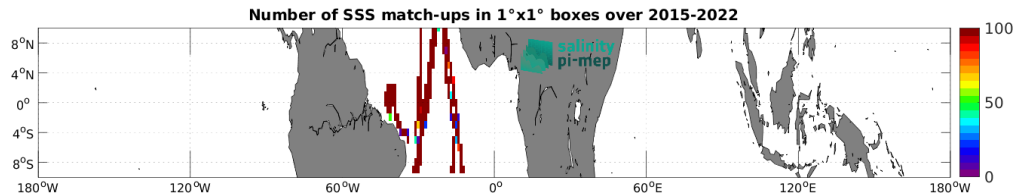
Figure 5: Number of SSS match-ups between TSG (CSIC-UTM) SSS and the SMAP SSS L3 v6 - Monthly (RSS) SSS product for the Equatorial Ocean 10N-10S Pi-MEP region over 1^\circ \times 1^\circ boxes and for the full satellite product period.
