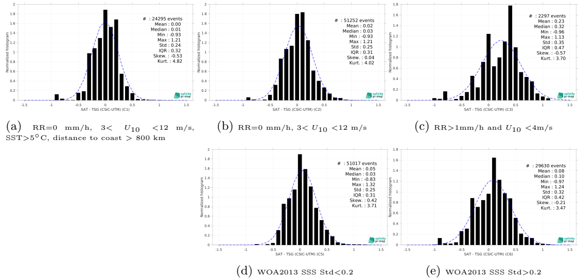
Figure 15: Normalized histogram of \Delta\text{SSS} (SMAP SSS L3 v6 - Monthly (RSS) - TSG (CSIC-UTM)) for 5 different subdatasets corresponding to: RR=0 mm/h, 3 < U_{10} < 12 m/s, SST>5°C, distance to coast > 800 km (a), RR=0 mm/h, 3 < U_{10} < 12 m/s (b), RR>1mm/h and U_{10} < 4 m/s (c), WOA2013 SSS Std<0.2 (d), WOA2013 SSS Std>0.2 (e).
