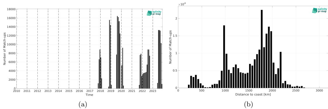
Figure 2: Number of match-ups between Saildrone and SMAP SSS L3 v6 - Monthly (RSS) SSS as a function of time (a) and as function of the distance to coast (b) over the Equatorial Ocean 10N-10S Pi-MEP region and for the full satellite product period.
