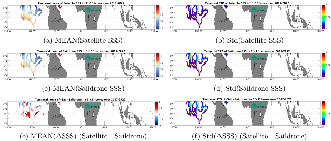
Figure 7: Temporal mean (left) and Std (right) of SSS from SMAP SSS L3 v6 - Monthly (RSS) (top), Saildrone (middle), and of \Delta SSS (Satellite - Saildrone). Only match-up pairs are used to generate these maps.
