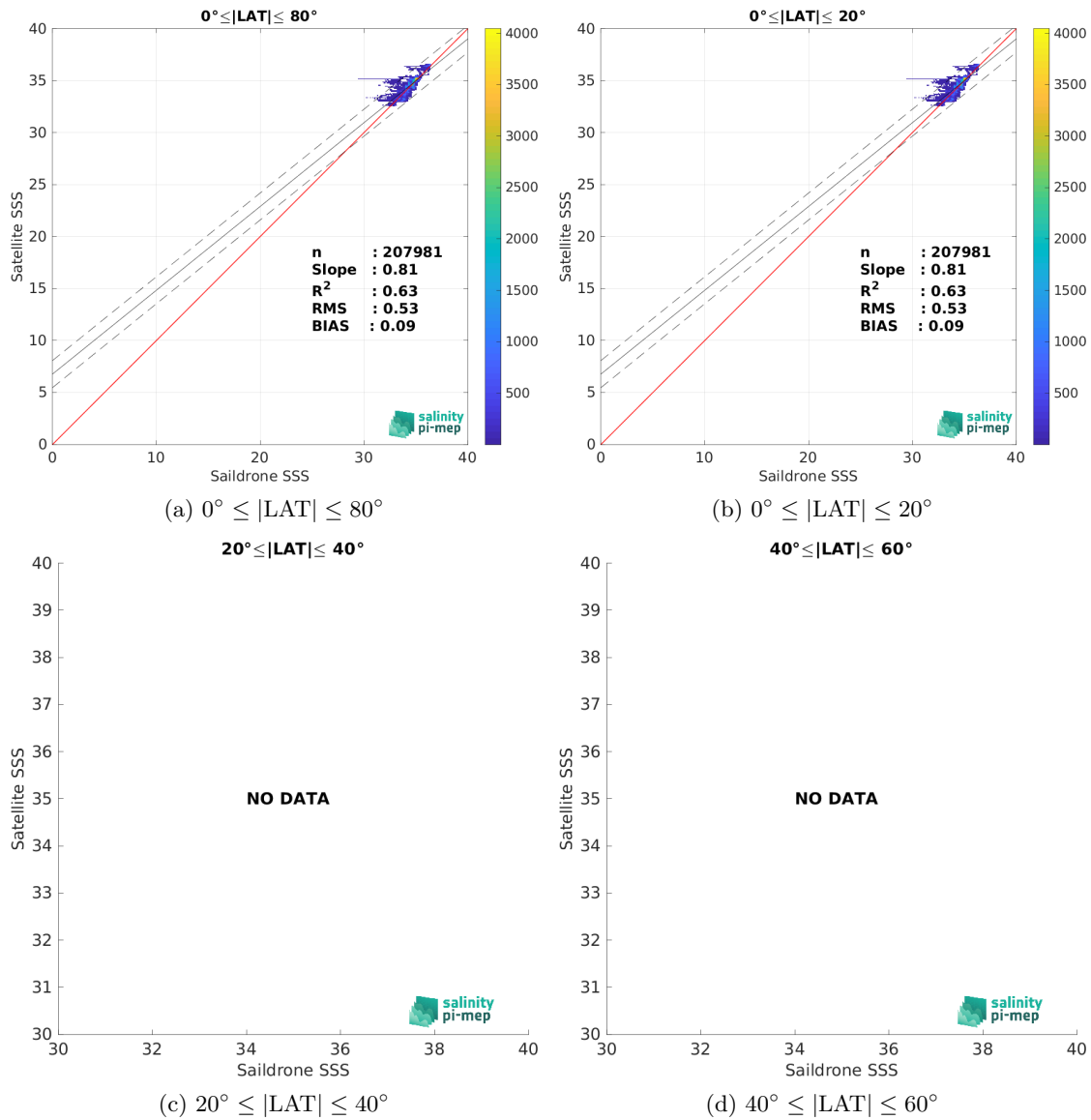
Figure 10: Contour maps of the concentration of SMAP SSS L3 v6 - Monthly (RSS) SSS (y-axis) versus Sairdrone SSS (x-axis) at match-up pairs for different latitude bands. For each plot, the red line shows x=y . The black thin and dashed lines indicate a linear fit through the data cloud and the \pm 95\% confidence levels, respectively. The number match-up pairs n , the slope and R^2 coefficient of the linear fit, the root mean square (RMS) and the mean bias between satellite and in situ data are indicated for each latitude band in each plots.
