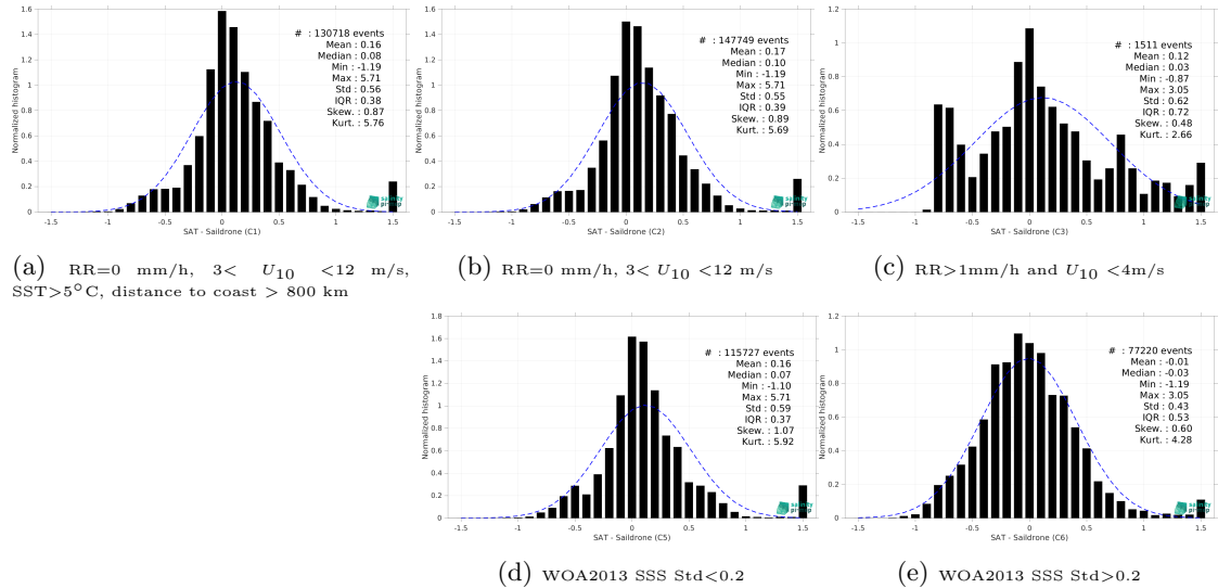
Figure 15: Normalized histogram of \Delta SSS (SMAP SSS L3 v6 - Monthly (RSS) - Saildrone) for 5 different subdatasets corresponding to: RR=0 mm/h, 3 < U_{10} < 12 m/s, SST>5°C, distance to coast > 800 km (a), RR=0 mm/h, 3 < U_{10} < 12 m/s (b), RR>1mm/h and U_{10} < 4 m/s (c), WOA2013 SSS Std<0.2 (d), WOA2013 SSS Std>0.2 (e).
