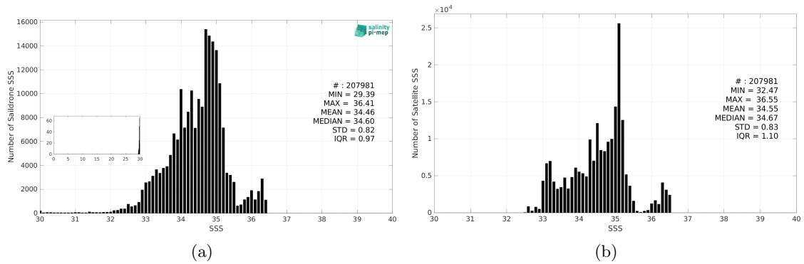
Figure 3: Histograms of SSS from Saildrone (a) and SMAP SSS L3 v6 - Monthly (RSS) (b) considering all match-up pairs per bins of 0.1 over the Equatorial Ocean 10N-10S Pi-MEP region and for the full satellite product period.
