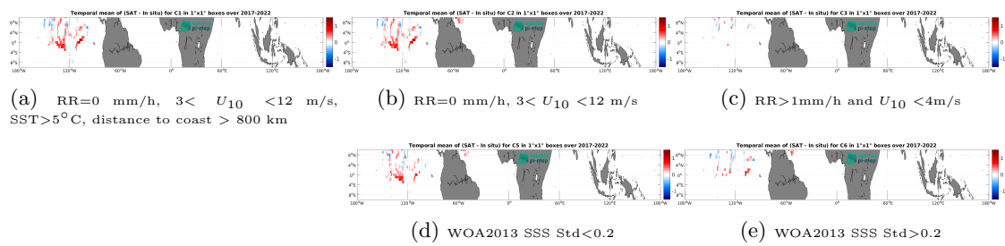
Figure 14: Temporal mean gridded over spatial boxes of size 1^\circ \times 1^\circ of \Delta SSS (SMAP SSS L3 v6 - Monthly (RSS) - Saildrone) for 5 different subdatasets corresponding to:RR=0 mm/h, 3 < U_{10} < 12 m/s, SST>5°C, distance to coast > 800 km (a), RR=0 mm/h, 3 < U_{10} < 12 m/s (b), RR>1mm/h and U_{10} < 4 m/s (c), WOA2013 SSS Std<0.2 (d), WOA2013 SSS Std>0.2 (e).
