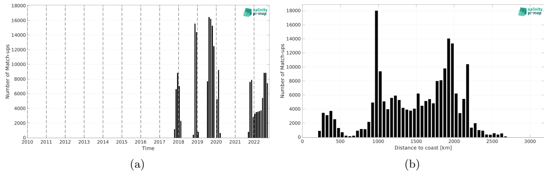
Figure 2: Number of match-ups between Saildrone and SMAP SSS L3 v6 - Monthly (RSS) SSS as a function of time (a) and as function of the distance to coast (b) over the Equatorial Ocean 10N-10S Pi-MEP region and for the full satellite product period.
