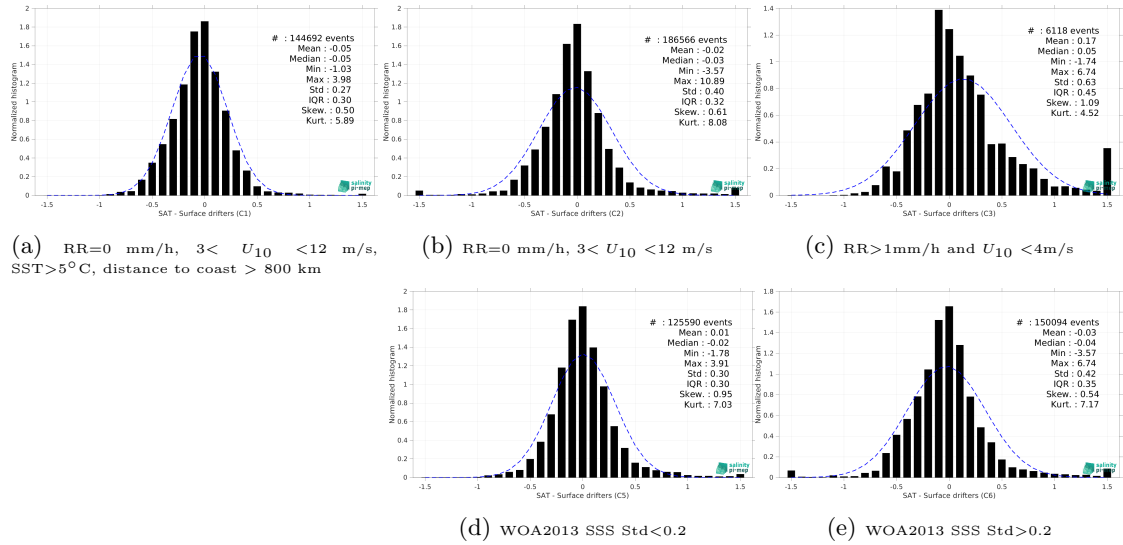
Figure 14: Normalized histogram of \Delta SSS (SMAP SSS L3 v6 - Monthly (RSS) - Surface drifters) for 5 different subdatasets corresponding to: RR=0 mm/h, 3 < U_{10} < 12 m/s, SST >5^\circ\text{C} , distance to coast > 800 km (a), RR=0 mm/h, 3 < U_{10} < 12 m/s (b), RR >1 mm/h and U_{10} < 4 m/s (c), WOA2013 SSS Std <0.2 (d), WOA2013 SSS Std >0.2 (e).
