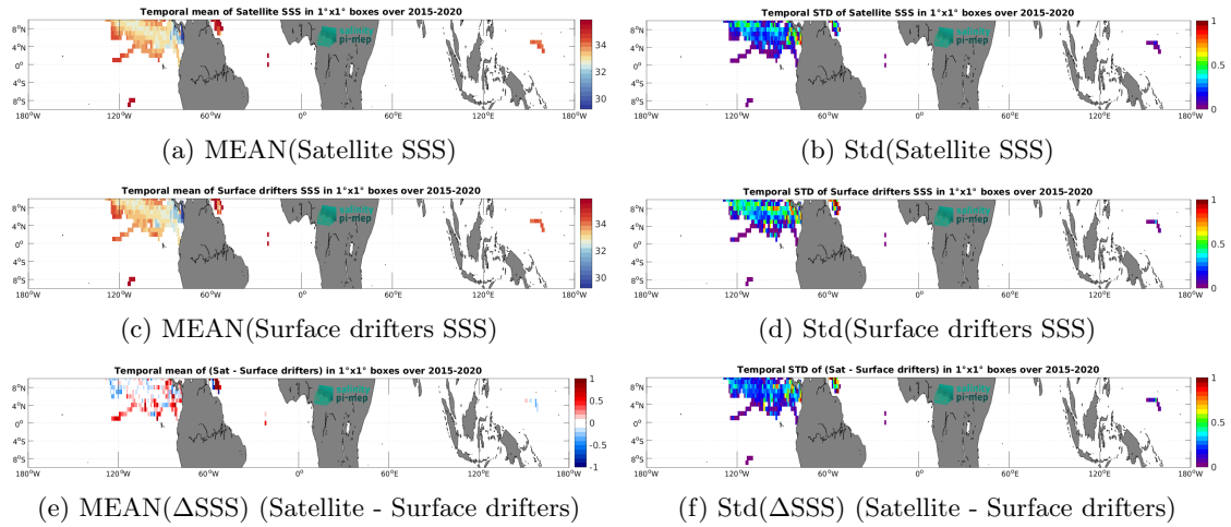
Figure 6: Temporal mean (left) and Std (right) of SSS from SMAP SSS L3 v6 - Monthly (RSS) (top), Surface drifters (middle), and of \Delta SSS (Satellite - Surface drifters). Only match-up pairs are used to generate these maps.
