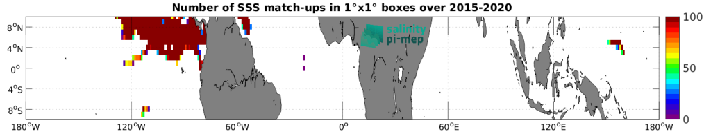
Figure 4: Number of SSS match-ups between Surface drifters SSS and the SMAP SSS L3 v6 - Monthly (RSS) SSS product for the Equatorial Ocean 10N-10S Pi-MEP region over 1^\circ \times 1^\circ boxes and for the full satellite product period.
