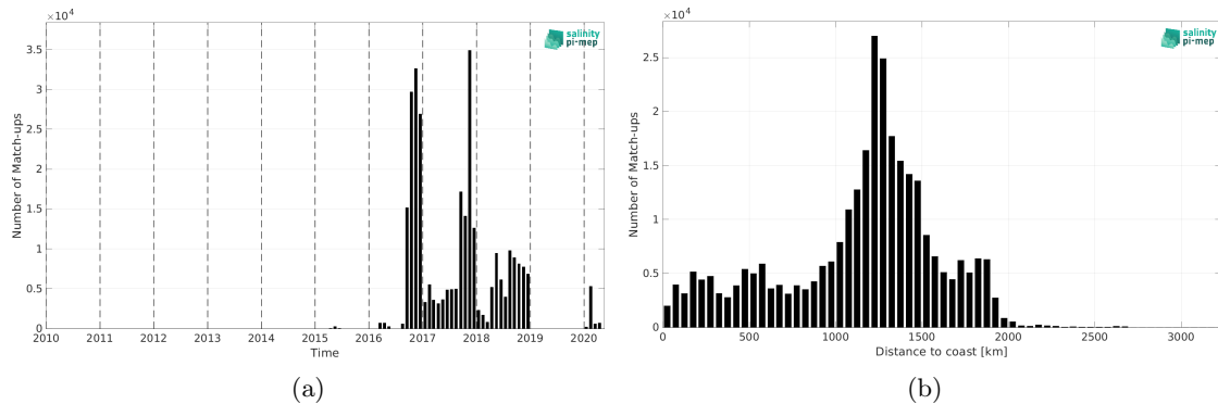
Figure 2: Number of match-ups between Surface drifters and SMAP SSS L3 v6 - Monthly (RSS) SSS as a function of time (a) and as function of the distance to coast (b) over the Equatorial Ocean 10N-10S Pi-MEP region and for the full satellite product period.
