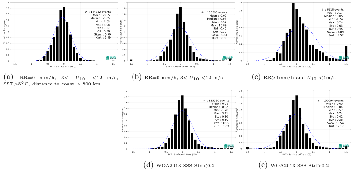
Figure 14: Normalized histogram of \Delta SSS (SMAP SSS L3 v6 - Monthly (RSS) - Surface drifters) for 5 different subdatasets corresponding to: RR=0 mm/h, 3 < U_{10} < 12 m/s, SST >5^\circ\text{C} , distance to coast > 800 km (a), RR=0 mm/h, 3 < U_{10} < 12 m/s (b), RR >1 mm/h and U_{10} < 4 m/s (c), WOA2013 SSS Std <0.2 (d), WOA2013 SSS Std >0.2 (e).
