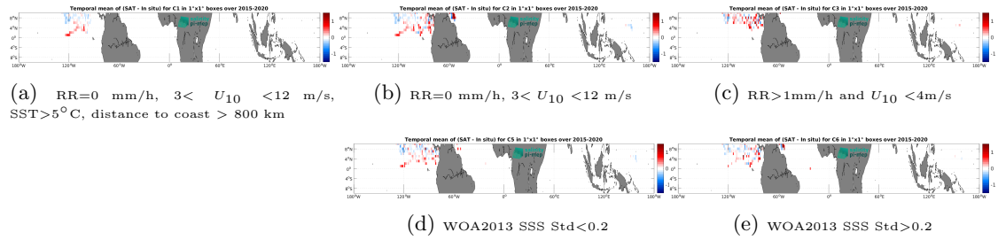
Figure 13: Temporal mean gridded over spatial boxes of size 1^\circ \times 1^\circ of \Delta SSS (SMAP SSS L3 v6 - Monthly (RSS) - Surface drifters) for 5 different subdatasets corresponding to:RR=0 mm/h, 3 < U_{10} < 12 m/s, SST >5^\circ\text{C} , distance to coast > 800 km (a), RR=0 mm/h, 3 < U_{10} < 12 m/s (b), RR >1 mm/h and U_{10} < 4 m/s (c), WOA2013 SSS Std <0.2 (d), WOA2013 SSS Std >0.2 (e).
