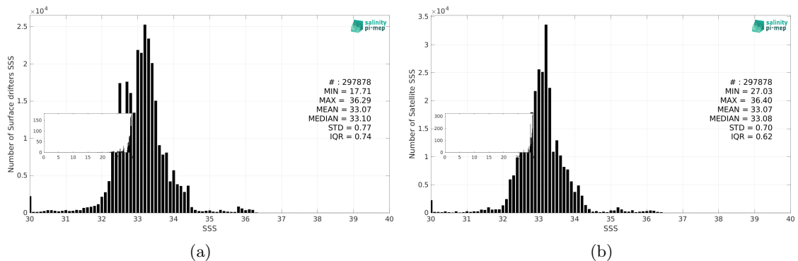
Figure 3: Histograms of SSS from Surface drifters (a) and SMAP SSS L3 v6 - Monthly (RSS) (b) considering all match-up pairs per bins of 0.1 over the Equatorial Ocean 10N-10S Pi-MEP region and for the full satellite product period.
