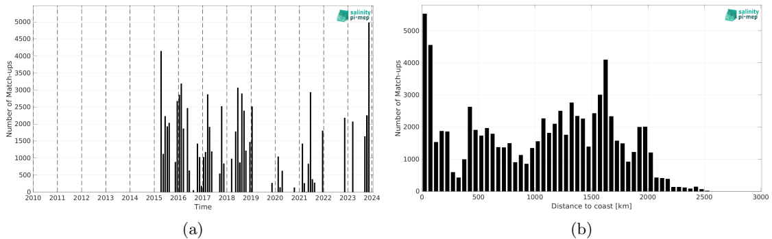
Figure 2: Number of match-ups between TSG (SAMOS) and SMAP SSS L3 v5.3 - 8-Day running (RSS) SSS as a function of time (a) and as function of the distance to coast (b) over the Equatorial Ocean 10N-10S Pi-MEP region and for the full satellite product period.
