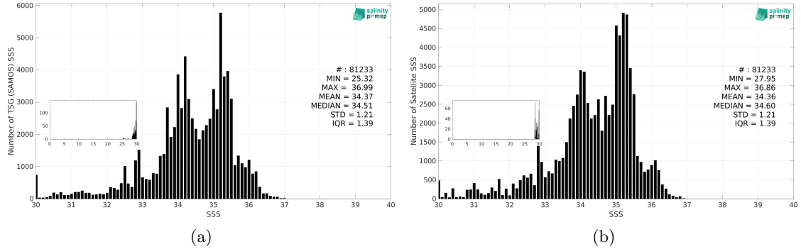
Figure 3: Histograms of SSS from TSG (SAMOS) (a) and SMAP SSS L3 v5.3 - 8-Day running (RSS) (b) considering all match-up pairs per bins of 0.1 over the Equatorial Ocean 10N-10S Pi-MEP region and for the full satellite product period.
