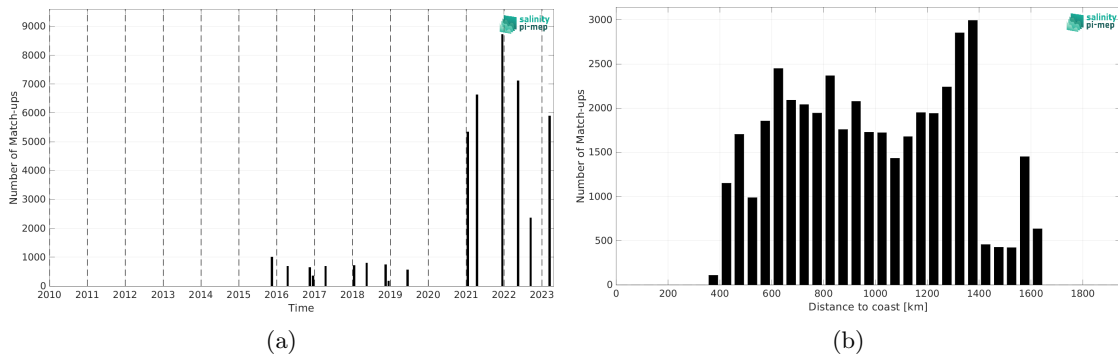
Figure 2: Number of match-ups between TSG (Polarstern) and SMAP SSS L3 v5.3 - 8-Day running (RSS) SSS as a function of time (a) and as function of the distance to coast (b) over the Equatorial Ocean 10N-10S Pi-MEP region and for the full satellite product period.
