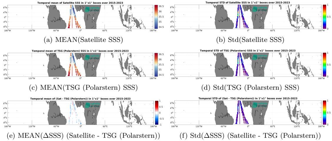
Figure 7: Temporal mean (left) and Std (right) of SSS from SMAP SSS L3 v5.3 - 8-Day running (RSS) (top), TSG (Polarstern) (middle), and of \Delta SSS (Satellite - TSG (Polarstern)). Only match-up pairs are used to generate these maps.
