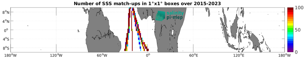
Figure 5: Number of SSS match-ups between TSG (Polarstern) SSS and the SMAP SSS L3 v5.3 - 8-Day running (RSS) SSS product for the Equatorial Ocean 10N-10S Pi-MEP region over 1^\circ \times 1^\circ boxes and for the full satellite product period.
