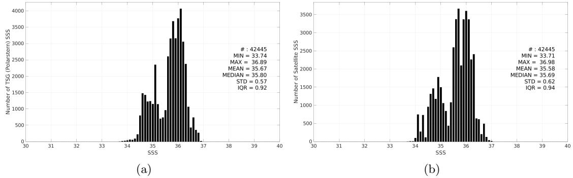
Figure 3: Histograms of SSS from TSG (Polarstern) (a) and SMAP SSS L3 v5.3 - 8-Day running (RSS) (b) considering all match-up pairs per bins of 0.1 over the Equatorial Ocean 10N-10S Pi-MEP region and for the full satellite product period.
