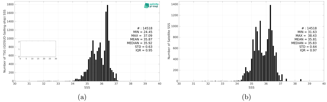
Figure 3: Histograms of SSS from TSG (GOSUD-Sailing-ship) (a) and SMAP SSS L3 v5.3 - 8-Day running (RSS) (b) considering all match-up pairs per bins of 0.1 over the Equatorial Ocean 10N-10S Pi-MEP region and for the full satellite product period.
