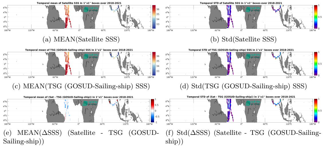
Figure 7: Temporal mean (left) and Std (right) of SSS from SMAP SSS L3 v5.3 - 8-Day running (RSS) (top), TSG (GOSUD-Sailing-ship) (middle), and of \Delta SSS (Satellite - TSG (GOSUD-Sailing-ship)). Only match-up pairs are used to generate these maps.
