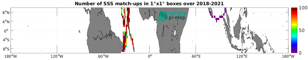
Figure 5: Number of SSS match-ups between TSG (GOSUD-Sailing-ship) SSS and the SMAP SSS L3 v5.3 - 8-Day running (RSS) SSS product for the Equatorial Ocean 10N-10S Pi-MEP region over 1^\circ \times 1^\circ boxes and for the full satellite product period.
