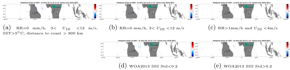
Figure 14: Temporal mean gridded over spatial boxes of size 1^\circ \times 1^\circ of \Delta\text{SSS} (SMAP SSS L3 v5.3 - 8-Day running (RSS) - TSG (GOSUD-Sailing-ship)) for 5 different subdatasets corresponding to: RR=0 mm/h, 3 < U_{10} < 12 m/s, SST>5°C, distance to coast > 800 km (a), RR=0 mm/h, 3 < U_{10} < 12 m/s (b), RR>1mm/h and U_{10} < 4 m/s (c), WOA2013 SSS Std<0.2 (d), WOA2013 SSS Std>0.2 (e).
