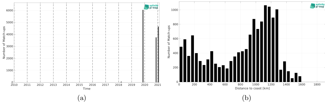
Figure 2: Number of match-ups between TSG (GOSUD-Sailing-ship) and SMAP SSS L3 v5.3 - 8-Day running (RSS) SSS as a function of time (a) and as function of the distance to coast (b) over the Equatorial Ocean 10N-10S Pi-MEP region and for the full satellite product period.
