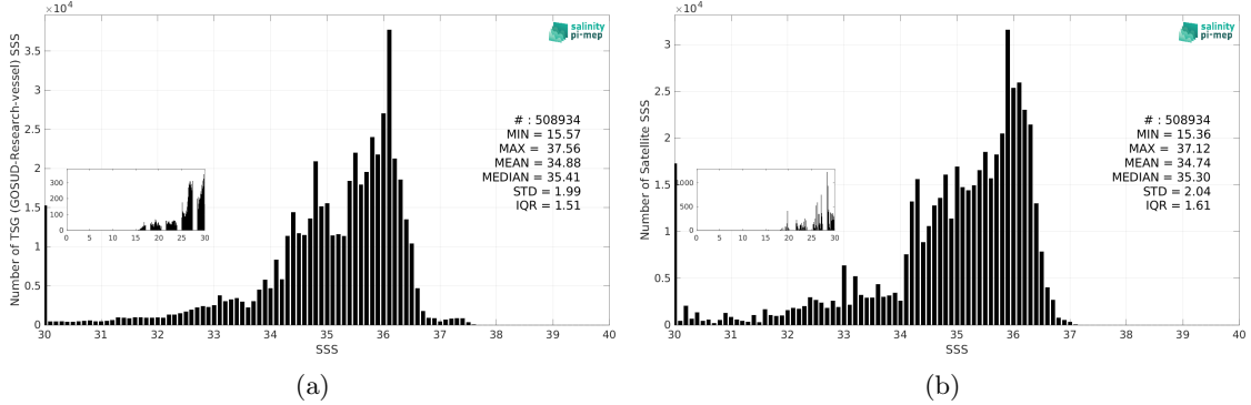
Figure 3: Histograms of SSS from TSG (GOSUD-Research-vessel) (a) and SMAP SSS L3 v5.3 - 8-Day running (RSS) (b) considering all match-up pairs per bins of 0.1 over the Equatorial Ocean 10N-10S Pi-MEP region and for the full satellite product period.
