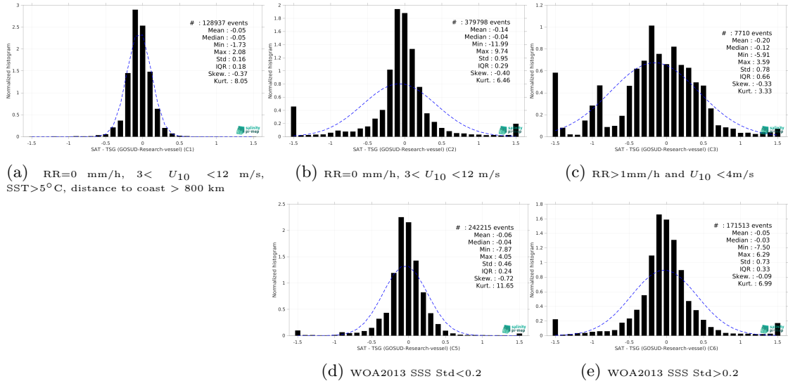
Figure 15: Normalized histogram of \Delta SSS (SMAP SSS L3 v5.3 - 8-Day running (RSS) - TSG (GOSUD-Research-vessel)) for 5 different subdatasets corresponding to: RR=0 mm/h, 3 < U_{10} < 12 m/s, SST>5°C, distance to coast > 800 km (a), RR=0 mm/h, 3 < U_{10} < 12 m/s (b), RR>1mm/h and U_{10} < 4 m/s (c), WOA2013 SSS Std<0.2 (d), WOA2013 SSS Std>0.2 (e).
