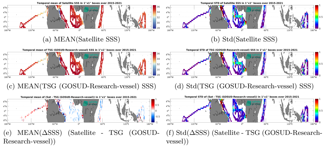
Figure 7: Temporal mean (left) and Std (right) of SSS from SMAP SSS L3 v5.3 - 8-Day running (RSS) (top), TSG (GOSUD-Research-vessel) (middle), and of \Delta SSS (Satellite - TSG (GOSUD-Research-vessel)). Only match-up pairs are used to generate these maps.
