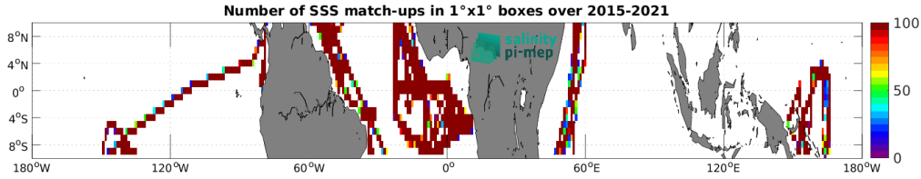
Figure 5: Number of SSS match-ups between TSG (GOSUD-Research-vessel) SSS and the SMAP SSS L3 v5.3 - 8-Day running (RSS) SSS product for the Equatorial Ocean 10N-10S Pi-MEP region over 1^\circ \times 1^\circ boxes and for the full satellite product period.
