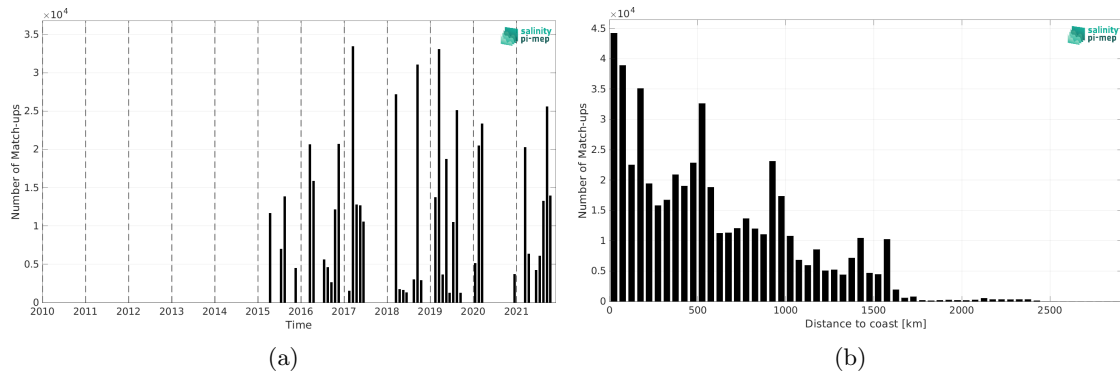
Figure 2: Number of match-ups between TSG (GOSUD-Research-vessel) and SMAP SSS L3 v5.3 - 8-Day running (RSS) SSS as a function of time (a) and as function of the distance to coast (b) over the Equatorial Ocean 10N-10S Pi-MEP region and for the full satellite product period.
