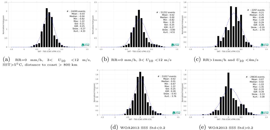
Figure 15: Normalized histogram of \Delta SSS (SMAP SSS L3 v5.3 - 8-Day running (RSS) - TSG (CSIC-UTM)) for 5 different subdatasets corresponding to: RR=0 mm/h, 3 < U_{10} < 12 m/s, SST>5°C, distance to coast > 800 km (a), RR=0 mm/h, 3 < U_{10} < 12 m/s (b), RR>1mm/h and U_{10} < 4 m/s (c), WOA2013 SSS Std<0.2 (d), WOA2013 SSS Std>0.2 (e).
