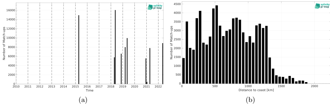
Figure 2: Number of match-ups between TSG (CSIC-UTM) and SMAP SSS L3 v5.3 - 8-Day running (RSS) SSS as a function of time (a) and as function of the distance to coast (b) over the Equatorial Ocean 10N-10S Pi-MEP region and for the full satellite product period.
