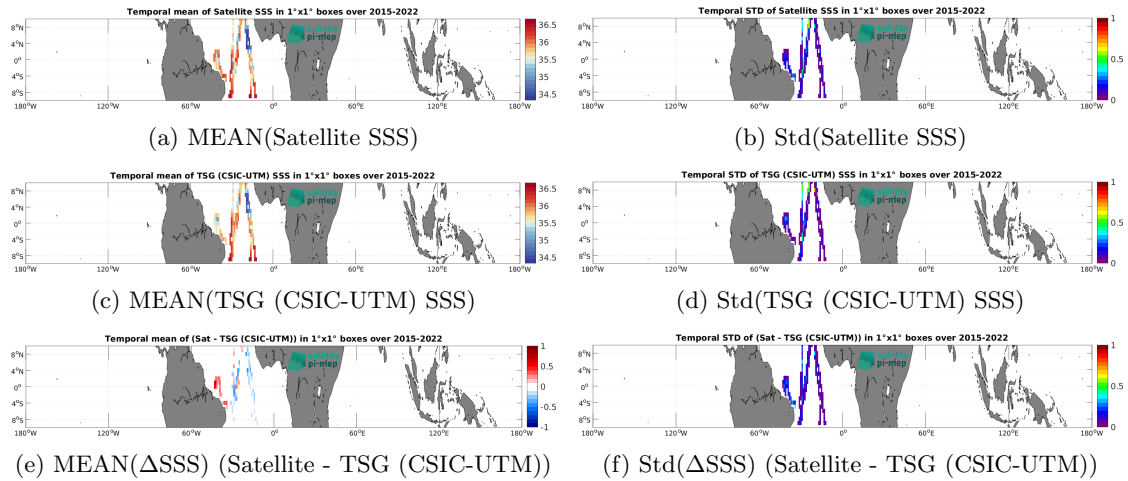
Figure 7: Temporal mean (left) and Std (right) of SSS from SMAP SSS L3 v5.3 - 8-Day running (RSS) (top), TSG (CSIC-UTM) (middle), and of \Delta SSS (Satellite - TSG (CSIC-UTM)). Only match-up pairs are used to generate these maps.
