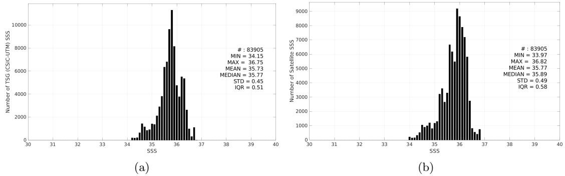
Figure 3: Histograms of SSS from TSG (CSIC-UTM) (a) and SMAP SSS L3 v5.3 - 8-Day running (RSS) (b) considering all match-up pairs per bins of 0.1 over the Equatorial Ocean 10N-10S Pi-MEP region and for the full satellite product period.
