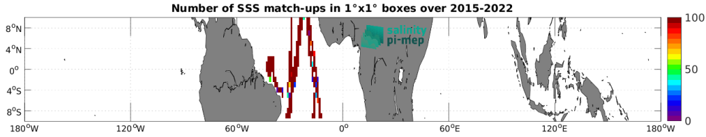
Figure 5: Number of SSS match-ups between TSG (CSIC-UTM) SSS and the SMAP SSS L3 v5.3 - 8-Day running (RSS) SSS product for the Equatorial Ocean 10N-10S Pi-MEP region over 1^\circ \times 1^\circ boxes and for the full satellite product period.
