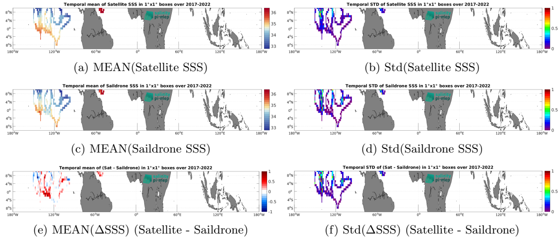
Figure 7: Temporal mean (left) and Std (right) of SSS from SMAP SSS L3 v5.3 - 8-Day running (RSS) (top), Saildrone (middle), and of \Delta SSS (Satellite - Saildrone). Only match-up pairs are used to generate these maps.
