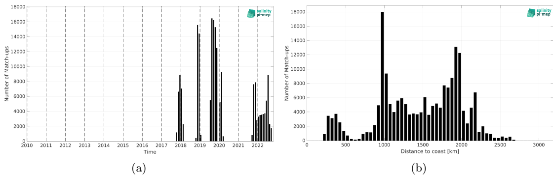
Figure 2: Number of match-ups between Saildrone and SMAP SSS L3 v5.3 - 8-Day running (RSS) SSS as a function of time (a) and as function of the distance to coast (b) over the Equatorial Ocean 10N-10S Pi-MEP region and for the full satellite product period.
