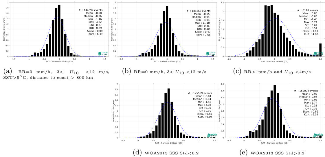
Figure 14: Normalized histogram of \Delta SSS (SMAP SSS L3 v5.3 - 8-Day running (RSS) - Surface drifters) for 5 different subdatasets corresponding to: RR=0 mm/h, 3 < U_{10} < 12 m/s, SST >5^\circ\text{C} , distance to coast > 800 km (a), RR=0 mm/h, 3 < U_{10} < 12 m/s (b), RR >1 mm/h and U_{10} < 4 m/s (c), WOA2013 SSS Std <0.2 (d), WOA2013 SSS Std >0.2 (e).
