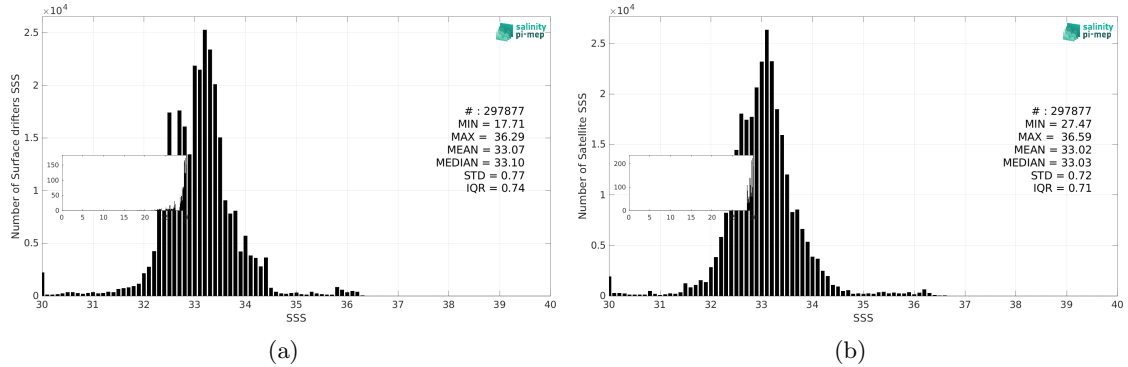
Figure 3: Histograms of SSS from Surface drifters (a) and SMAP SSS L3 v5.3 - 8-Day running (RSS) (b) considering all match-up pairs per bins of 0.1 over the Equatorial Ocean 10N-10S Pi-MEP region and for the full satellite product period.
