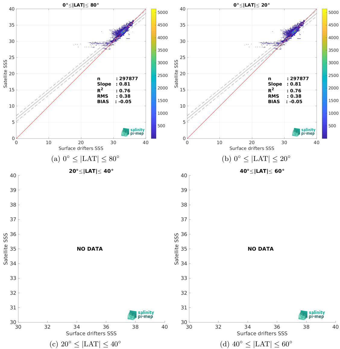
Figure 9: Contour maps of the concentration of SMAP SSS L3 v5.3 - 8-Day running (RSS) SSS (y-axis) versus Surface drifters SSS (x-axis) at match-up pairs for different latitude bands. For each plot, the red line shows x=y . The black thin and dashed lines indicate a linear fit through the data cloud and the \pm 95\% confidence levels, respectively. The number match-up pairs n , the slope and R^2 coefficient of the linear fit, the root mean square (RMS) and the mean bias between satellite and in situ data are indicated for each latitude band in each plots.
