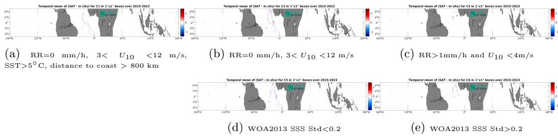
Figure 14: Temporal mean gridded over spatial boxes of size 1^\circ \times 1^\circ of \Delta SSS (SMAP SSS L3 v5.3 - Monthly (RSS) - TSG (Polarstern)) for 5 different subdatasets corresponding to:RR=0 mm/h, 3 < U_{10} < 12 m/s, SST>5°C, distance to coast > 800 km (a), RR=0 mm/h, 3 < U_{10} < 12 m/s (b), RR>1mm/h and U_{10} < 4 m/s (c), WOA2013 SSS Std<0.2 (d), WOA2013 SSS Std>0.2 (e).
