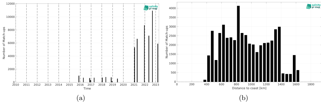
Figure 2: Number of match-ups between TSG (Polarstern) and SMAP SSS L3 v5.3 - Monthly (RSS) SSS as a function of time (a) and as function of the distance to coast (b) over the Equatorial Ocean 10N-10S Pi-MEP region and for the full satellite product period.
