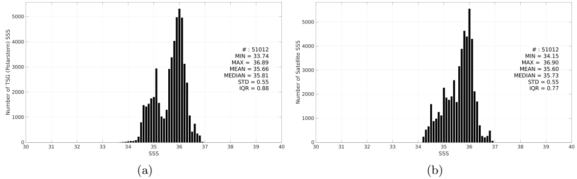
Figure 3: Histograms of SSS from TSG (Polarstern) (a) and SMAP SSS L3 v5.3 - Monthly (RSS) (b) considering all match-up pairs per bins of 0.1 over the Equatorial Ocean 10N-10S Pi-MEP region and for the full satellite product period.
