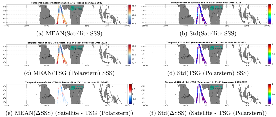
Figure 7: Temporal mean (left) and Std (right) of SSS from SMAP SSS L3 v5.3 - Monthly (RSS) (top), TSG (Polarstern) (middle), and of \Delta SSS (Satellite - TSG (Polarstern)). Only match-up pairs are used to generate these maps.
