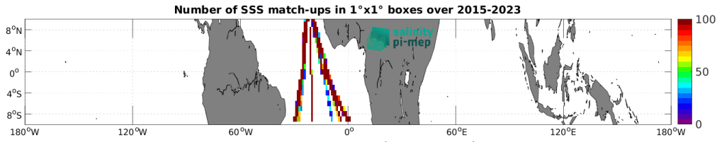
Figure 5: Number of SSS match-ups between TSG (Polarstern) SSS and the SMAP SSS L3 v5.3 - Monthly (RSS) SSS product for the Equatorial Ocean 10N-10S Pi-MEP region for 1^\circ \times 1^\circ boxes and for the full satellite product period.
