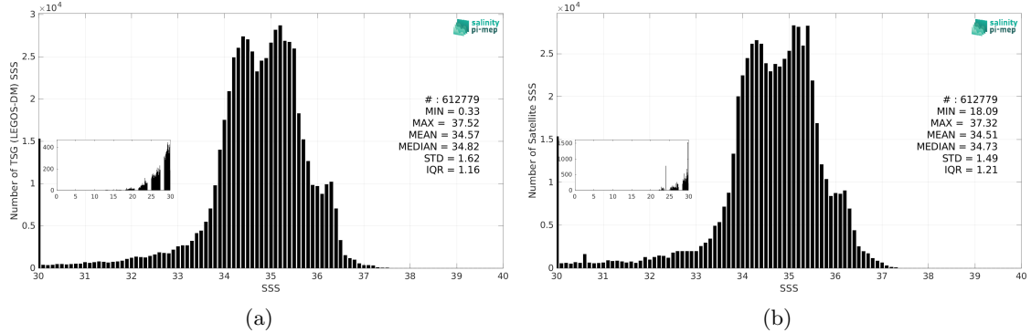
Figure 3: Histograms of SSS from TSG (LEGOS-DM) (a) and SMAP SSS L3 v5.3 - Monthly (RSS) (b) histograms all match-up pairs per bins of 0.1 over the Equatorial Ocean 10N-10S Pi-MEP region and for the full satellite product period.
