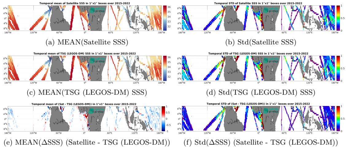
Figure 7: Temporal mean (left) and Std (right) of SSS from SMAP SSS L3 v5.3 - Monthly (RSS) (top), TSG (LEGOS-DM) (middle), and of \Delta SSS (Satellite - TSG (LEGOS-DM)). Only match-up pairs are used to generate these maps.
