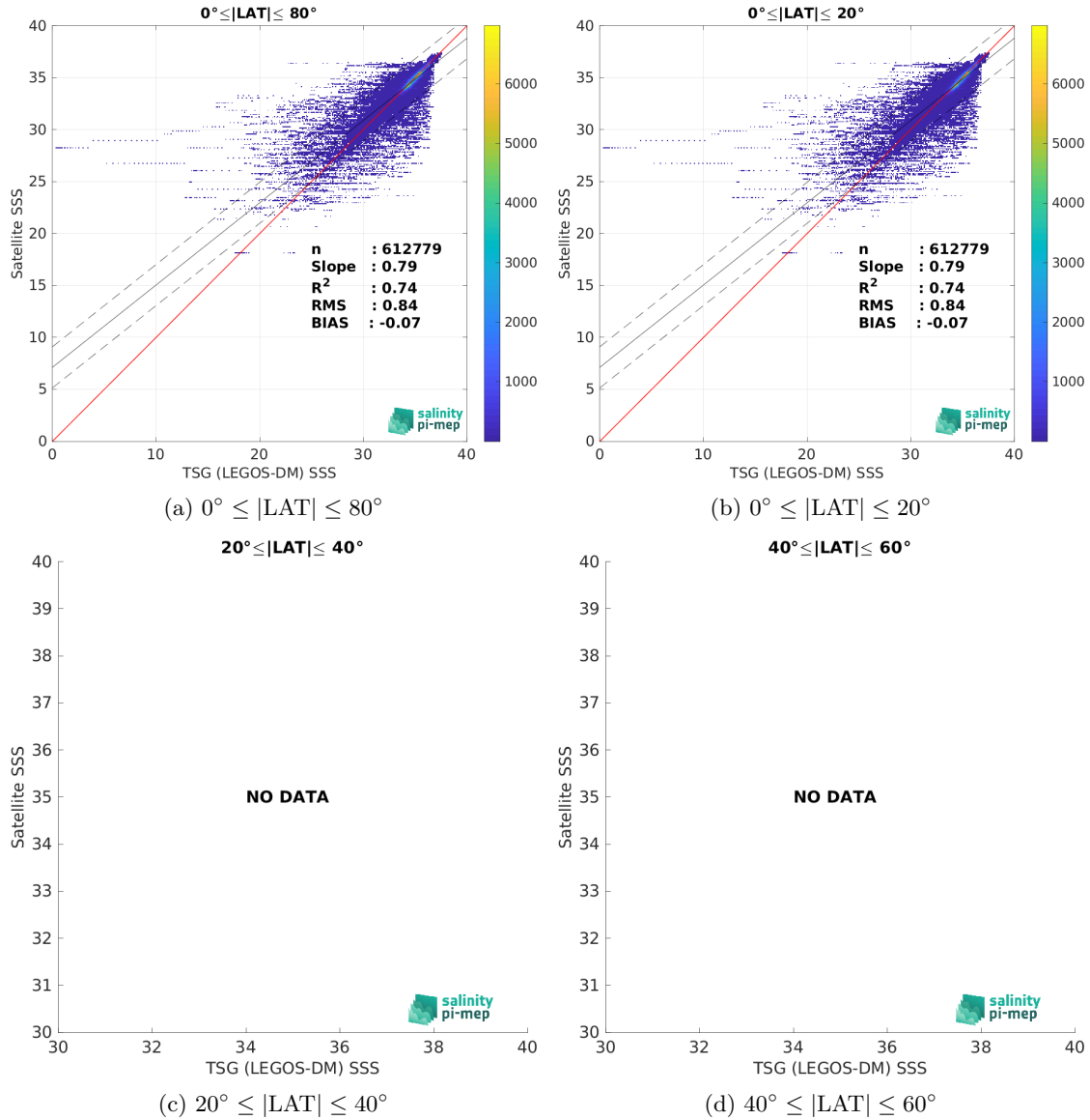
Figure 10: Contour maps of the concentration of SMAP SSS L3 v5.3 - Monthly (RSS) SSS (y-axis) versus TSG (LEGOS-DM) SSS (x-axis) at match-up pairs for different latitude bands. For each plot, the red line shows x=y . The black thin and dashed lines indicate a linear fit through the data cloud and the \pm 95\% confidence levels, respectively. The number match-up pairs n , the slope and R^2 coefficient of the linear fit, the root mean square (RMS) and the mean bias between satellite and in situ data are indicated for each latitude band in each plot.
