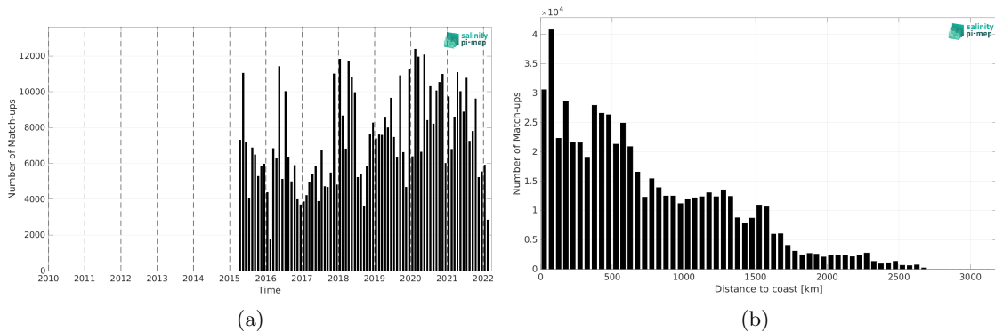
Figure 2: Number of match-ups between TSG (LEGOS-DM) and SMAP SSS L3 v5.3 - Monthly (RSS) SSS as a function of time (a) and as function of the distance to coast (b) over the Equatorial Ocean 10N-10S Pi-MEP region and for the full satellite product period.
