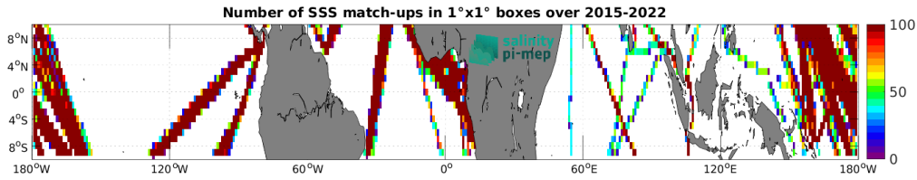
Figure 5: Number of SSS match-ups between TSG (LEGOS-DM) SSS and the SMAP SSS L3 v5.3 - Monthly (RSS) SSS product for the Equatorial Ocean 10N-10S Pi-MEP region over 1^\circ \times 1^\circ boxes and for the full satellite product period.
