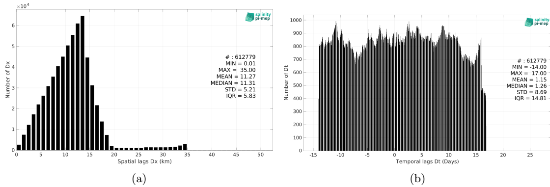
Figure 6: Histograms of the spatial (a) and temporal (b) lags between the location/time of the TSG (LEGOS-DM) measurement and the date of the corresponding SMAP SSS L3 v5.3 - Monthly (RSS) SSS pixel.
