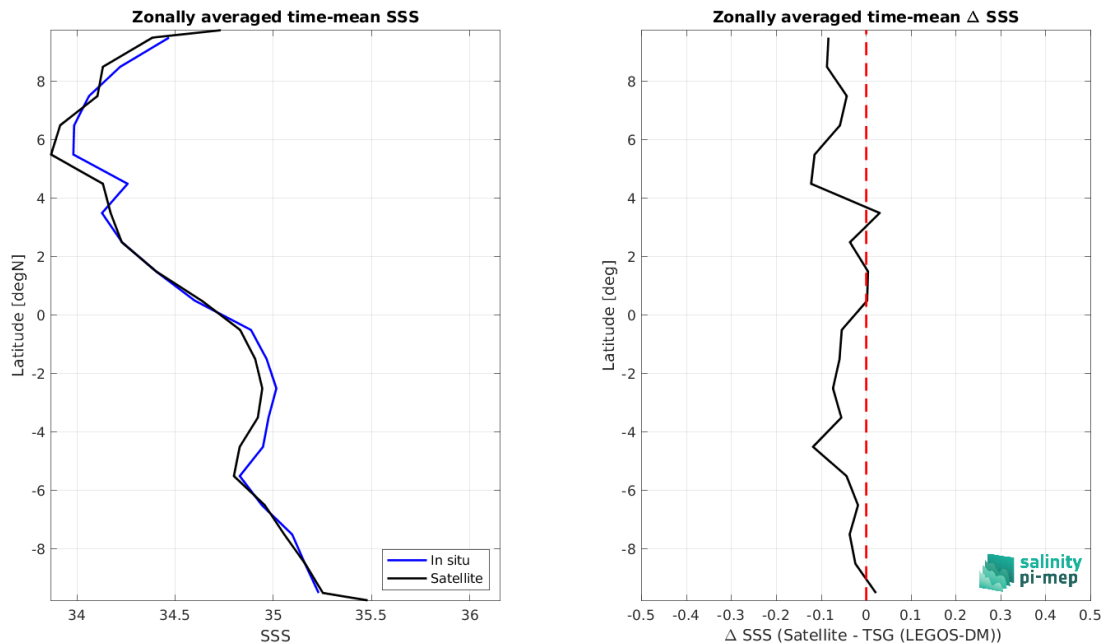
Figure 9: Left panel: Zonal mean SSS from SMAP SSS L3 v5.3 - Monthly (RSS) satellite product (black) and from TSG (LEGOS-DM) (blue). Right panel: Zonal mean of \Delta SSS (Satellite - TSG (LEGOS-DM)) for all the collected Pi-MEP match-up pairs estimated over the full satellite product period.
