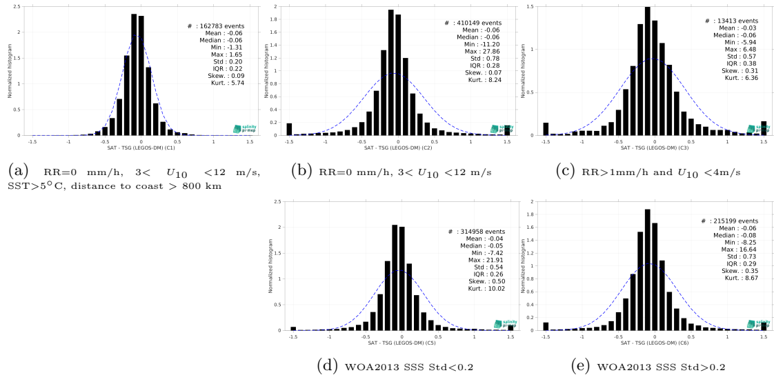
Figure 15: Normalized histogram of \Delta SSS (SMAP SSS L3 v5.3 - Monthly (RSS) - TSG (LEGOS-DM)) for 5 different subdatasets corresponding to: RR=0 mm/h, 3 < U_{10} < 12 m/s, SST>5°C, distance to coast > 800 km (a), RR=0 mm/h, 3 < U_{10} < 12 m/s (b), RR>1mm/h and U_{10} < 4 m/s (c), WOA2013 SSS Std<0.2 (d), WOA2013 SSS Std>0.2 (e).
