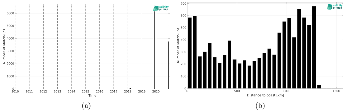
Figure 2: Number of match-ups between TSG (GOSUD-Sailing-ship) and SMAP SSS L3 v5.3 - Monthly (RSS) SSS as a function of time (a) and as function of the distance to coast (b) over the Equatorial Ocean 10N-10S Pi-MEP region and for the full satellite product period.
