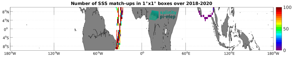
Figure 5: Number of SSS match-ups between TSG (GOSUD-Sailing-ship) SSS and the SMAP SSS L3 v5.3 - Monthly (RSS) SSS product for the Equatorial Ocean 10N-10S Pi-MEP region over 1^\circ \times 1^\circ boxes and for the full satellite product period.
