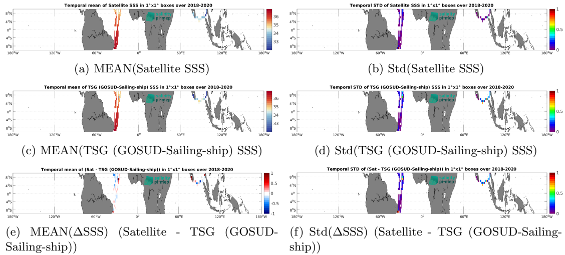
Figure 7: Temporal mean (left) and Std (right) of SSS from SMAP SSS L3 v5.3 - Monthly (RSS) (top), TSG (GOSUD-Sailing-ship) (middle), and of \Delta SSS (Satellite - TSG (GOSUD-Sailing-ship)). Only match-up pairs are used to generate these maps.
