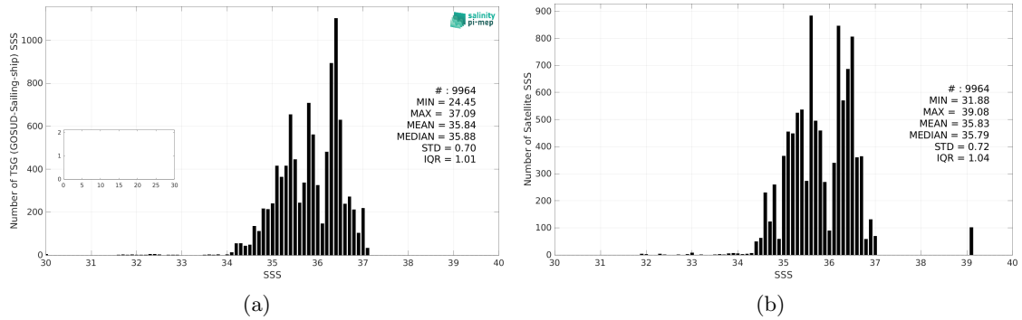
Figure 3: Histograms of SSS from TSG (GOSUD-Sailing-ship) (a) and SMAP SSS L3 v5.3 - Monthly (RSS) (b) considering all match-up pairs per bins of 0.1 over the Equatorial Ocean 10N-10S Pi-MEP region and for the full satellite product period.
