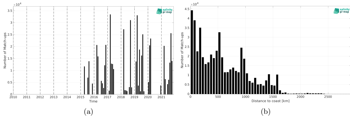
Figure 2: Number of match-ups between TSG (GOSUD-Research-vessel) and SMAP SSS L3 v5.3 - Monthly (RSS) SSS as a function of time (a) and as function of the distance to coast (b) over the Equatorial Ocean 10N-10S Pi-MEP region and for the full satellite product period.
