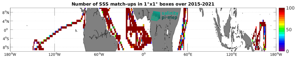
Figure 5: Number of SSS match-ups between TSG (GOSUD-Research-vessel) SSS and the SMAP SSS L3 v5.3 - Monthly (RSS) SSS product for the Equatorial Ocean 10N-10S Pi-MEP region over 1^\circ \times 1^\circ boxes and for the full satellite product period.
