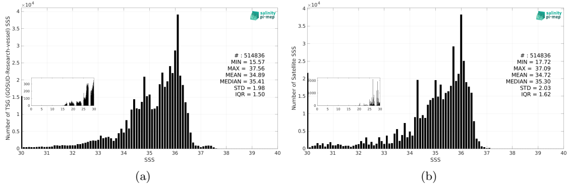
Figure 3: Histograms of SSS from TSG (GOSUD-Research-vessel) (a) and SMAP SSS L3 v5.3 - Monthly (RSS) (b) considering all match-up pairs per bins of 0.1 over the Equatorial Ocean 10N-10S Pi-MEP region and for the full satellite product period.
