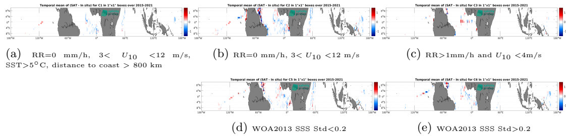
Figure 14: Temporal mean gridded over spatial boxes of size 1^\circ \times 1^\circ of \Delta SSS (SMAP SSS L3 v5.3 - Monthly (RSS) - TSG (GOSUD-Research-vessel)) for 5 different subdatasets corresponding to: RR=0 mm/h, 3 < U_{10} < 12 m/s, SST >5^\circ C, distance to coast > 800 km (a), RR=0 mm/h, 3 < U_{10} < 12 m/s (b), RR >1 mm/h and U_{10} < 4 m/s (c), WOA2013 SSS Std <0.2 (d), WOA2013 SSS Std >0.2 (e).
