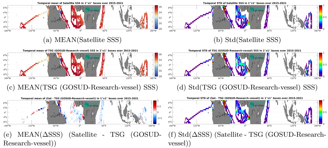
Figure 7: Temporal mean (left) and Std (right) of SSS from SMAP SSS L3 v5.3 - Monthly (RSS) (top), TSG (GOSUD-Research-vessel) (middle), and of \Delta SSS (Satellite - TSG (GOSUD-Research-vessel)). Only match-up pairs are used to generate these maps.
