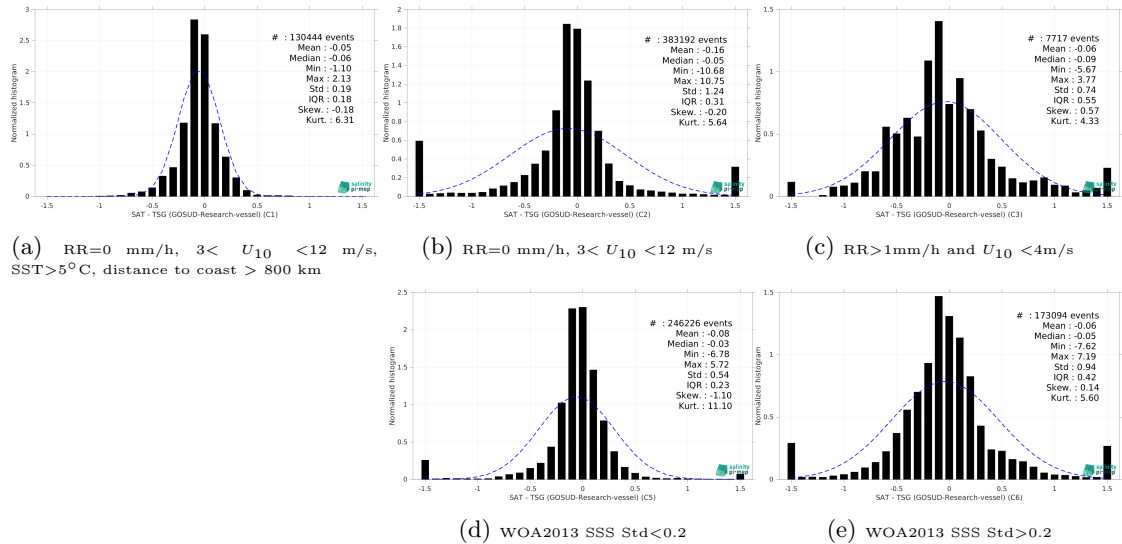
Figure 15: Normalized histogram of \Delta SSS (SMAP SSS L3 v5.3 - Monthly (RSS) - TSG (GOSUD-Research-vessel)) for 5 different subdatasets corresponding to: RR=0 mm/h, 3 < U_{10} < 12 m/s, SST >5^\circ C, distance to coast > 800 km (a), RR=0 mm/h, 3 < U_{10} < 12 m/s (b), RR >1 mm/h and U_{10} < 4 m/s (c), WOA2013 SSS Std <0.2 (d), WOA2013 SSS Std >0.2 (e).
