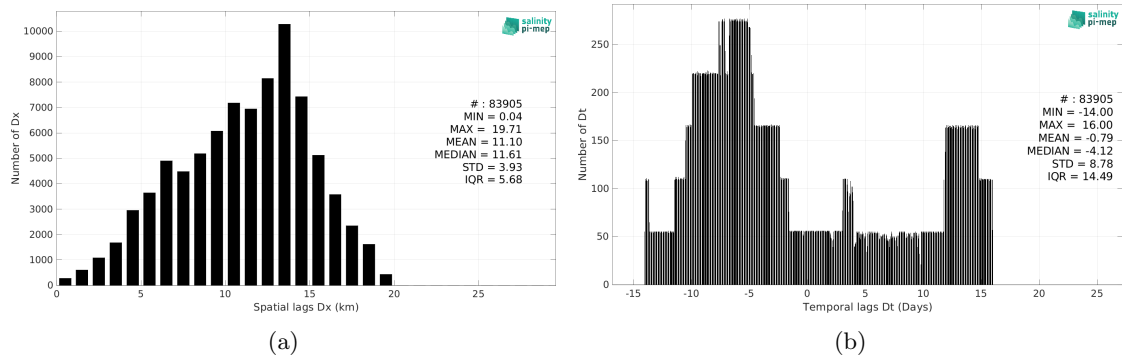
Figure 6: Histograms of the spatial (a) and temporal (b) lags between the location/time of the TSG (CSIC-UTM) measurement and the date of the corresponding SMAP SSS L3 v5.3 - Monthly (RSS) SSS pixel.
