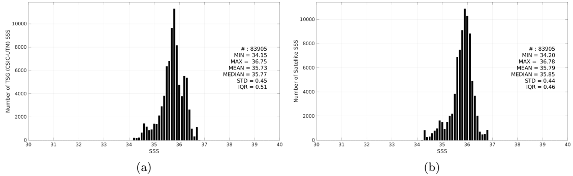
Figure 3: Histograms of SSS from TSG (CSIC-UTM) (a) and SMAP SSS L3 v5.3 - Monthly (RSS) (b) considering all match-up pairs per bins of 0.1 over the Equatorial Ocean 10N-10S Pi-MEP region and for the full satellite product period.
