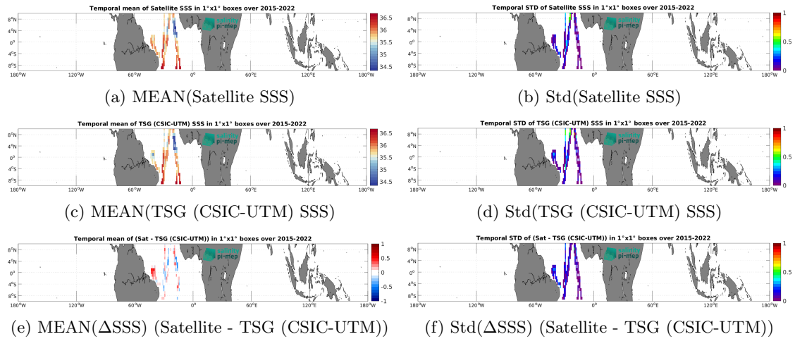
Figure 7: Temporal mean (left) and Std (right) of SSS from SMAP SSS L3 v5.3 - Monthly (RSS) (top), TSG (CSIC-UTM) (middle), and of \Delta SSS (Satellite - TSG (CSIC-UTM)). Only match-up pairs are used to generate these maps.
