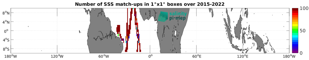
Figure 5: Number of SSS match-ups between TSG (CSIC-UTM) SSS and the SMAP SSS L3 v5.3 - Monthly (RSS) SSS product for the Equatorial Ocean 10N-10S Pi-MEP region over 1^\circ \times 1^\circ boxes and for the full satellite product period.
