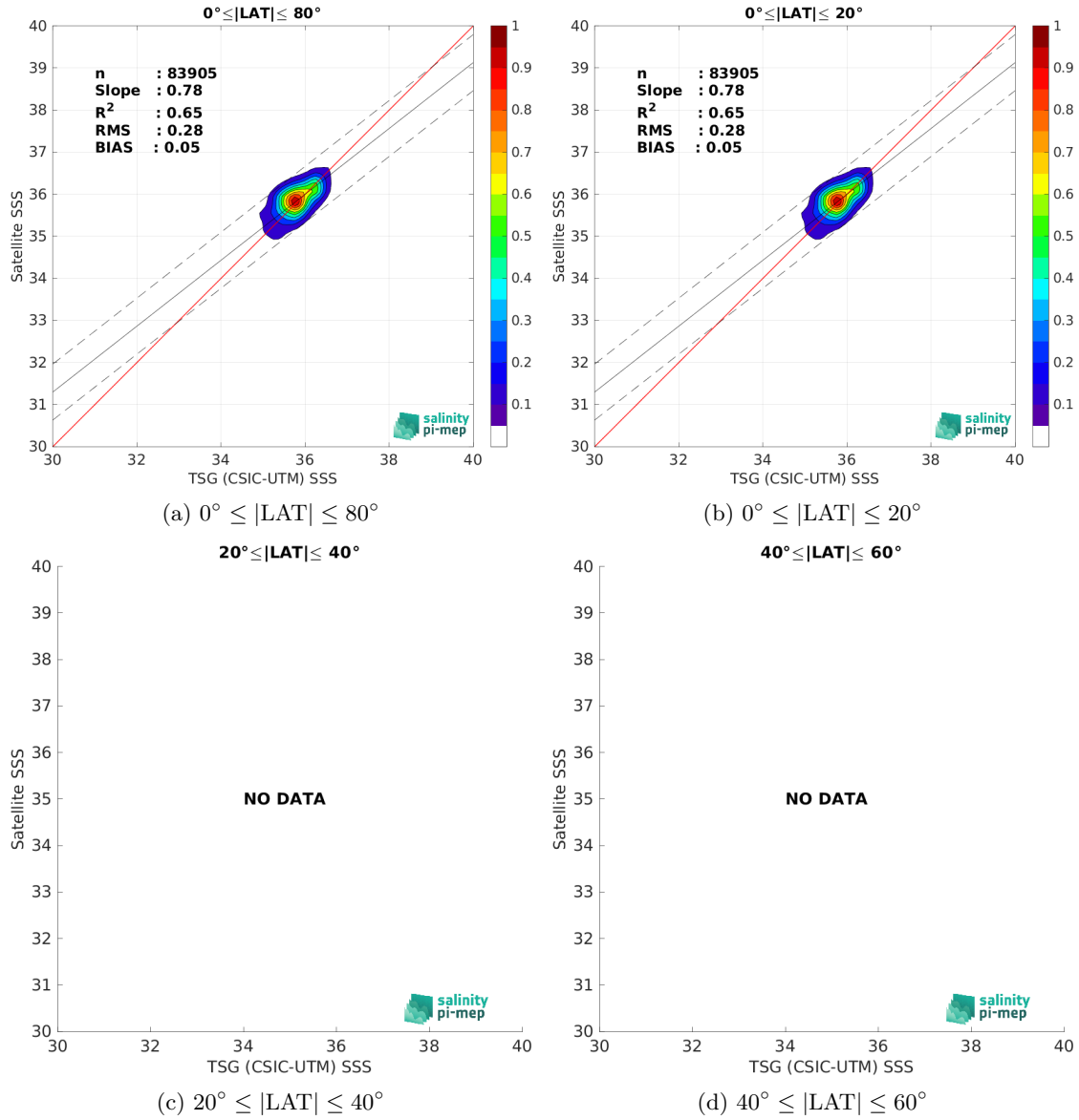
Figure 10: Contour maps of the concentration of SMAP SSS L3 v5.3 - Monthly (RSS) SSS (y-axis) versus TSG (CSIC-UTM) SSS (x-axis) at match-up pairs for different latitude bands. For each plot, the red line shows x=y . The black thin and dashed lines indicate a linear fit through the data cloud and the \pm 95\% confidence levels, respectively. The number match-up pairs n , the slope and R^2 coefficient of the linear fit, the root mean square (RMS) and the mean bias between satellite and in situ data are indicated for each latitude band in each plots.
