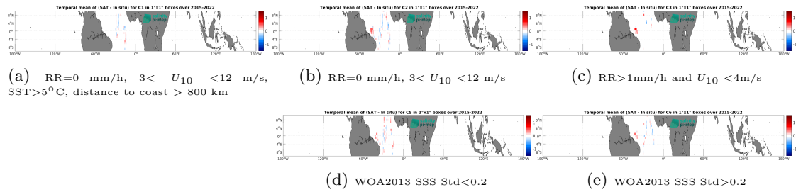
Figure 14: Temporal mean gridded over spatial boxes of size 1^\circ \times 1^\circ of \Delta SSS (SMAP SSS L3 v5.3 - Monthly (RSS) - TSG (CSIC-UTM)) for 5 different subdatasets corresponding to: RR=0 mm/h, 3 < U_{10} < 12 m/s, SST>5°C, distance to coast > 800 km (a), RR=0 mm/h, 3 < U_{10} < 12 m/s (b), RR>1mm/h and U_{10} < 4 m/s (c), WOA2013 SSS Std<0.2 (d), WOA2013 SSS Std>0.2 (e).
