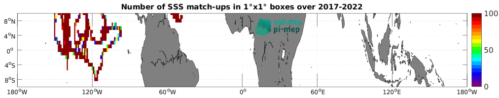
Figure 5: Number of SSS match-ups between Saildrone SSS and the SMAP SSS L3 v5.3 - Monthly (RSS) SSS product for the Equatorial Ocean 10N-10S Pi-MEP region over 1^\circ \times 1^\circ boxes and for the full satellite product period.
