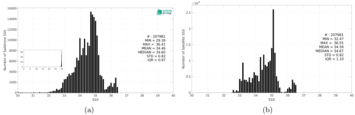
Figure 3: Histograms of SSS from Saildrone (a) and SMAP SSS L3 v5.3 - Monthly (RSS) (b) considering all match-up pairs per bins of 0.1 over the Equatorial Ocean 10N-10S Pi-MEP region and for the full satellite product period.
