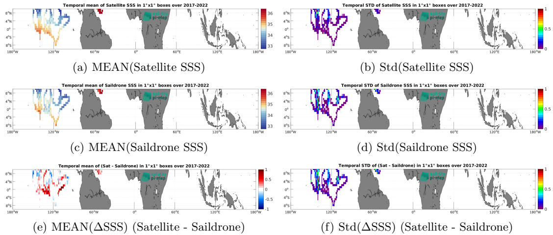
Figure 7: Temporal mean (left) and Std (right) of SSS from SMAP SSS L3 v5.3 - Monthly (RSS) (top), Saildrone (middle), and of \Delta SSS (Satellite - Saildrone). Only match-up pairs are used to generate these maps.
