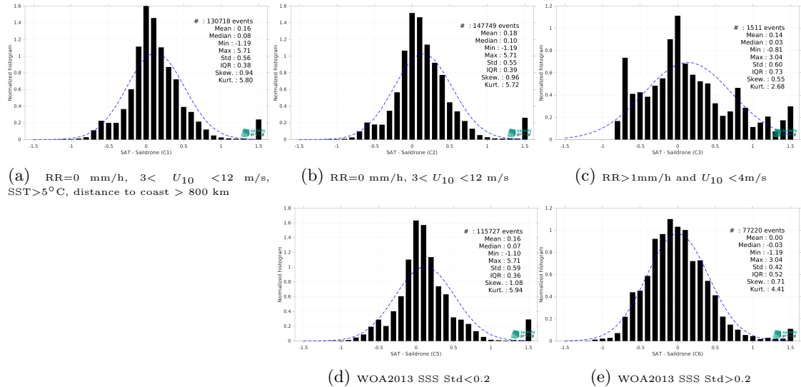
Figure 15: Normalized histogram of \Delta SSS (SMAP SSS L3 v5.3 - Monthly (RSS) - Saildrone) for 5 different subdatasets corresponding to: RR=0 mm/h, 3 < U_{10} < 12 m/s, SST>5°C, distance to coast > 800 km (a), RR=0 mm/h, 3 < U_{10} < 12 m/s (b), RR>1mm/h and U_{10} < 4 m/s (c), WOA2013 SSS Std<0.2 (d), WOA2013 SSS Std>0.2 (e).
